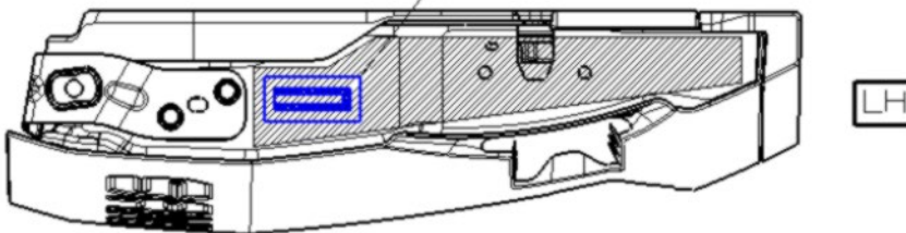
PNL ASSY-T/GATE (LH) (SCALE 3/10)
