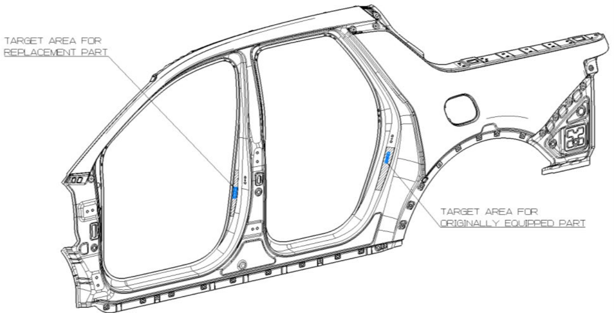
PNL-SIDE OTR, LH/RH
