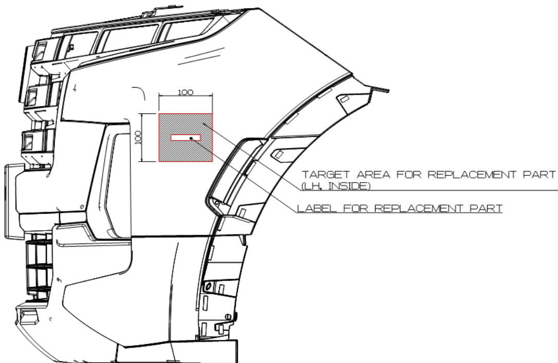
< FRONT BUMPER — SIDE VIEW >
