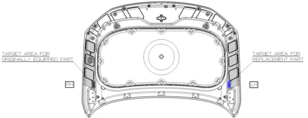
PNL ASSY-HOOD (SCALE 3/20)
