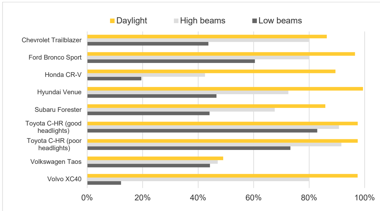
Figure 1 Average speed reductions in PAEB tests by light condition across multiple runs in each of three test scenarios performed at two speeds
