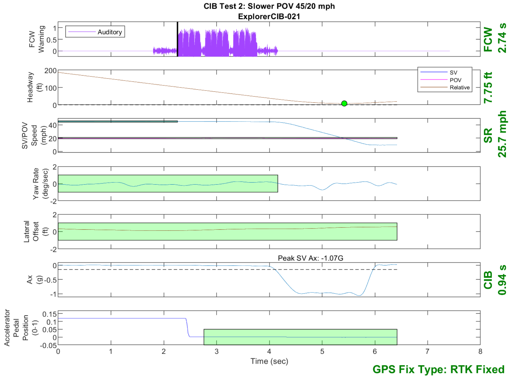
Figure D26. Time History for CIB Run 21, Test 2 - Slower Moving POV, 45/20 mph
