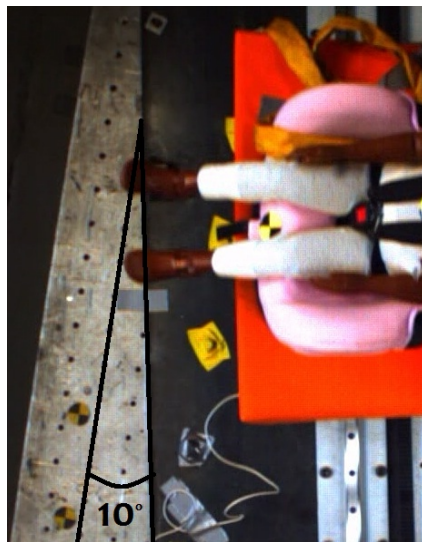
Figure 2: Depiction of the 10° secondary carriage CCW rotation angle with respect to the longitudinal axis of the primary carriage (not to scale)
