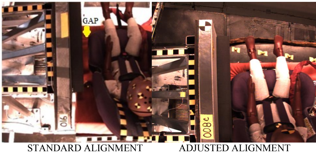
Figure 32: Overhead view of CRS-to-door interface at impact with the aluminum honeycomb
