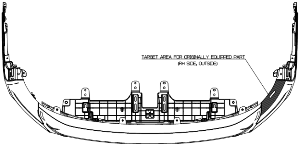
BOTTOM VIEW
