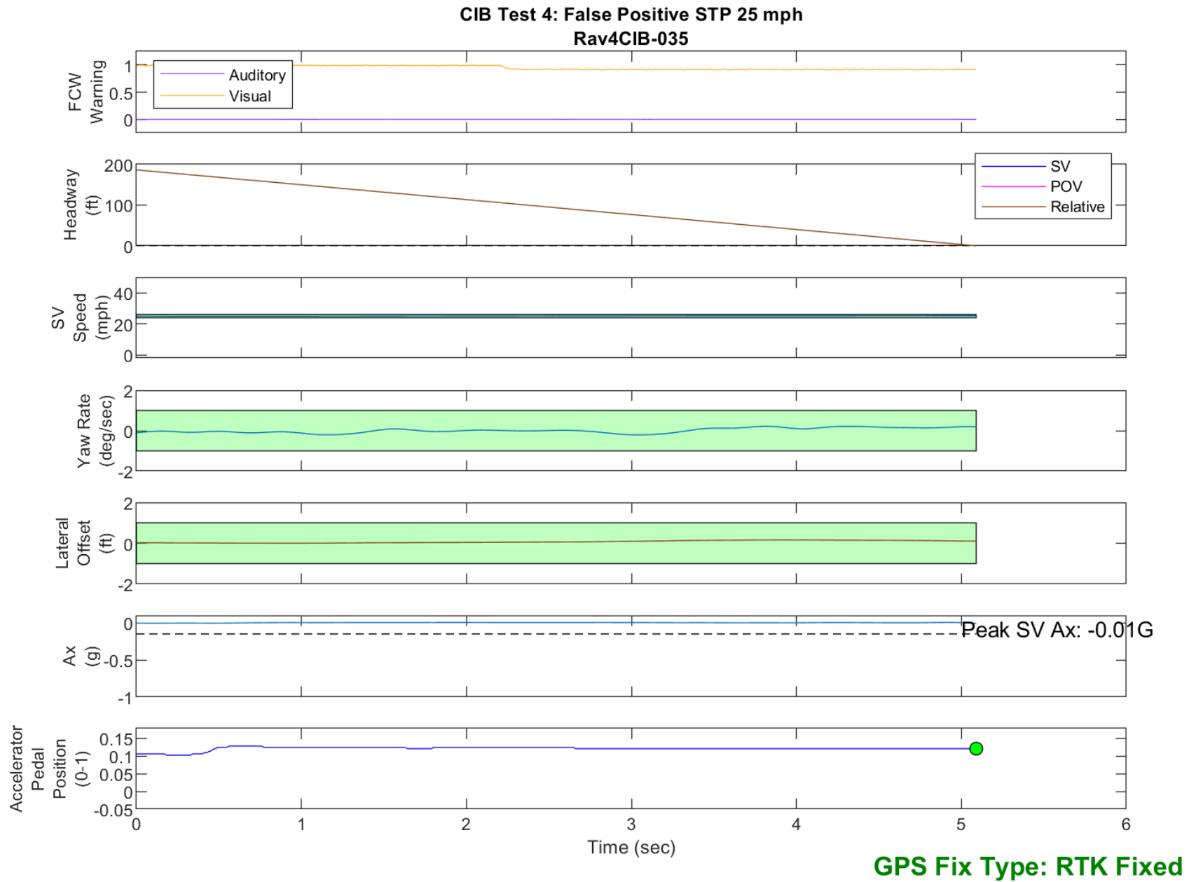
Figure D38. Time History for CIB Run 35, Test 4 - False Positive STP, 25 mph
