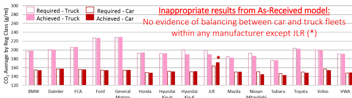
Figure 11 MY2030 Required and Achieved CO2 levels for Each manufacturers regulatory car and truck fleets in As-Received CAFE model output
