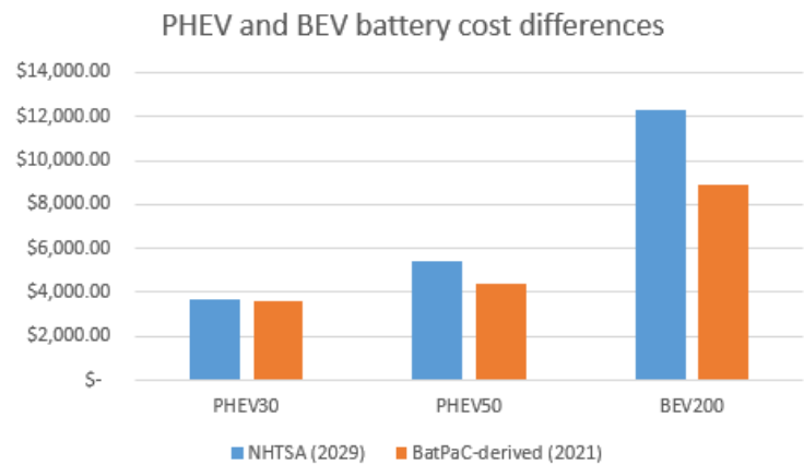
Figure 2 Comparison of PHEV and BEV battery costs
