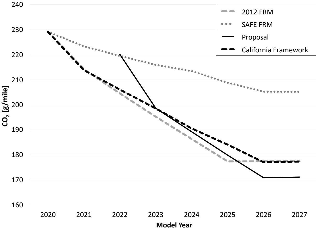
Figure 2-4: Proposed Standards Fleet Average Targets Compared to Alternatives
