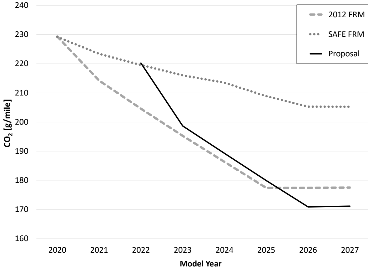
Figure 1 EPA Proposed Industry Fleet-Wide CO 2 Compliance Targets, Compared to 2012 and SAFE Rules, grams/mile, 2021-2026
