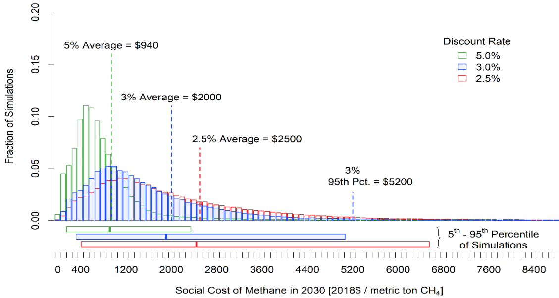
Figure 3-2: Frequency Distribution of SC-CH 4 Estimates for 2030 m
