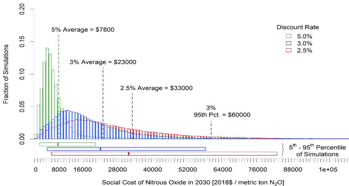
Figure 3-3: Frequency Distribution of SC-N 2 O Estimates for 2030 m
