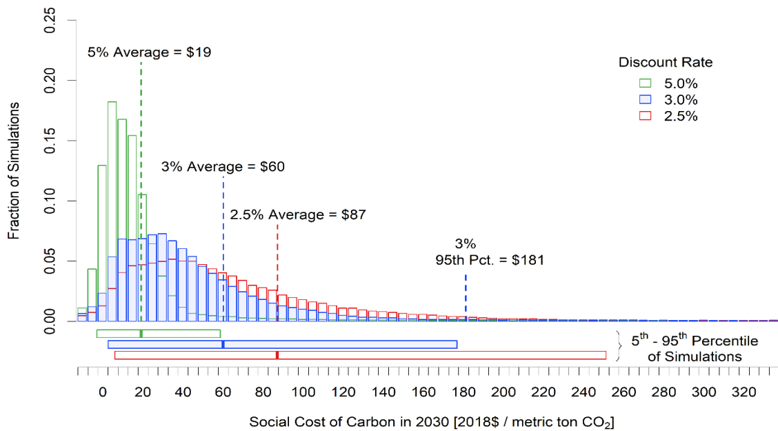
Figure 3-1: Frequency Distribution of SC-CO 2 Estimates for 2030 m
