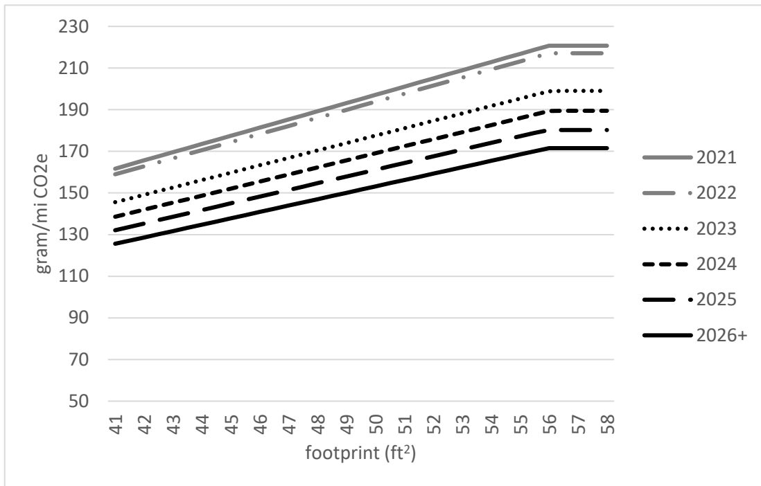
Figure 2-1: CO 2 vs Footprint Compliance Curves for Cars
