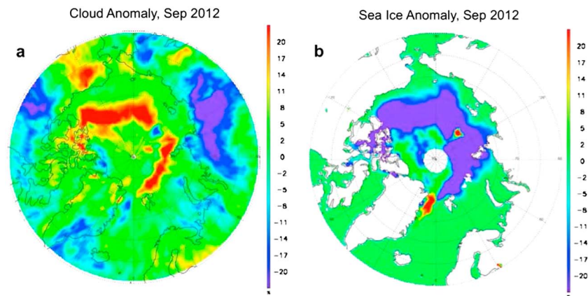
Figure 9. (a) Cloud cover and (b) sea ice concentration anomalies (in %) in September 2012 relative to the corresponding monthly means for the period 2002–2010. Data are from the Moderate Resolution Imaging Spectroradiometer on the Aqua satellite.
