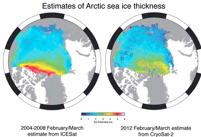
Figure 4. Sea ice thickness maps for February/March, (left) 2004–2008 average from ICESat and (right) 2012 from CryoSat-2 with location of validation data from ULS moorings (triangle, circle, and square) and airborne missions (gray and black lines). Adapted from Laxon et al. [2013].
