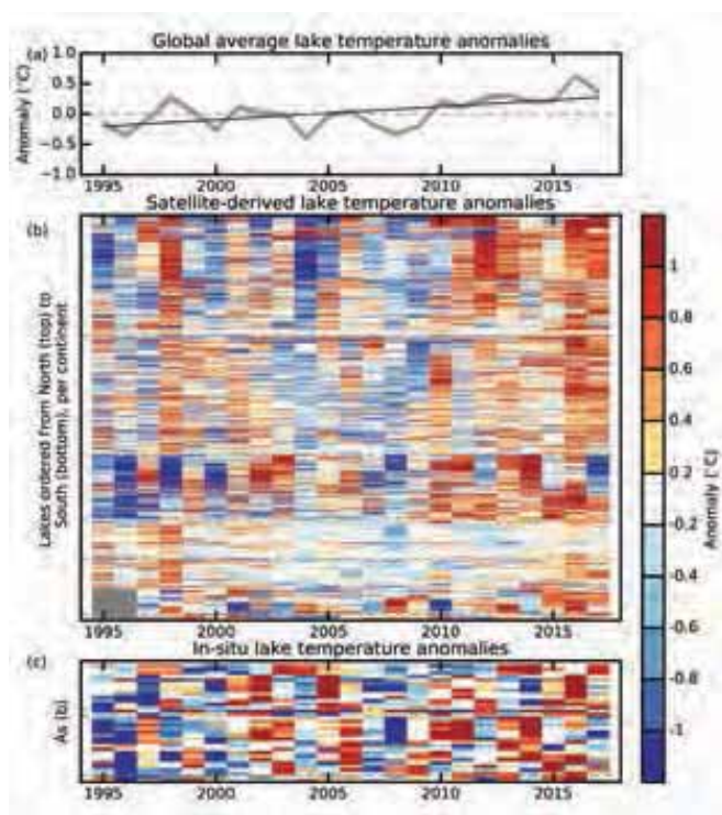
FIG. 2.3. Annual lake surface water temperature anomalies 1995–2017 (°C; relative to 1996–2015). (a) Global average (with 95% confidence intervals) satellite-derived lake surface temperature anomalies; (b) satellite-derived lake surface temperature anomalies for 688 lakes; and (c) in situ lake surface temperature anomalies for 34 globally distributed lakes. Annual lake surface water temperatures anomalies are calculated for the warm season (Jul–Sep in NH; Jan–Mar in SH), except within 23.5° of the equator, where the averages are taken over the whole year.
