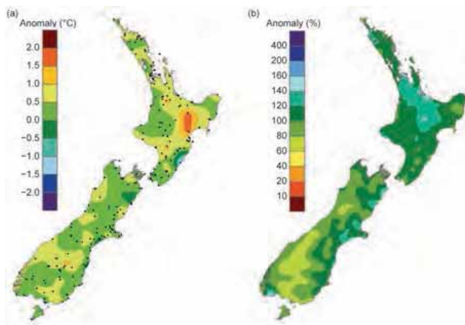
FIG. 7.56. 2017 annual (a) mean temperature anomaly (°C) and (b) total rainfall (%), relative to 1981–2010. (Source: NIWA.)
