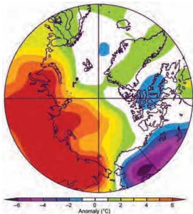
FIG. 5.3. Arctic Mar 2017 air temperature anomalies (°C).
