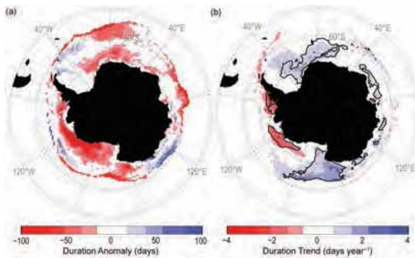
FIG. 6.9. Maps showing (a) duration anomaly for the 2016/17 sea ice season in days and (b) duration trend for 1979/80–2016/17 in days yr -1 . The black contour in (b) delineates those trends with significance at the p < 0.01 significance level.
