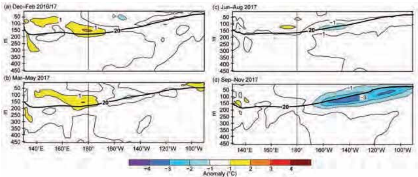
FIG. 4.3. Equatorial depth–longitude section of Pacific Ocean temperature anomalies ( ^{\circ}\text{C} ) averaged between 5^{\circ}\text{N} and 5^{\circ}\text{S} during (a) DJF 2016/17, (b) MAM 2017, (c) JJA 2017, and (d) SON 2017. The 20^{\circ}\text{C} isotherm (thick solid line) approximates the center of the oceanic thermocline. The data are derived from an analysis system that assimilates oceanic observations into an oceanic general circulation model (Behringer et al. 1998). Anomalies are departures from the 1981–2010 monthly means.
