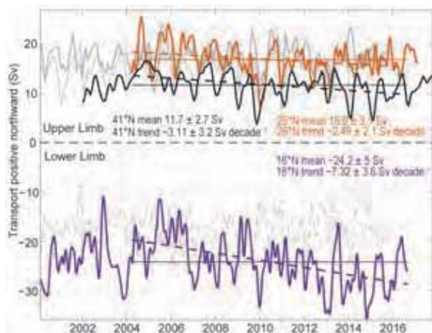
FIG. 3.23. Estimates of AMOC transports ( 1 \text{ Sv} = \times 10^6 \text{ m}^3 \text{ s}^{-1} ) from the Argo/Altimetry estimate at 41^\circ\text{N} (black; Willis 2010), the RAPID-MOC/MOCHA/WBTS 26^\circ\text{N} array (orange; Smeed et al. 2017), and the German/NOAA MOVE array at 16^\circ\text{N} (purple; Send et al. 2011) shown vs. year. All time series have a 3-month second-order Butterworth low-pass filter applied. Horizontal lines are mean transports during similar time periods as listed in the corresponding text. Dashed lines are trends for each series over the time period with data available for all three series (Apr 2004 through Aug 2016). For MOVE data, the net zonal and vertical integral of the deep circulation represents the lower limb of the AMOC (with a negative sign indicating southward flow), and hence a stronger negative (southward) flow represents an increase in the AMOC amplitude. Light gray lines show ECCO2-derived transports (Menemenlis et al. 2008): (top) thin gray is the 41^\circ\text{N} transport, thick gray is the 26^\circ\text{N} transport, (bottom) the negative meridional overturning circulation in the model shown for ease of comparison with the 16^\circ\text{N} data.
