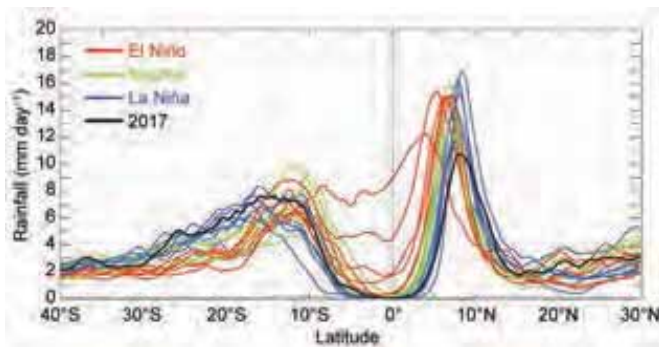
FIG. 4.12. CMORPH rainfall rate ( \text{mm day}^{-1} ) for Oct–Dec, for each year 1998 to 2017, averaged over the longitude sector 180^{\circ} – 150^{\circ} W. The cross-sections are color-coded according to NOAA's ONI, except for 2017 (a La Niña period) shown in black.
