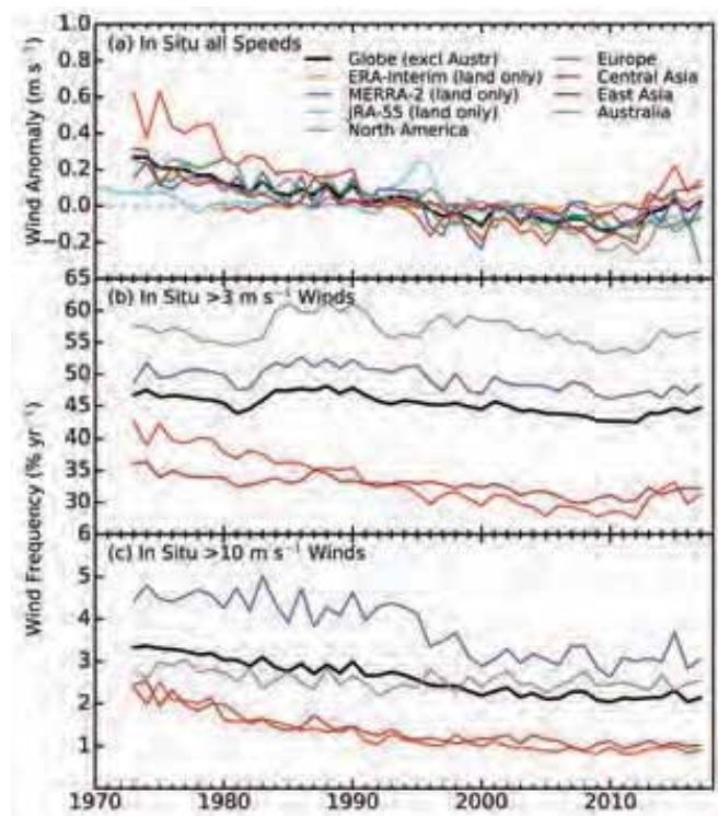
FIG. 2.38. Global (excluding Australia) and regional annual time series of land surface wind speed anomaly ( \text{m s}^{-1} ; relative to 1981–2010) using HadISD2 (1973–2017), an Australian dataset, and ERA-Interim (1979–2017), MERRA-2 (1980–2017) and JRA-55 (1970–2017). Occurrence frequencies (in %) for wind speeds (b) > 3 \text{ m s}^{-1} and (c) > 10 \text{ m s}^{-1} do not include Australia.
