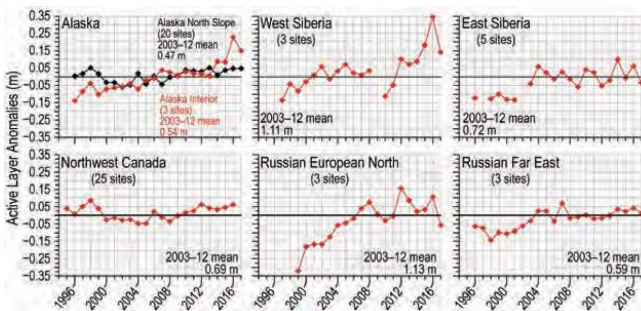
FIG. 5.20. Long-term annual active-layer thickness change (m) in six different Arctic regions for 2017 as observed by the CALM program relative to the 2003–12 mean. Positive (negative) anomaly values indicate the active layer was thicker (thinner) than average. Thaw depth observations from the end of the thawing season were used. Only sites with at least 20 years of continuous thaw depth observations are shown.
