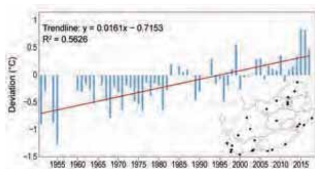
FIG. 7.27. Annual mean temperature anomalies (°C; 1981–2010 base period) of 26 climate stations in South Africa, as indicated on inset map, for 1951–2017. Red line represents the linear trend. (Source: South African Weather Service.)
