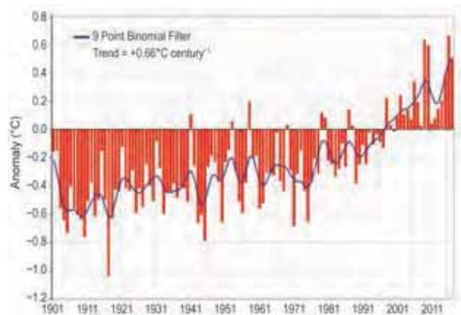
FIG. 7.46. Annual mean temperature anomalies ( ^{\circ}\text{C} ; 1981–2010 base period) averaged over India for 1901–2017. The smoothed time series (9-point binomial filter) is shown as a continuous blue line.
