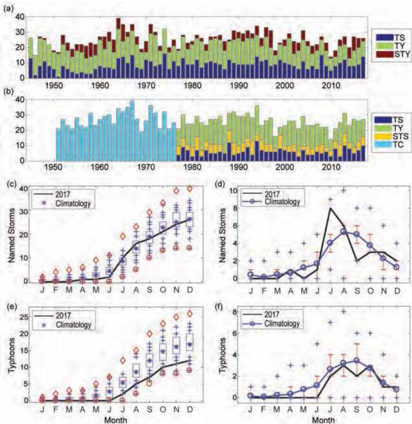
FIG. 4.28. (a) Number of tropical storms (TS), typhoons (TY), and supertyphoons (STY) per year in the western North Pacific (WNP) for the period 1945–2017 based on the JTWC best-track dataset. (b) Number of tropical cyclones (TC; all storms which reach TS intensity or higher) from 1951 to 1976; number of TSs, severe tropical storms (STS) and TY from 1977 to 2017 based on the JMA best-track dataset. Panels (c) and (e) show the cumulative number of tropical cyclones with TS intensity or higher (named storms) and number of TYs, per month in the WNP in 2017 (black line), and climatology (1981–2010) as box plots [interquartile range: box; median: red line; mean: blue asterisk; values in the top or bottom quartile: blue crosses; high (low) records in the 1945–2016 period: red diamonds (circles)]. Panels (d) and (f) show the number of NSs and TYs respectively, per month in 2017 (black line) and the climatological mean (blue line), the blue plus signs denote the maximum and minimum monthly historical records and the red error bars show the climatological interquartile range for each month (in the case of no error bars, the upper and/or lower percentiles coincide with the median). [Sources: 1945–2017 JTWC best-track dataset, 2017 JTWC preliminary operational track data for panels (a) and (c)–(f). 1951–2017 RSMCenter-Tokyo, JMA best-track dataset for panel (b).]
