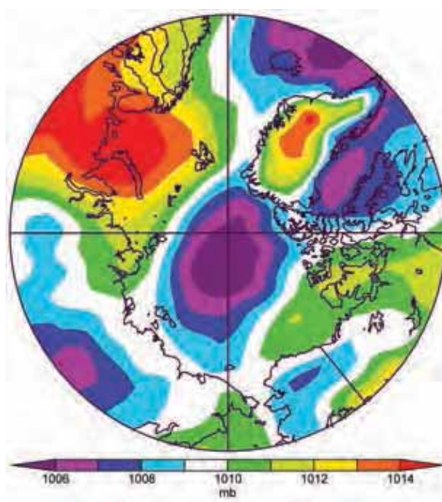
FIG. 5.4. Arctic mean sea level pressure field (hPa) for summer 2017.
