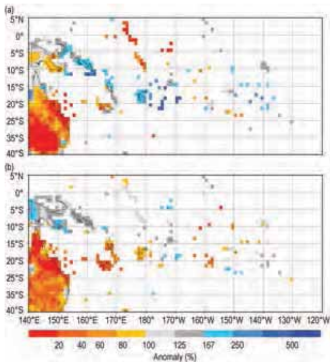
FIG. 7.52. Precipitation anomalies (% of normal wrt 1951–2000): (a) Feb 2017, (b) Jun–Aug 2017. (Source: GPCC Monitoring Product version 5.)
