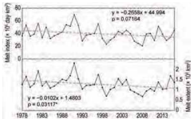
FIG. 6.7. (a) Melt index ( \times 10^6 day \cdot km ^2 ) from 1978/79 to 2016/17, showing a negative trend (265 800 day \cdot km ^2 yr ^{-1} , not significant at 95%). (b) Melt extent ( \times 10^6 km ^2 ) from 1978/79 to 2016/17, showing a negative trend (10200 km ^2 yr ^{-1} , p < 0.05\% ). The year on the x-axis corresponds to the start of the austral summer melt season, that is, 2008 corresponds to summer 2008/09.
