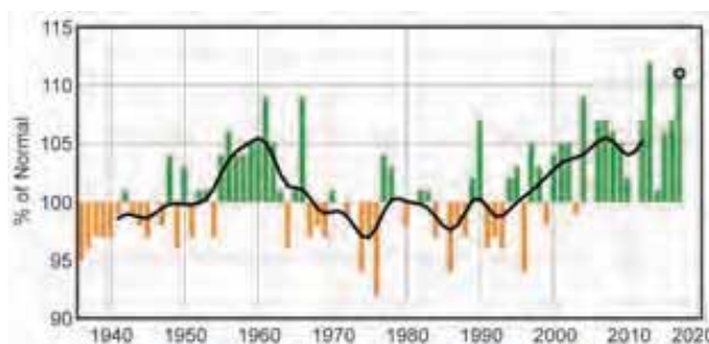
FIG. 7.45. Annual precipitation (% of normal; 1961–90 base period) averaged over Russia for 1936–2017. The smoothed time series (11-point binomial filter) is shown as a bold line.
