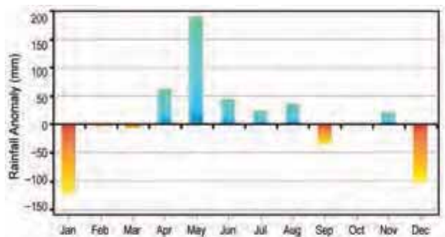
FIG. 7.32. Mean monthly total precipitation anomalies (mm; 1981–2010 base period) over Mauritius in 2017 (Source: Mauritius Meteorological Services.)
