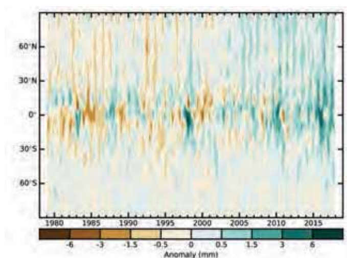
FIG. 2.19. Hovmöller plot of TCWV anomalies (mm; base period 1981–2010) including both land and ocean derived from the JRA-55 reanalysis
