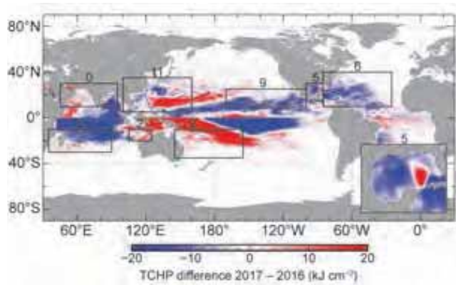
FIG. 4.37. TCHP differences ( \text{kJ cm}^{-2} ) between 2017 and 2016.
