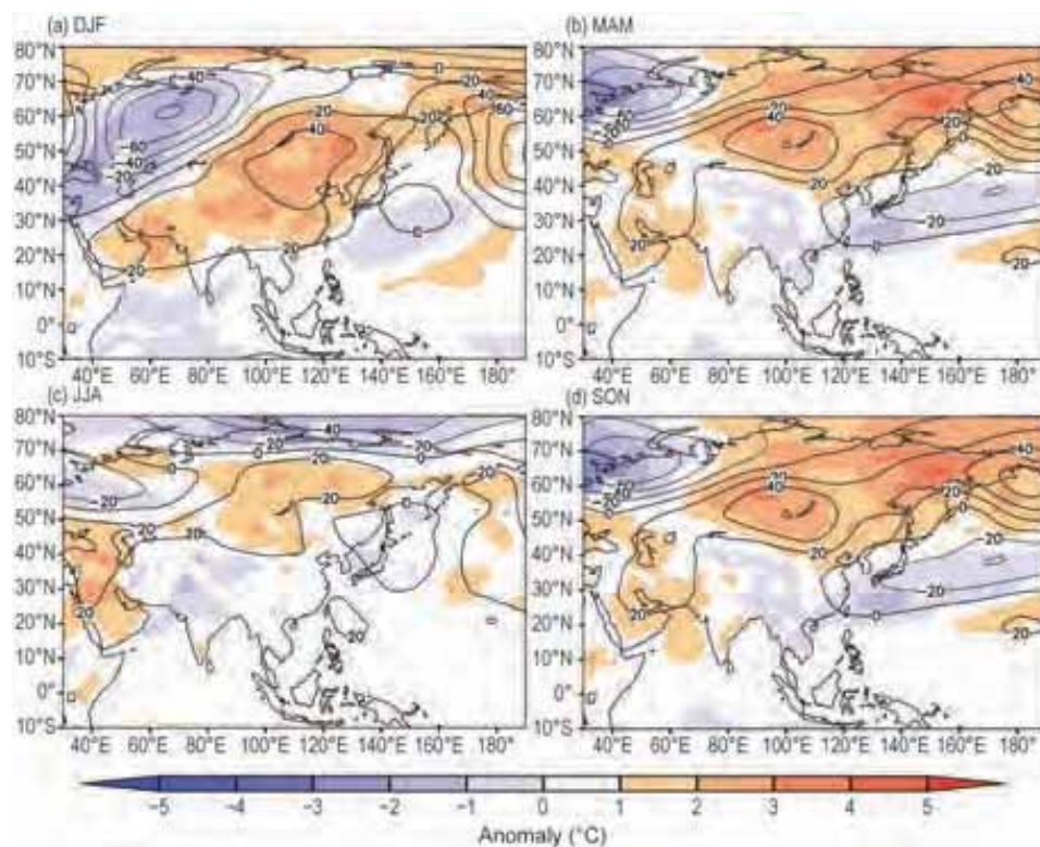
FIG. 7.42. Seasonal mean anomalies of 500-hPa geopotential height (contour, gpm) and 850-hPa temperature (shading, ^{\circ}C ) in 2017 for (a) winter, (b) spring, (c) summer, and (d) autumn, using data from the JRA-55 reanalysis. Base period: 1981–2010. (Source: Japan Meteorological Agency.)
