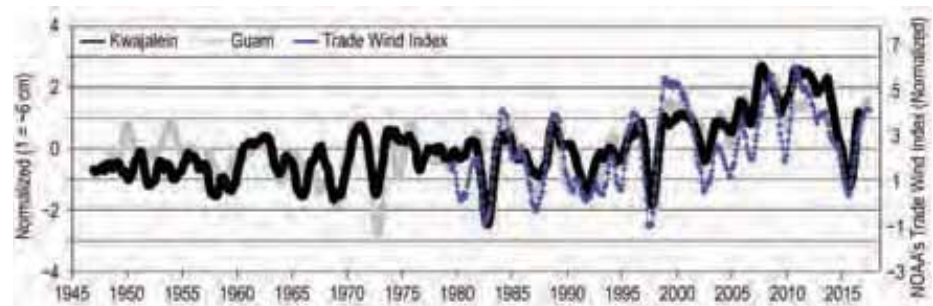
FIG. 7.49. Time series of sea level at Guam (gray line) and Kwajalein (black line) since 1945. Blue line is a time series of NOAA's trade wind index for the region. Note the rapid rise in all times series at the end of the 1990s through the mid-2000s coinciding with La Niña, and also the sharp minima during strong El Niño events (e.g., 1983, 1997, and 2015). There is a sharp rise of sea level in 2016 that remained high during 2017. A 12-month moving average has been applied to the raw monthly values of each time series.
