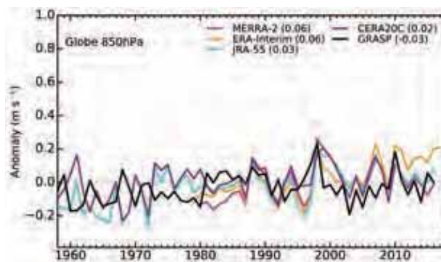
FIG. 2.41. Annual anomalies of global mean wind speed ( \text{m s}^{-1} ; base period 1981–2010) at 850 hPa from four reanalyses and one observational dataset (GRASP; Ramella Pralungo et al. 2014). The numbers in brackets are linear trends in \text{m s}^{-1} \text{ decade}^{-1} ; valid for 1979–2017.
