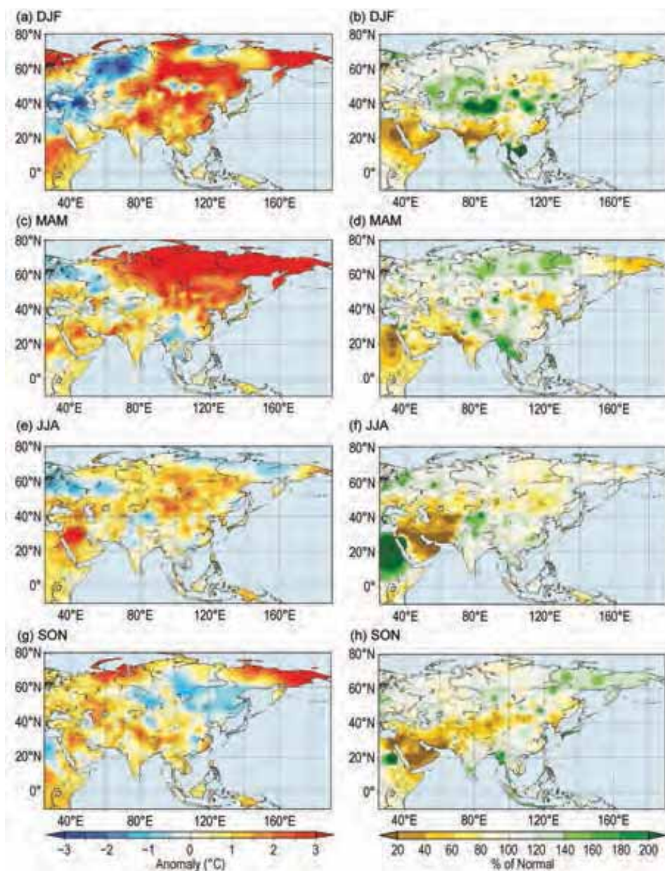
FIG. 7.40. Seasonal mean surface temperature anomalies (°C, left column) and seasonal precipitation (% of normal, right column) over Asia in 2017 for (a), (b) winter; (c), (d) spring; (e), (f) summer; and (g), (h) autumn. All relative to 1981–2010. (Source: Japan Meteorological Agency)
