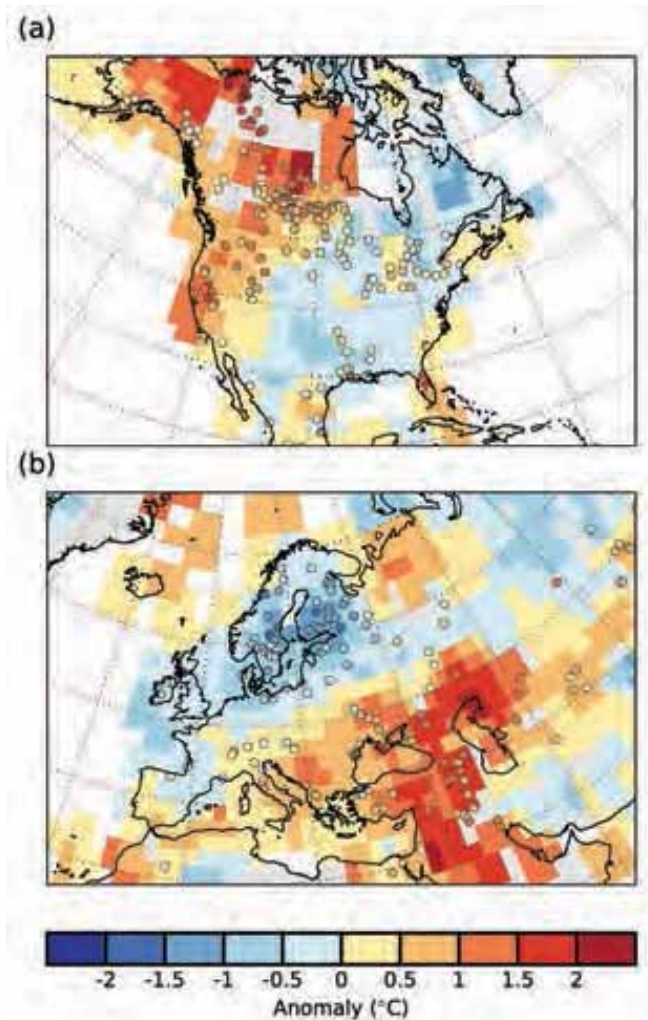
FIG. 2.4. Comparisons of satellite-derived lake surface water temperature anomalies (colored dots) to air surface temperature anomalies (calculated from the NASA GISS Surface Temperature Analysis) in (a) North America and (b) Europe in 2017. Temperatures anomalies (°C; relative to 1996–2015) are calculated for the NH warm season (Jul–Sep).
