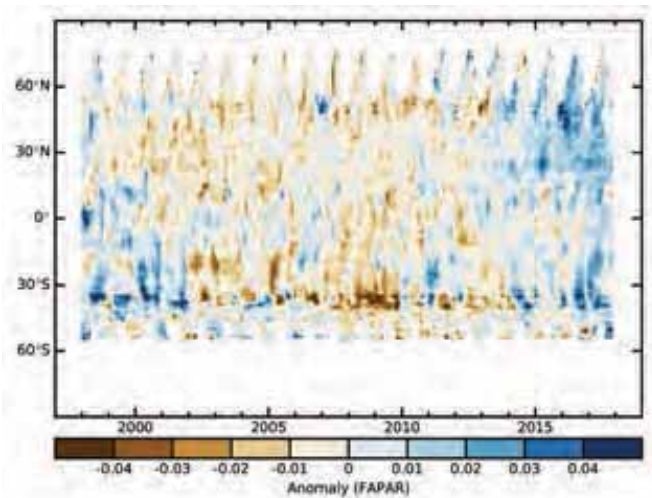
FIG. 2.65. Zonally averaged FAPAR anomalies from 1998–2017.
