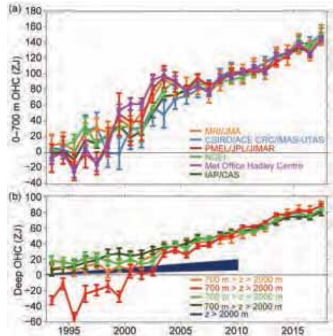
FIG. 3.6. (a) Annual average global integrals of in situ estimates of upper (0–700 m) OHCA ( \text{ZJ} ; 1 \text{ ZJ} = 10^{21} \text{ J} ) for 1993–2017 with standard errors of the mean. The MRI/JMA estimate is an update of Ishii et al. (2017). The CSIRO/ACE CRC/IMAS-UTAS estimate is an update of Domingues et al. (2008). The PMEL/JPL/JIMAR estimate is an update and refinement of Lyman and Johnson (2014). The NCEI estimate follows Levitus et al. (2012). The Met Office Hadley Centre estimate is computed from gridded monthly temperature anomalies (relative to 1950–2016) following Palmer et al. (2007). The IAP/CAS estimate is described in Cheng et al. (2017). See Johnson et al. (2014) for details on uncertainties, methods, and datasets. For comparison, all estimates have been individually offset (vertically on the plot), first to their individual 2005–17 means (the best sampled time period), and then to their collective 1993 mean. (b) Annual average global integrals of in situ estimates of intermediate (700–2000 m) OHCA for 1993–2017 with standard errors of the mean, and a long-term trend with one standard error uncertainty shown from 1992–2010 for deep and abyssal ( z > 2000 \text{ m} ) OHCA following Purkey and Johnson (2010) but updated using all repeat hydrographic section data available from https://cchdo.ucsd.edu/ as of Jan 2018.
