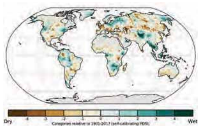
FIG. 2.32. Change in drought (mean scPDSI) from 2016 to 2017. Increases in drought severity are indicated by negative values (brown), decreases by positive values (green). No calculation is made where a drought index is meaningless (gray areas: ice sheets or deserts with approximately zero mean precipitation).
