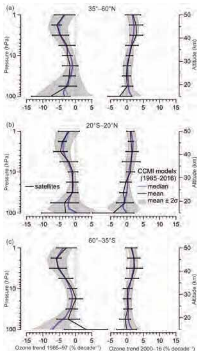
FIG. 2.54. Mean ozone trends in the upper atmosphere (% decade -1 ) prior to 1997 and after 2000 as derived from the CCMI REF-C2 models' simulation (median in blue and mean in purple) and satellite data (black line) in three zonal bands: (a) 35°–60°N (NH), (b) 20°N–20°S (tropics), and (c) 35°–60°S (SH). Mean trends were averaged from trends of individual model runs and various merged datasets shown in Fig. 2.53. The shading shows the 2σ of the models' mean trend. Same type of multilinear regression analysis was used to determine the trends in models and observations. Adapted from LOTUS (2018, SPARC report under review).
