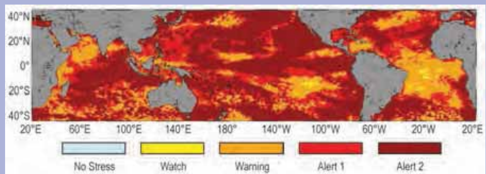
FIG. SB3.2. NOAA CRW Maximum Bleaching Alert Area map for Jun 2014–May 2017. Data from CRW's Daily Global 5-km Coral Bleaching Heat Stress Monitoring Product Suite v.3 (G. Liu et al. 2017).
