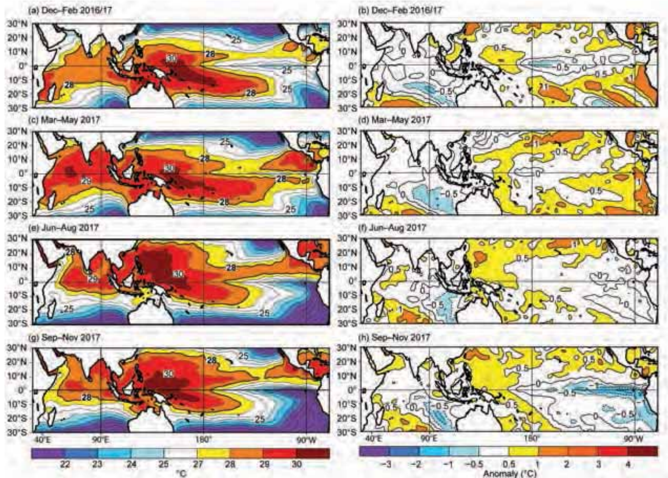
FIG. 4.2. Seasonal SST (left) and anomaly (right) for (a),(b) DJF 2016/17; (c),(d) MAM 2017; (e),(f) JJA 2017; and (g),(h) SON 2017. Contour interval for seasonal SST is 1^{\circ}\text{C} . For anomalous SST, contour interval is 0.5^{\circ}\text{C} for anomalies between \pm 1^{\circ}\text{C} , and 1^{\circ}\text{C} for anomalies > \pm 1^{\circ}\text{C} . Anomalies are departures from the 1981–2010 seasonal adjusted OI climatology (Reynolds et al. 2002).
