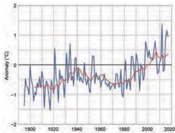
FIG. 7.3. Annual mean temperature anomalies (°C; 1981–2010 base period) for the contiguous United States for 1895–2017. Red line is the 10-year running mean. (Source: NOAA/NCEI.)
