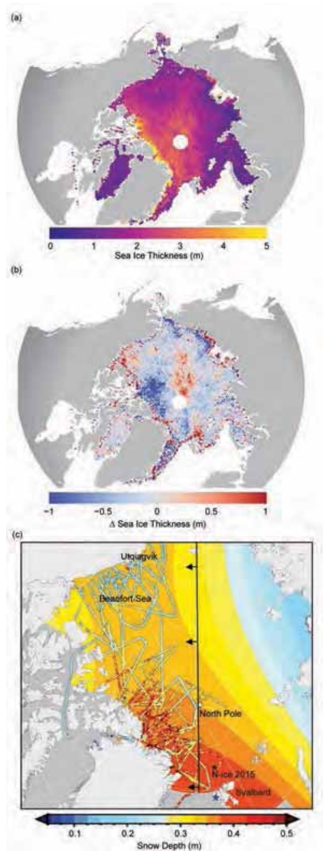
FIG. 5.10. Apr 2017 (a) sea ice thickness (m) derived from CryoSat-2 radar altimeter data and (b) sea ice thickness anomaly (m; base period 2011–16). (c) Snow depth (m) on Arctic sea ice at the end of winter, prior to melt onset; recent in situ measurements (stars), made in 2015 and 2017, and airborne observations (multiple airborne survey lines), made in Mar and May in 2009–12 and 2014–15, are overlaid on the long term mean snow depth for the months of Mar and Apr (adapted from Warren et al. 1999). Black line and arrows in (c) designate the western Arctic.
