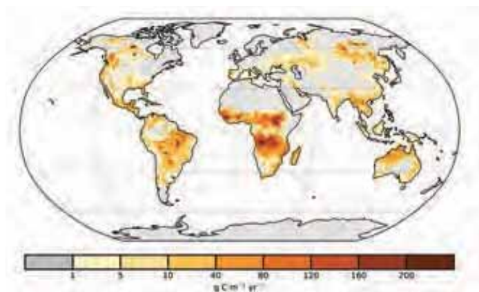
FIG. 2.67. Global map of fire activity in 2017 in terms of carbon consumption ( \text{g C m}^{-2} \text{ yr}^{-1} ). (GFASv1.4)
