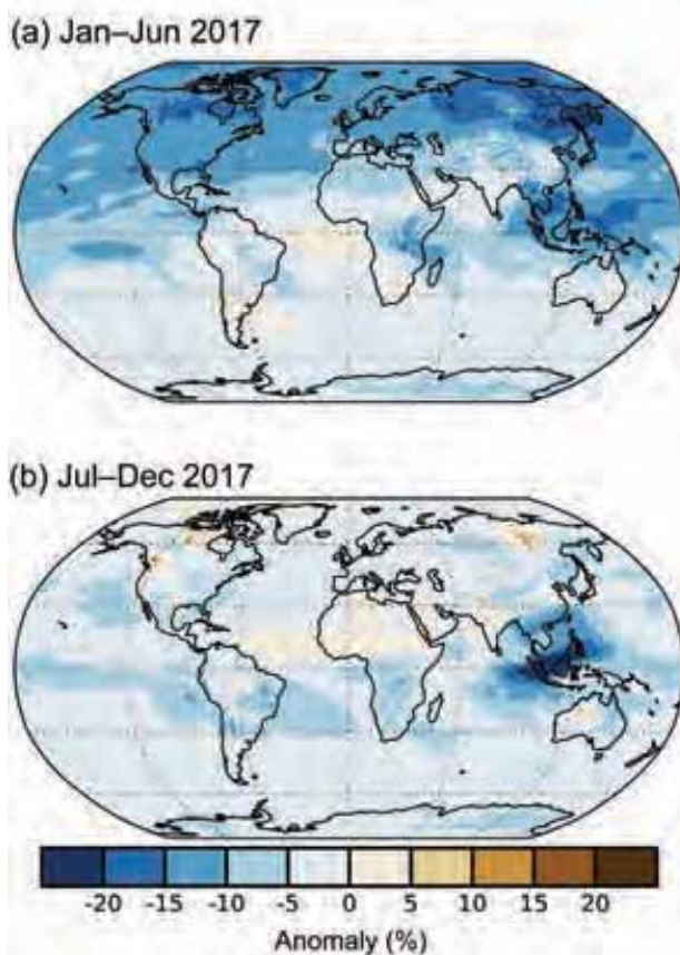
FIG. 2.62. Total column CO anomalies (%) for (a) Jan–Jun 2017 and (b) Jul–Dec 2017 with respect to 2003–17 median from the CAMS interim reanalysis.
