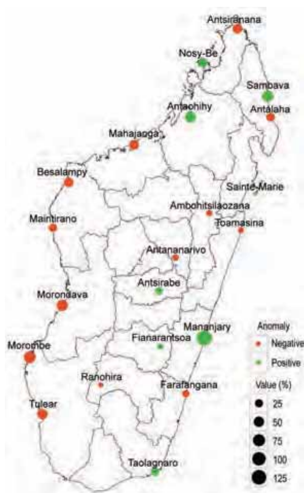
FIG. 7.31. Annual total precipitation anomalies (% of average; 1981–2010 base period) for Madagascar in 2017. (Source: Madagascar Meteorological Services.)
