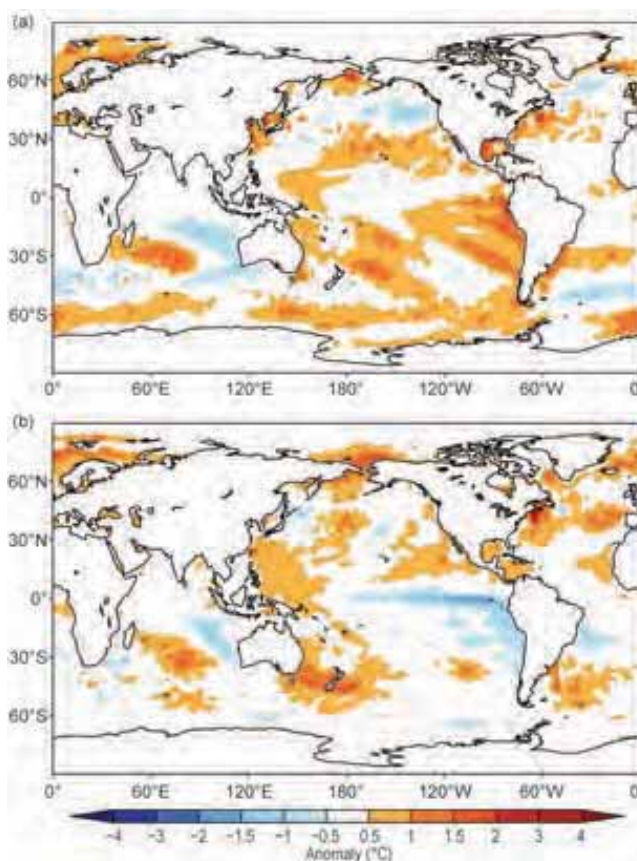
FIG. 4.13. Spatial distribution global SST anomalies ( ^{\circ}\text{C} ; Reynolds et al. 2002) for (a) Jan–Apr and (b) Sep–Dec 2017.
