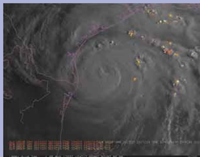
FIG. SB4.4. GOES-16 ABI Band 1 (0.47 \mu\text{m} ) and color-coded GLM parallax-corrected observations of lightning groups in the 5 minutes prior to the nominal time of the ABI image (red: oldest; yellow: latest), 1247 UTC on 25 Aug 2017, just prior to the rapid intensification of Hurricane Harvey.
