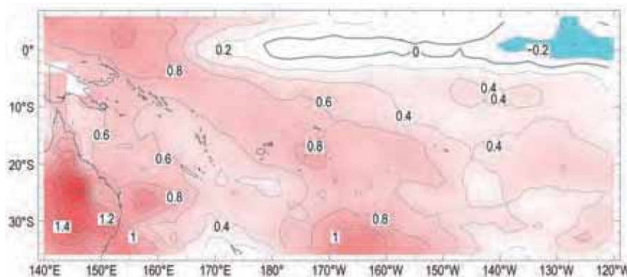
Fig. 7.50. Annual average surface air temperature anomalies ( ^{\circ}\text{C} , 1981–2010 base period; Source: NOAA NCEP CPC CAMS.)
