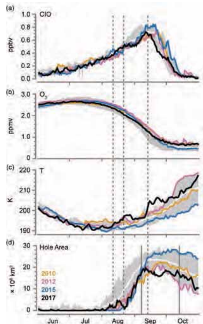
FIG. 6.11. Antarctic vortex-averaged concentrations of: (a) CIO and (b) ozone from Aura MLS (updated from Manney et al. 2011). These MLS averages are made inside the polar vortex on the 440-K isentropic surface ( \sim 18 \text{ km} or 65 hPa). (c) Temperature on the 440-K isentropic surface over Antarctica ( 60^\circ\text{--}90^\circ\text{S} ) from MERRA-2 (Gelaro et al. 2017). (d) Ozone hole area based on Ozone Monitoring Instrument (OMI) and Ozone Mapping and Profiler Suite (OMPS) satellite observations. Four years are shown: 2010 (orange), 2012 (pink), 2015 (blue), and 2017 (black). The white line shows the daily average and the gray shading shows the daily ranges for 2005–16. The vertical solid lines indicate the averaging period for Fig. 6.13, while the vertical dashed lines indicate the dates of maximum wave forcing for the stratospheric warming events in 2017.
