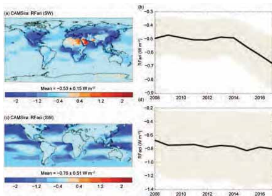
FIG. 2.51. Radiative forcing (W m -2 ) in the SW spectrum resulting from (a) RFar and (c) RFaci from 2008–17. (b,d) The uncertainties of these estimates are shown in gray.
