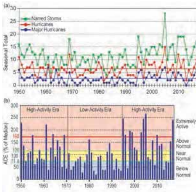
FIG. 4.19. Seasonal Atlantic hurricane activity during 1950–2017 based on HURDAT2 (Landsea and Franklin 2013). (a) Number of named storms (green), hurricanes (red), and major hurricanes (blue), with 1981–2010 seasonal means shown by solid colored lines. (b) ACE index expressed as percent of the 1981–2010 median value. ACE is calculated by summing the squares of the 6-hourly maximum sustained surface wind speed (knots) for all periods while the storm is at least tropical storm strength. Red, yellow, and blue shadings correspond to NOAA's classifications for above-, near-, and below-normal seasons, respectively ( www.cpc.ncep.noaa.gov/products/outlooks/background_information.shtml ). The thick red horizontal line at 165% ACE value denotes the threshold for an extremely active season. Vertical brown lines separate high- and low-activity eras.
