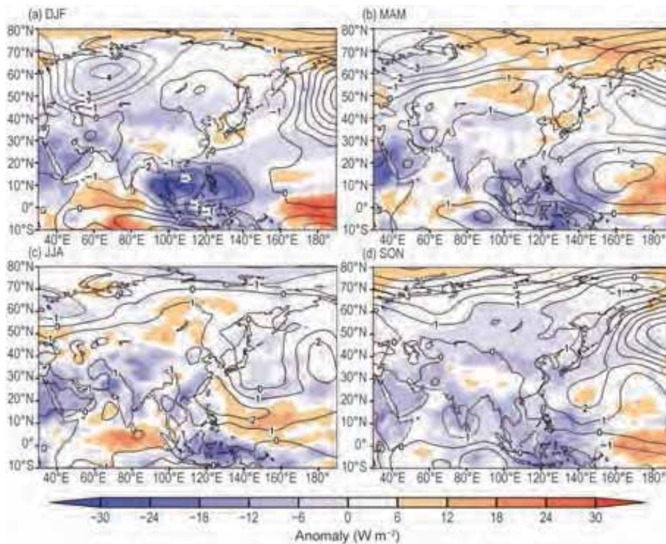
FIG. 7.41. Seasonal mean anomalies of 850-hPa stream function (contour, 1 \times 10^6 m^2 s^{-1} ) using data from the JRA-55 reanalysis and OLR (shading, W m^{-2} ) using data originally provided by NOAA in 2017 for (a) winter, (b) spring, (c) summer, and (d) autumn. Base period: 1981–2010. (Source: Japan Meteorological Agency.)
