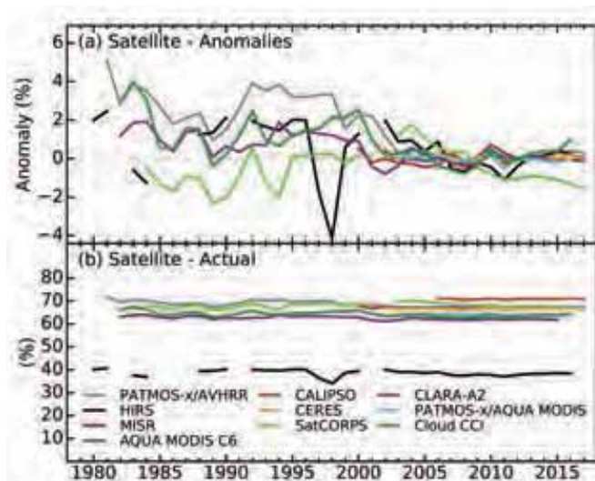
FIG. 2.23. (a) Annual global cloudiness anomalies (%) for 1981–2017, defined as the annual value minus the mean, derived between 2003 and 2015, a period common to the satellite records excluding CALIPSO, where the entire record was used instead. (b) Annual actual global cloudiness (%). The datasets include PATMOS-x/AVHRR, HIRS High Cloud, MISR, Aqua MODIS C6, CALIPSO, CERES Aqua MODIS, SatCORPS, CLARA-A2, PATMOS-x/Aqua MODIS, and CLOUD_CCI.
