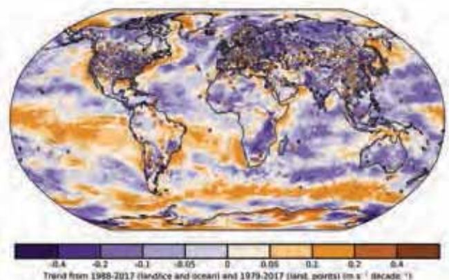
FIG. 2.39. Wind speed trends ( \text{m s}^{-1} \text{ decade}^{-1} ) for the observational HadISD2 and Australian datasets (circles) over land for 1979–2017, and MERRA2 over land/ice and RSS over ocean for 1988–2017 (shaded areas).
