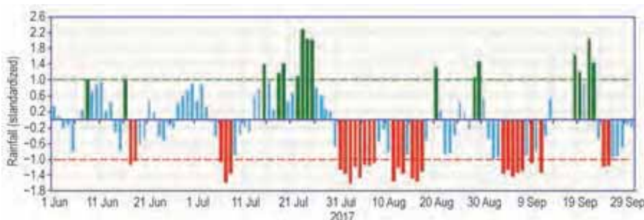
FIG. 7.48. Daily standardized rainfall time series averaged over the core monsoon zone of India (1 Jun–30 Sep 2017).
