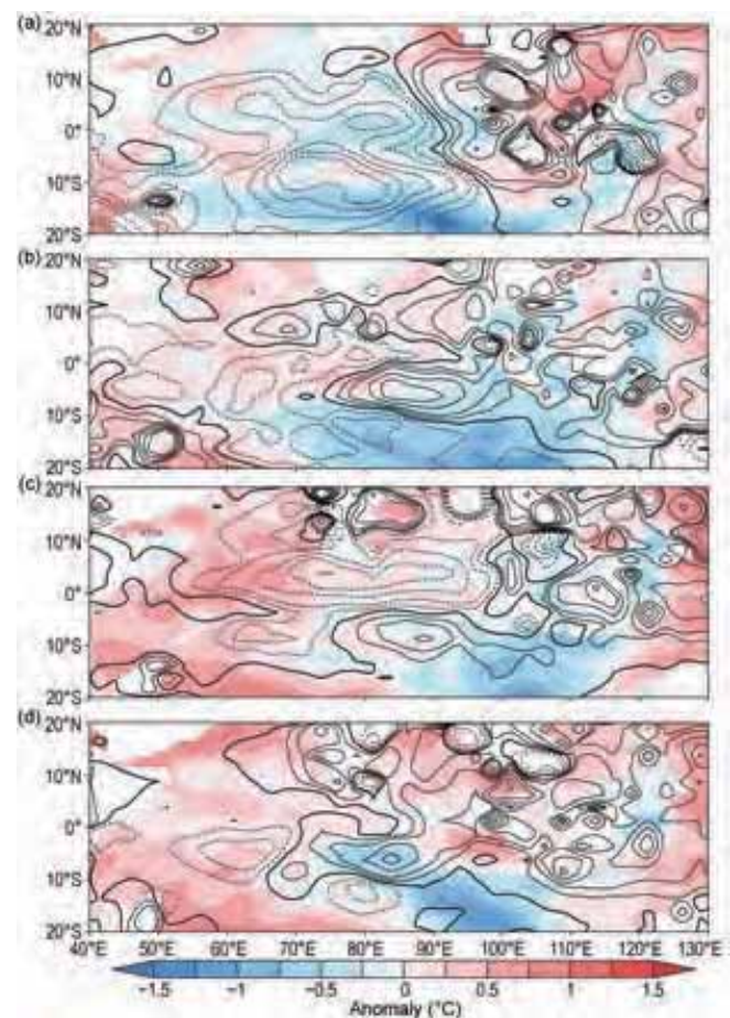
FIG. 4.41. SST ( ^{\circ}\text{C} ; colors) and precipitation (contoured at: 0, \pm 0.5 , \pm 1 , \pm 2 , \pm 3 , \pm 4 , and \pm 5 \text{ mm day}^{-1} ). Solid/dashed lines denote positive/negative values, and thick solid lines indicate the zero contour) anomalies during (a) Dec 2016–Feb 2017, (b) Mar–May 2017, (c) Jun–Aug 2017, and (d) Sep–Nov 2017. Anomalies were calculated relative to 1982–2017. [Sources: NOAA OISST (Reynolds et al. 2002) and monthly GPCP precipitation analysis (available at http://precip.gsfc.nasa.gov/ ).]
