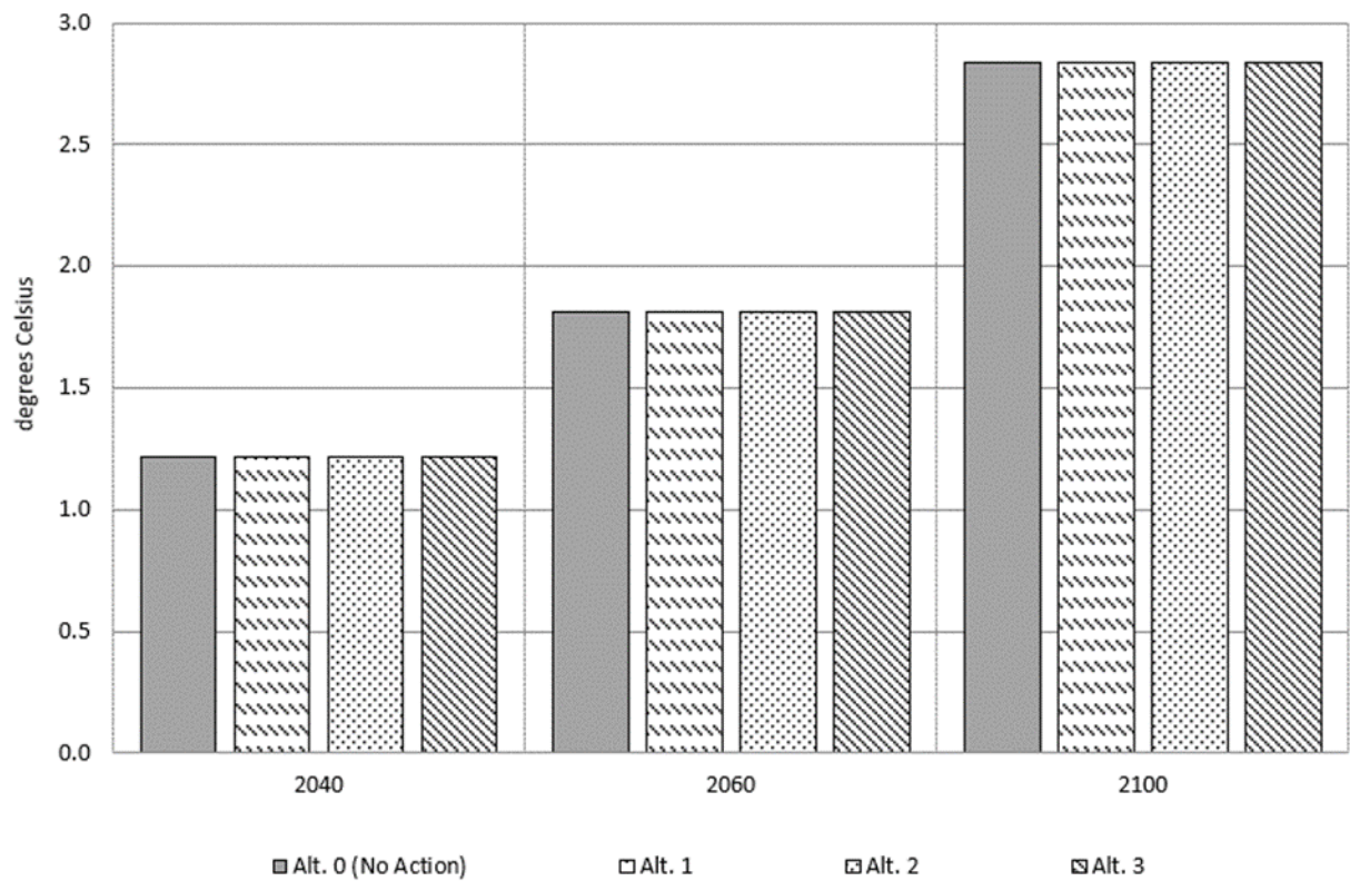
Figure 8.6.4-3. Global Mean Surface Temperature Increase by Alternative
