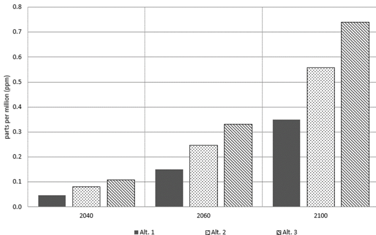
Figure 8.6.4-2. Reductions in Atmospheric Carbon Dioxide Concentrations Compared to the No Action Alternative
