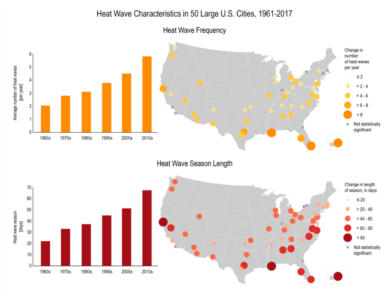
Figure 5.2.2-3. Heat Waves Increasing in Frequency and Duration from 1961 to 2017
