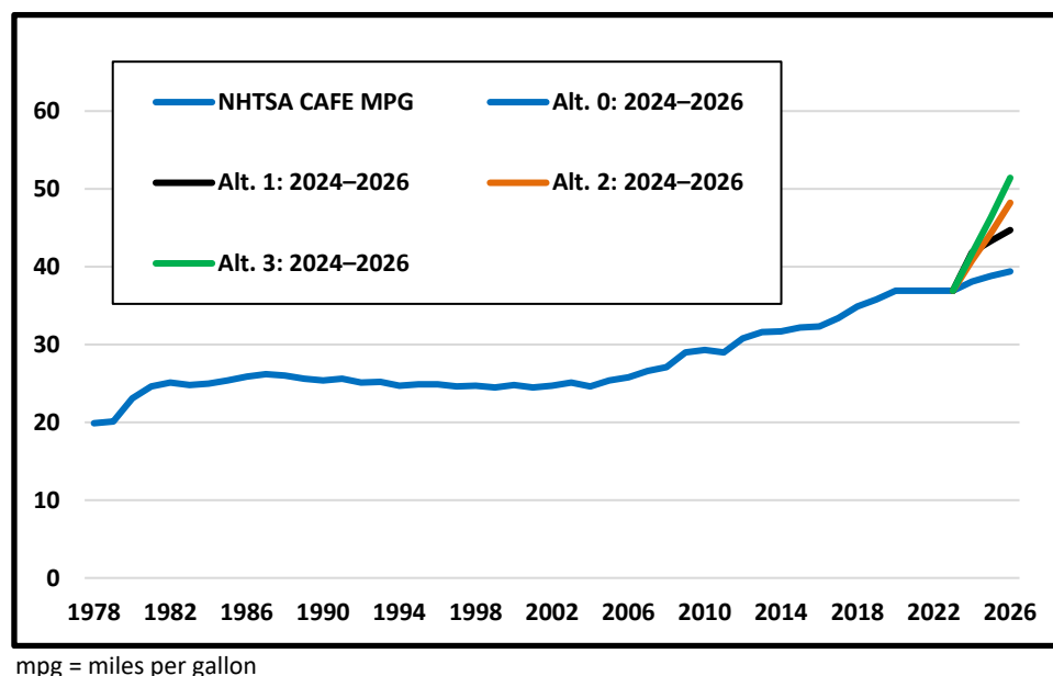
Figure 2.2.3-1. Historical CAFE Fuel Economy Requirements for Passenger Cars and Light Trucks through MY 2023 and Range of Projected EIS Alternative Standards through MY 2026
