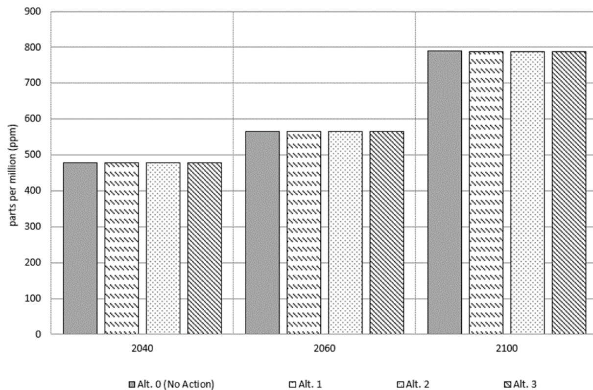
Figure 5.4.2-1. Atmospheric Carbon Dioxide Concentrations by Alternative
