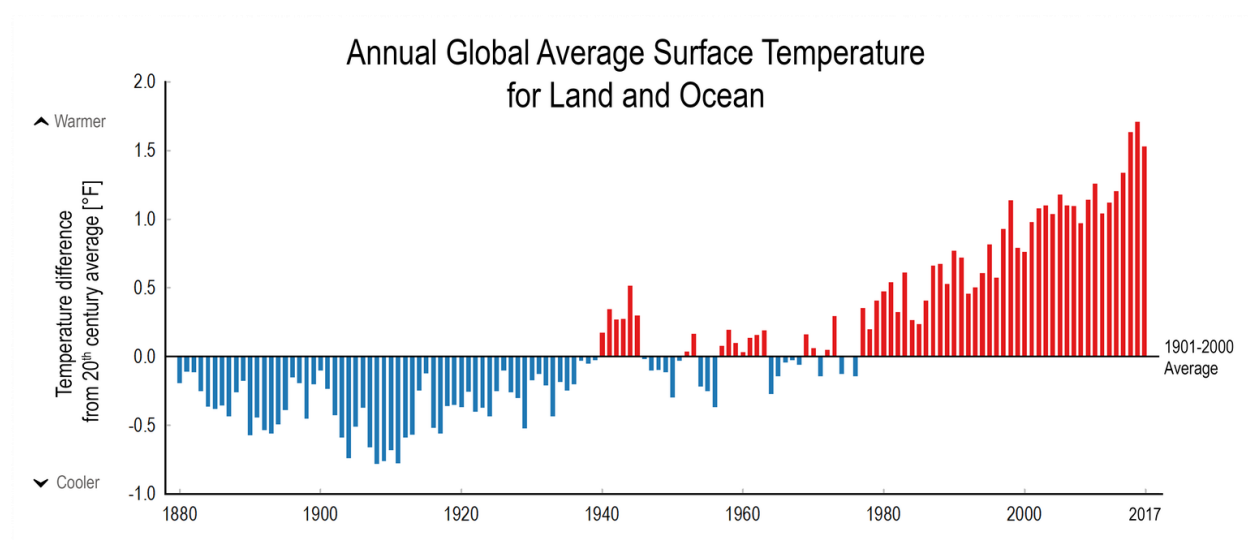
Figure 5.2.2-2. Annual Global Average Surface Temperature Increases of About 0.9°C (1.6°F) from 1880 to 2016
