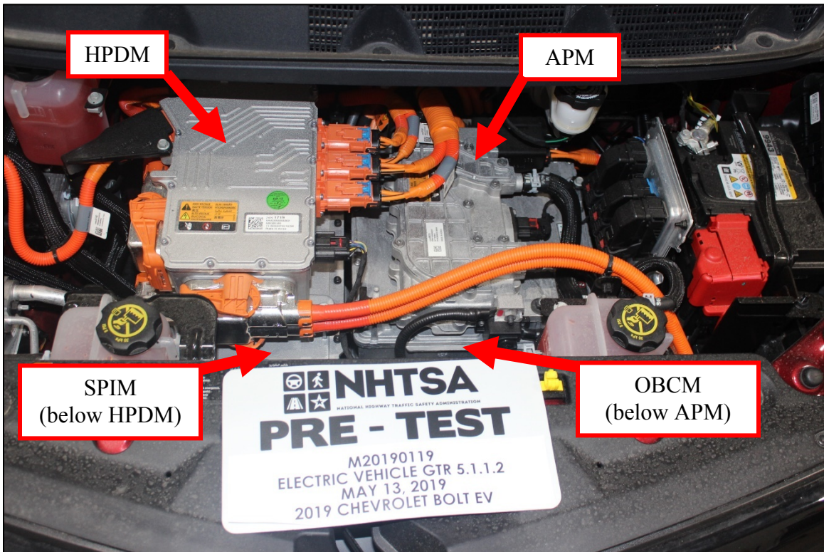
Figure 6: Vehicle Front Compartment
