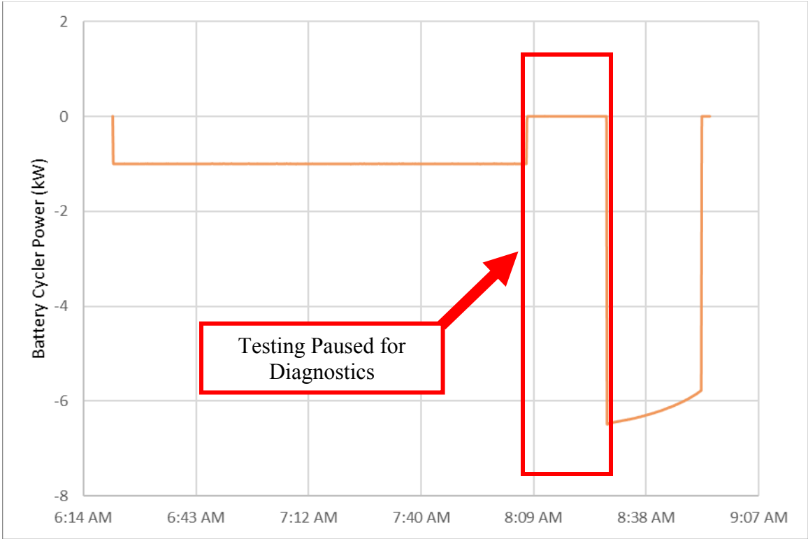
Figure 36: Over-Discharge Test Battery Tester Power
