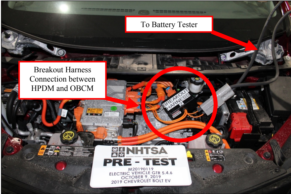
Figure 22: Over-Charge Breakout Harness
