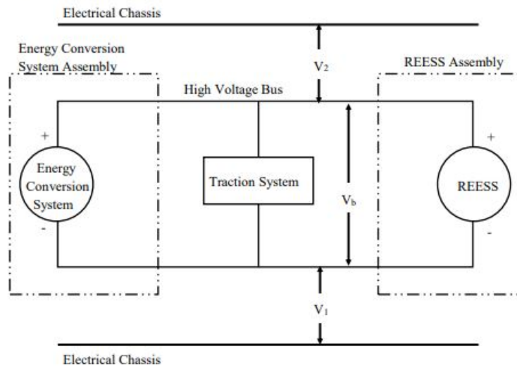
Figure 2 Measurement of V_b , V_1 , V_2
