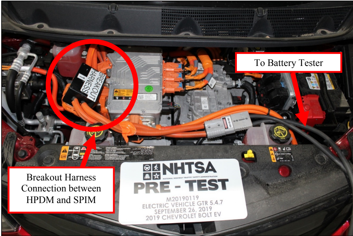
Figure 30: Over-Discharge Breakout Harness
