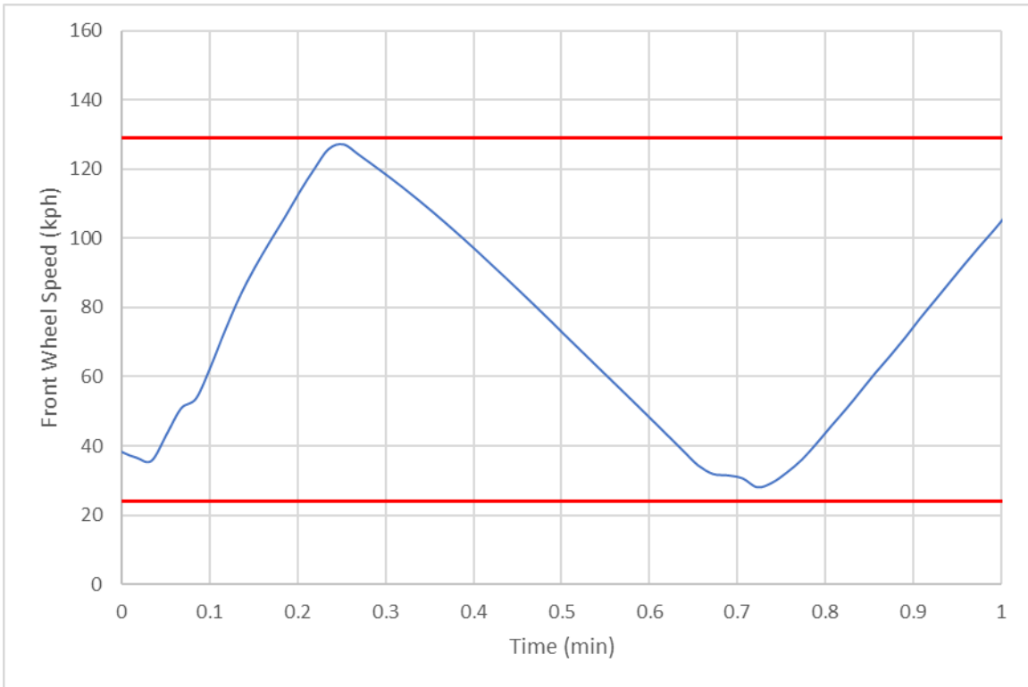
Figure 42: Over-Temperature Test Vehicle Drive Profile – Single Cycle
