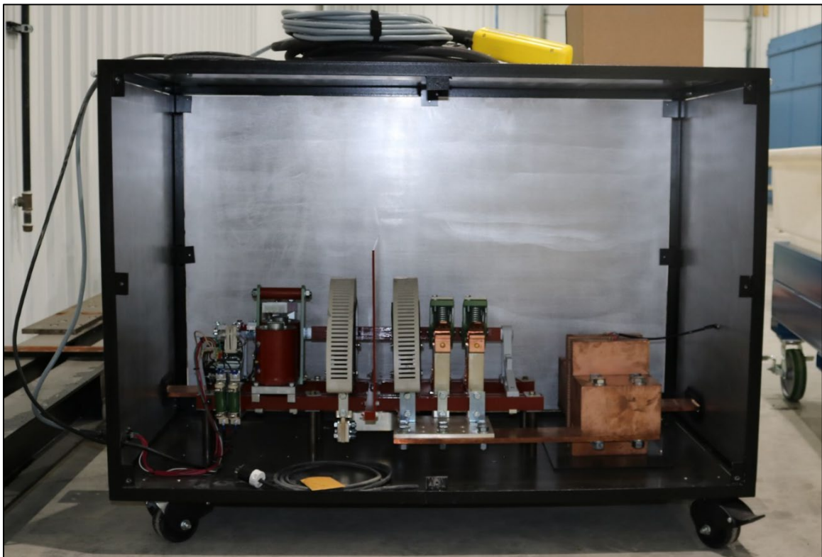
Figure 17: External Short Circuit Contactor
