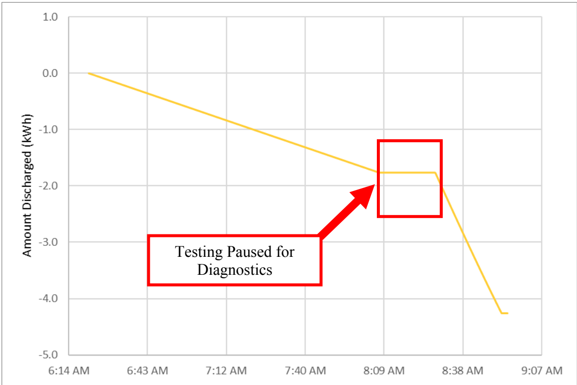
Figure 37: Over-Discharge Test Battery Tester Amount Discharged
