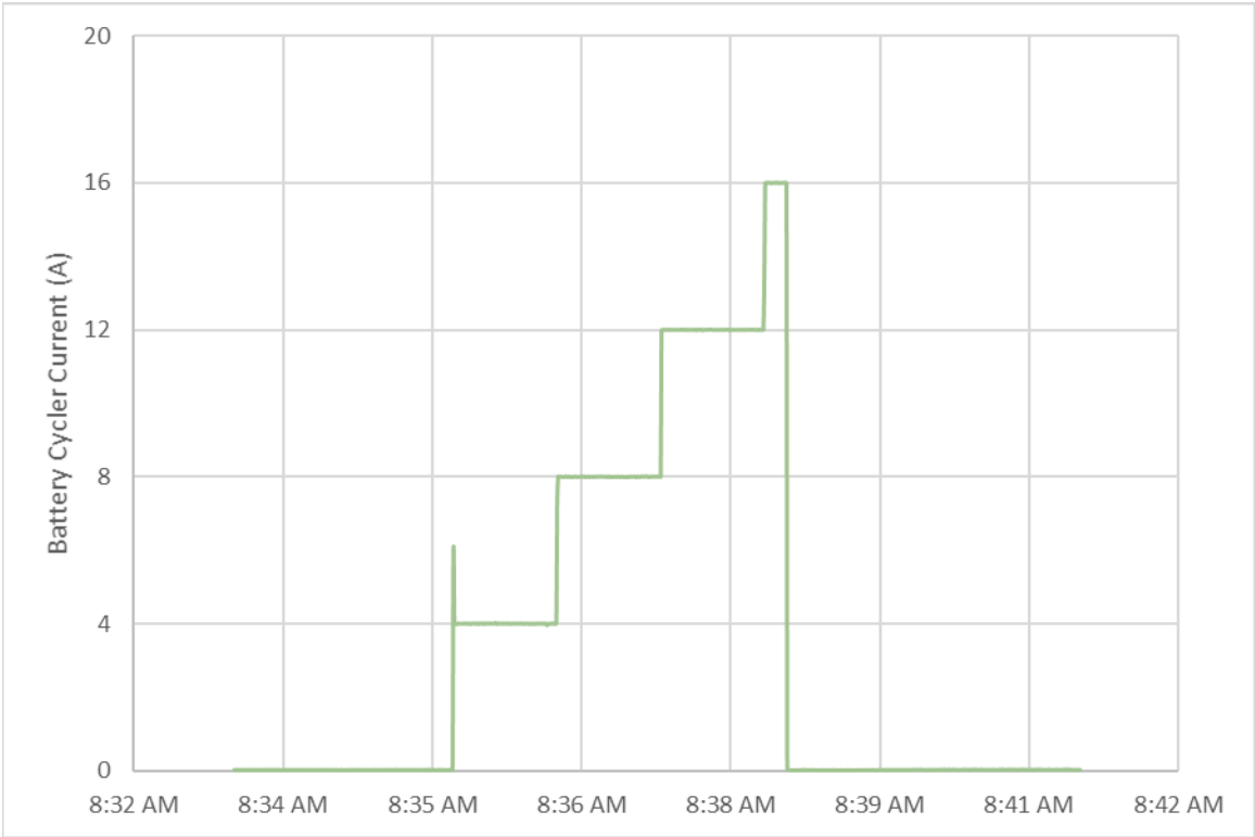
Figure 53: Over-Current Test Battery Tester Current
