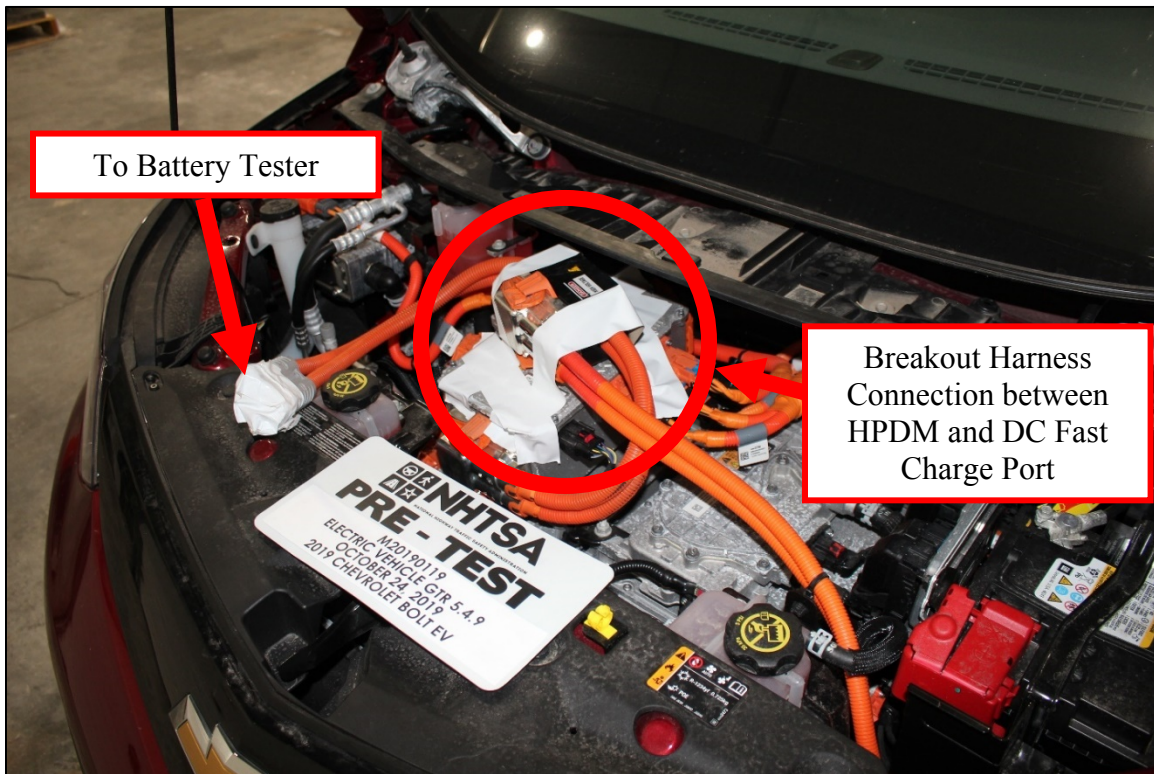
Figure 48: Over-Current Breakout Harness
