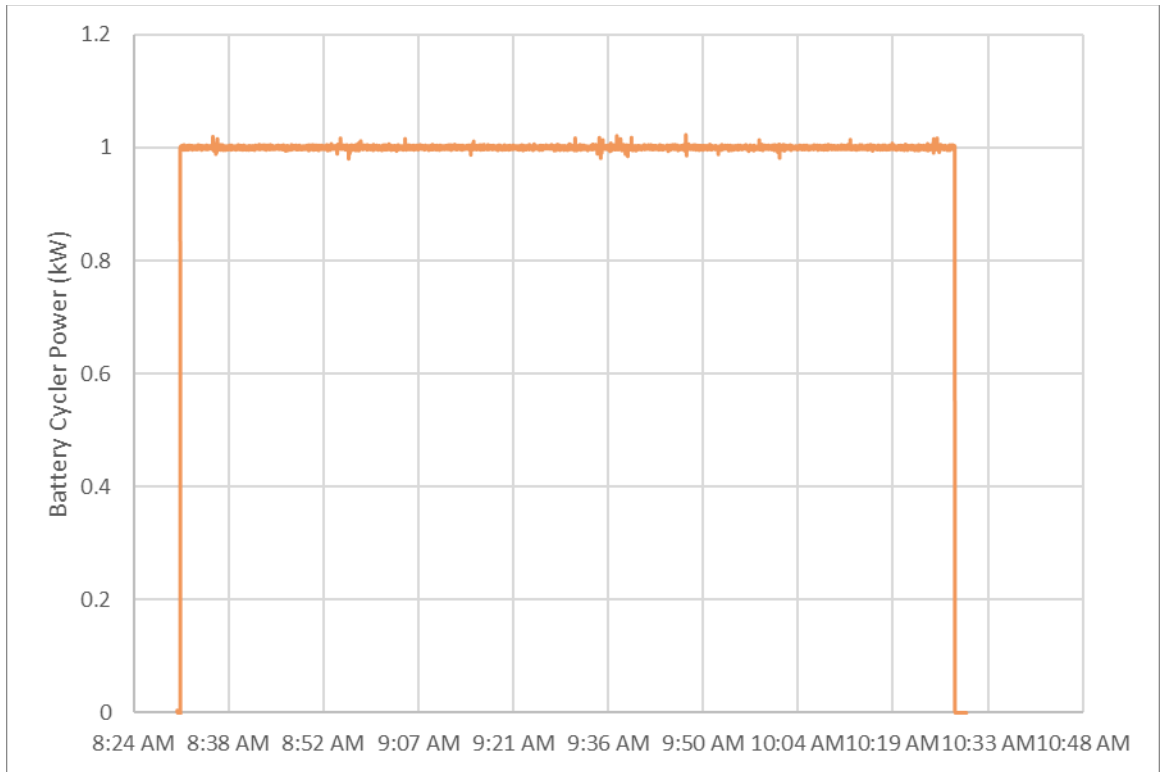
Figure 28: Over-Charge Test Battery Tester Power
