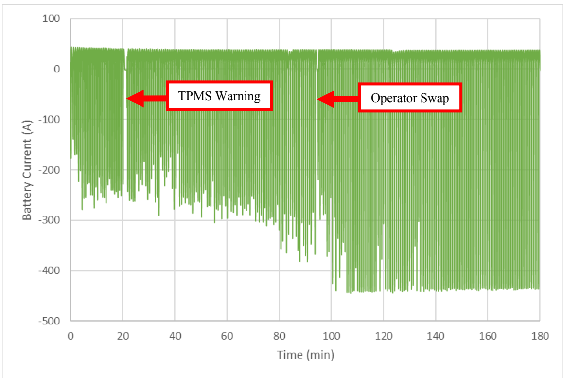
Figure 46: Over-Temperature Test Battery Current
