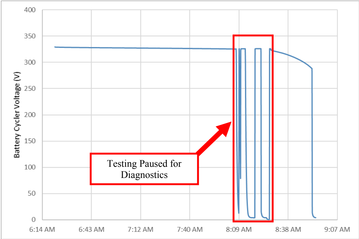
Figure 34: Over-Discharge Test Battery Tester Voltage
