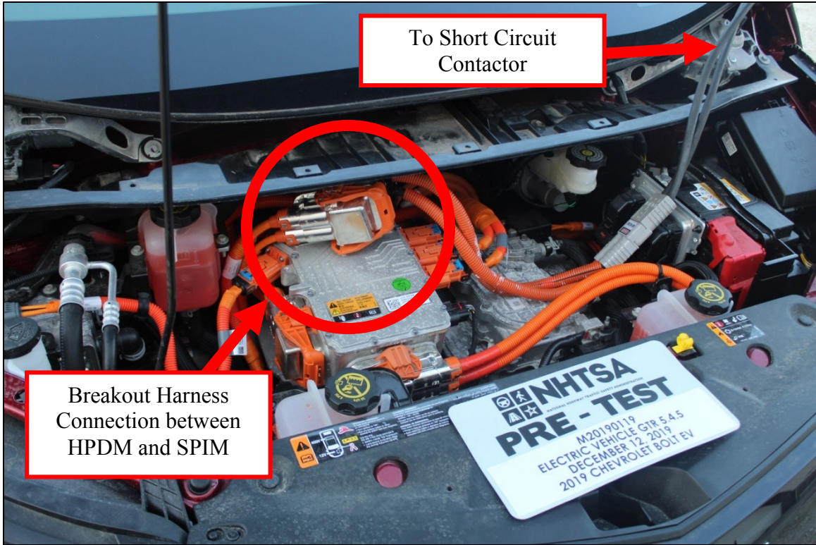
Figure 16: External Short Circuit Breakout Harness
