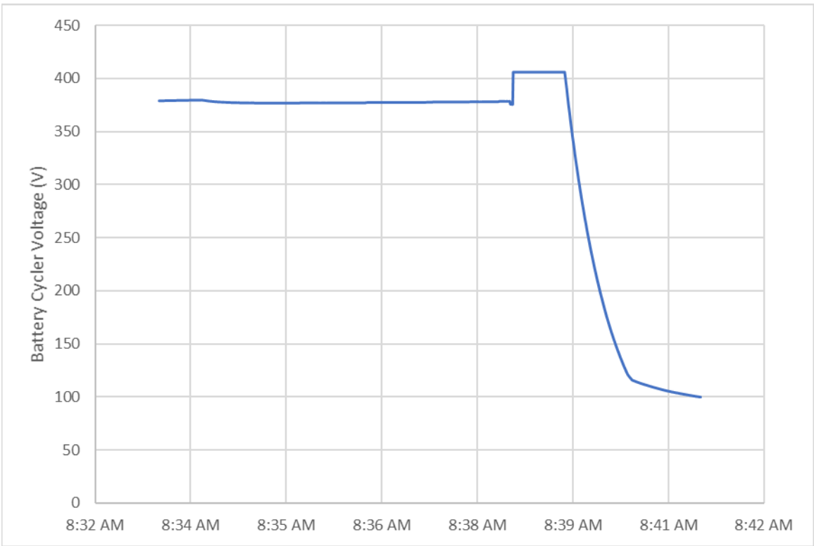
Figure 52: Over-Current Test Battery Tester Voltage
