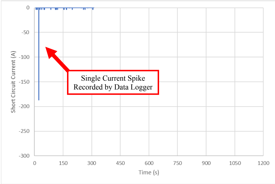
Figure 18: External Short Circuit Test Shunt Current at 1,000 sps
