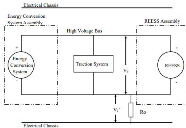
Figure 3 Measurement of V_1'
