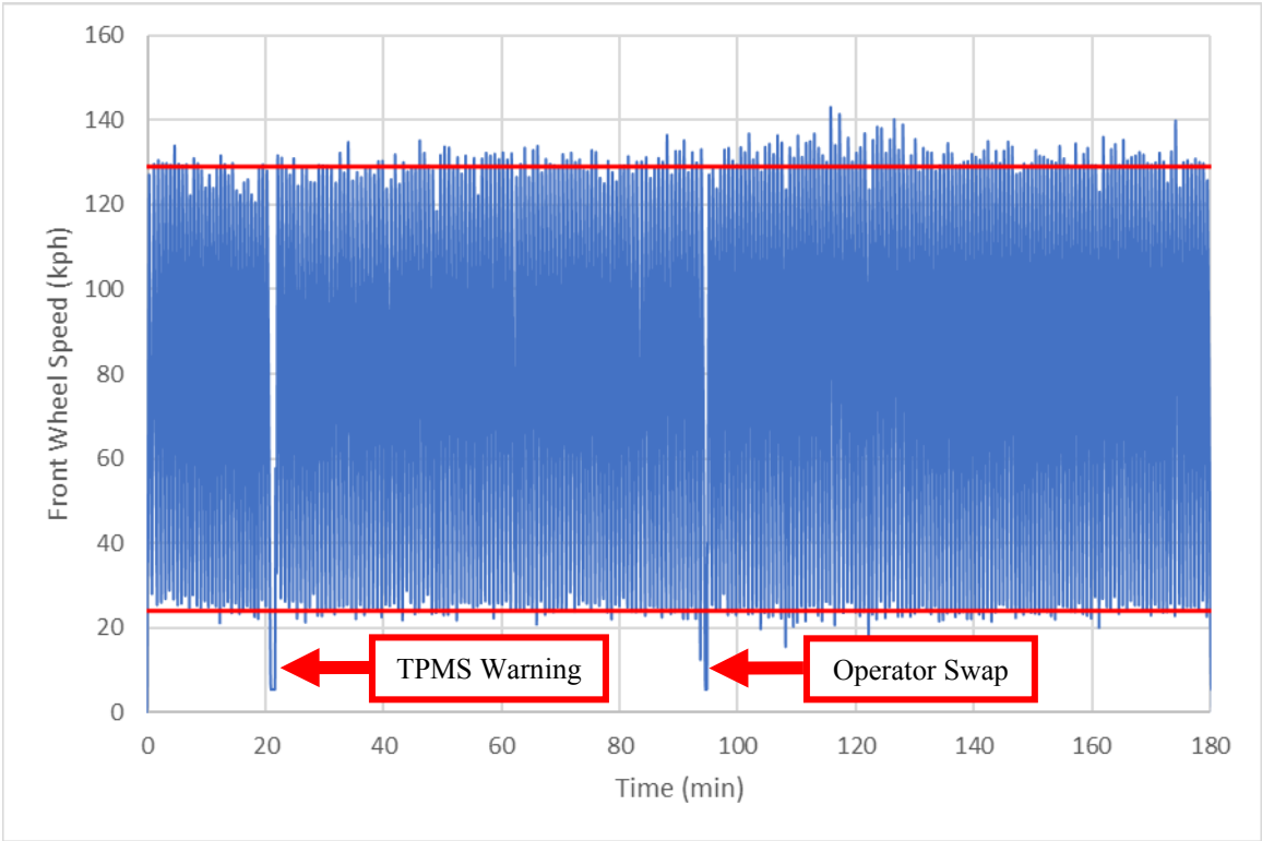
Figure 43: Over-Temperature Test Vehicle Drive Profile
