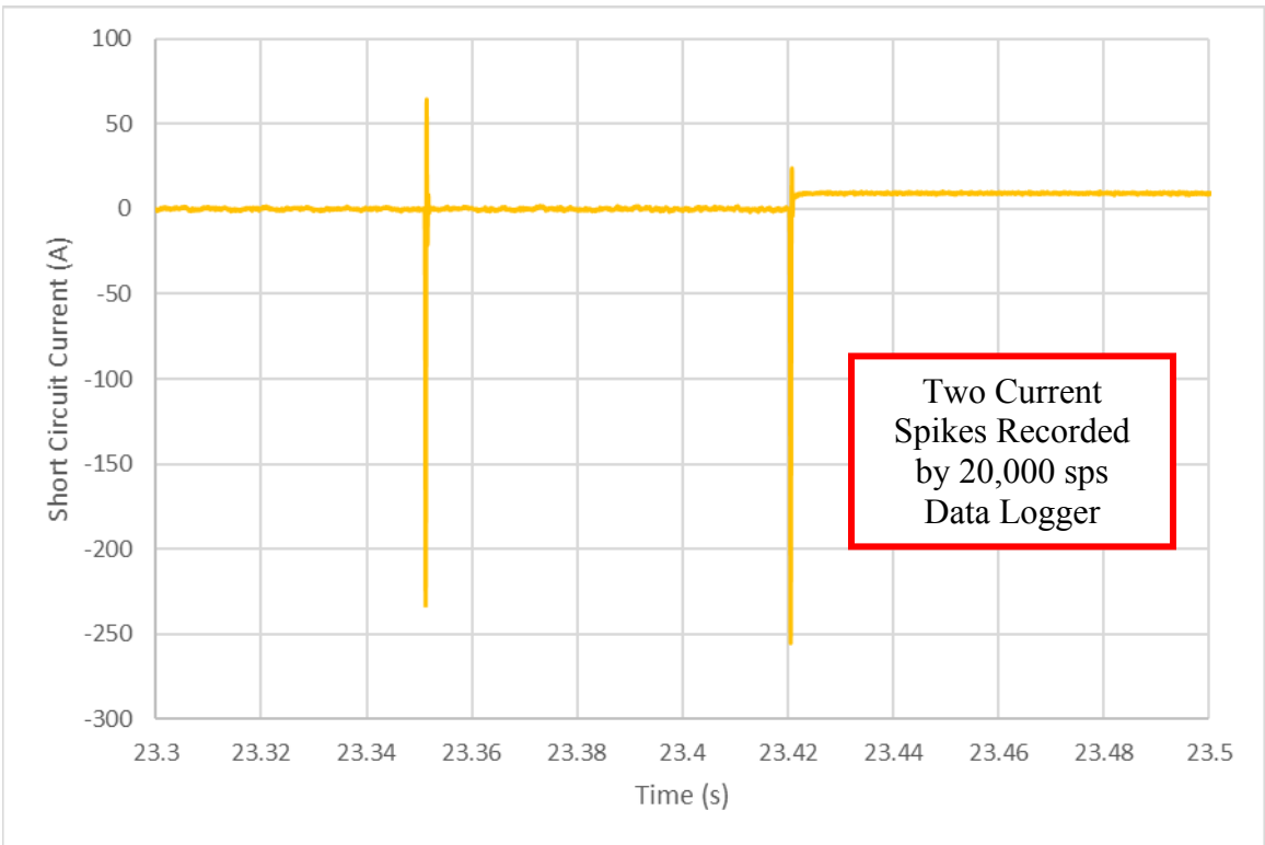
Figure 21: External Short Circuit Test Shunt Current at 20,000 sps
