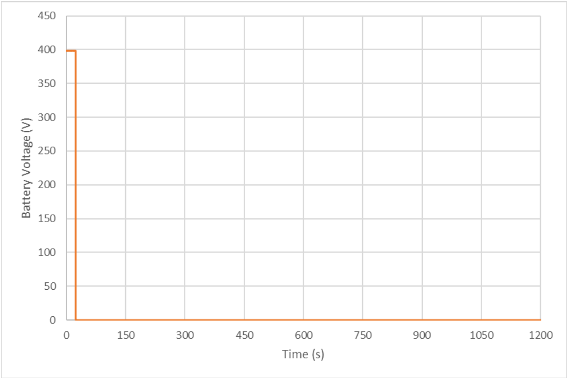
Figure 20: External Short Circuit Test Battery Voltage
