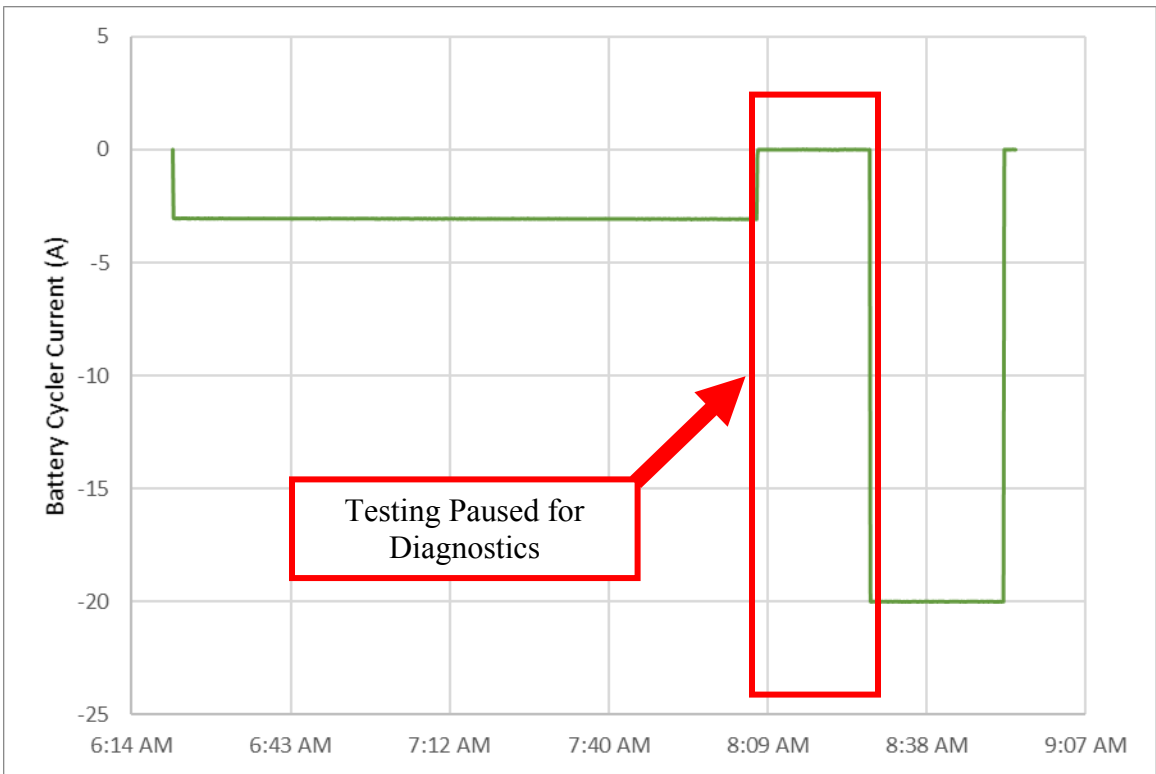
Figure 35: Over-Discharge Test Battery Tester Current
