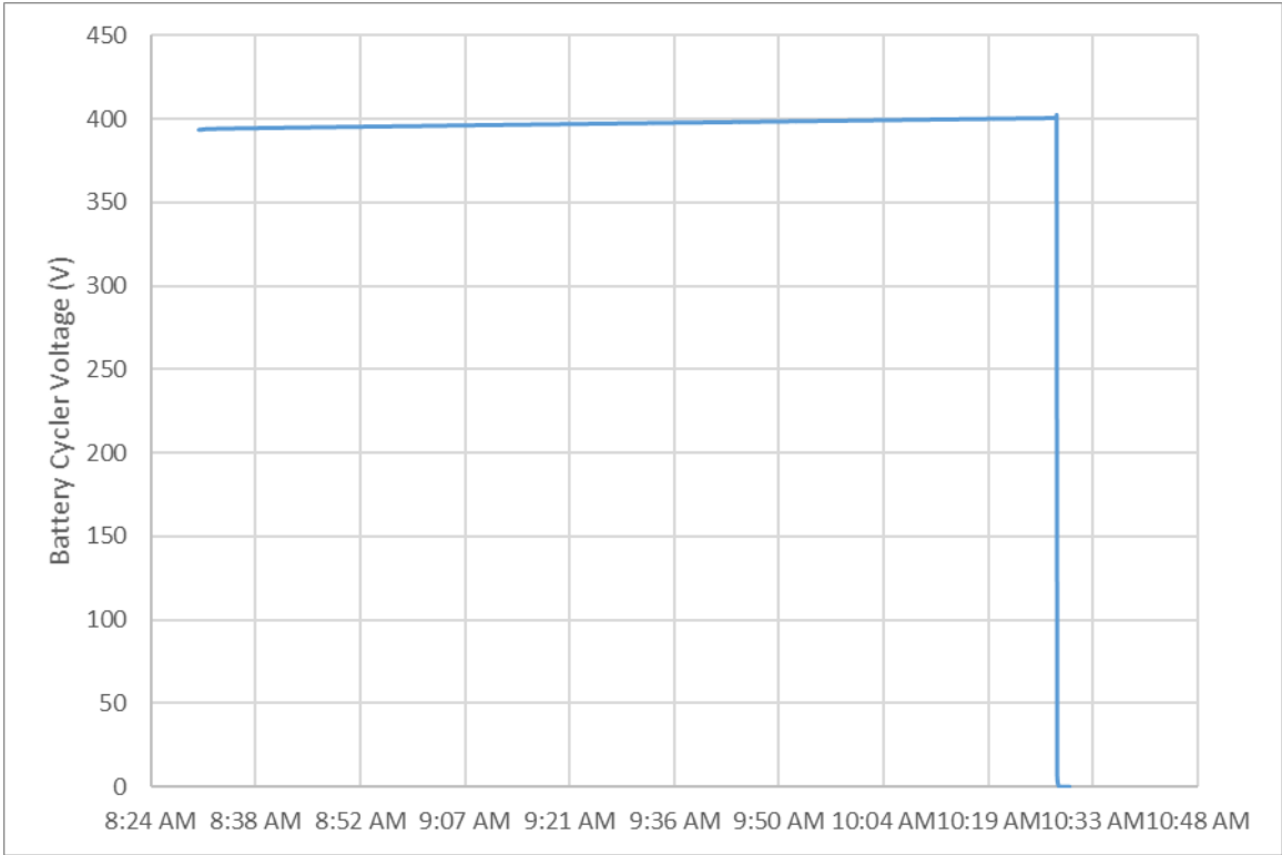
Figure 26: Over-Charge Test Battery Tester Voltage
