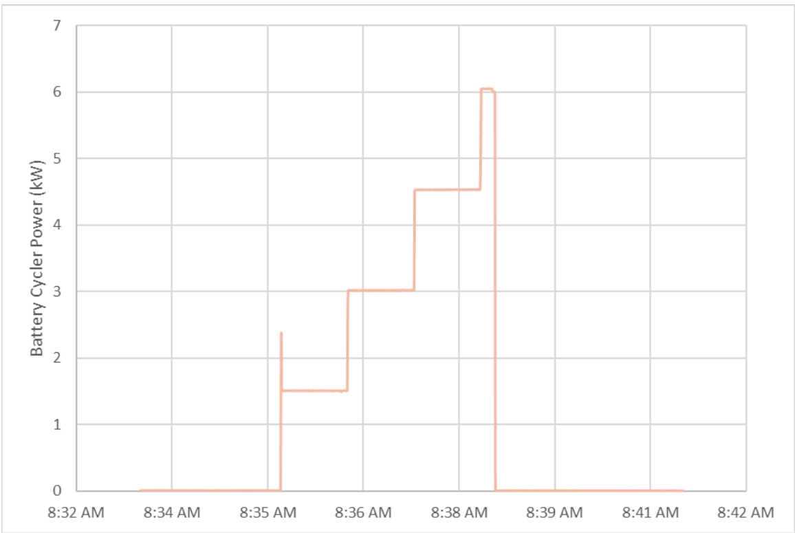
Figure 54: Over-Current Test Battery Tester Power
