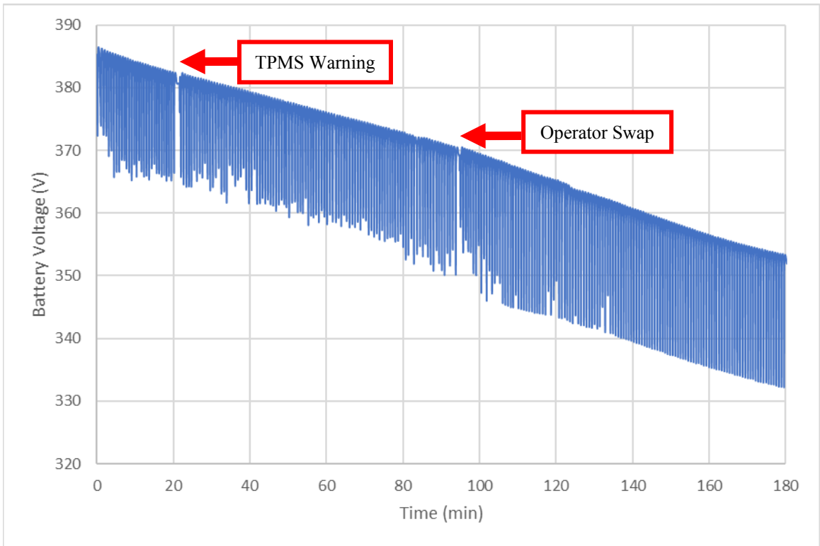
Figure 45: Over-Temperature Test Battery Voltage
