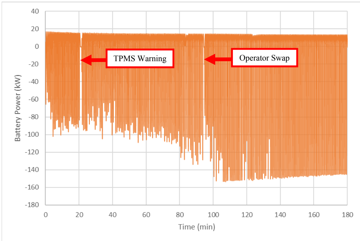
Figure 47: Over-Temperature Test Battery Power
