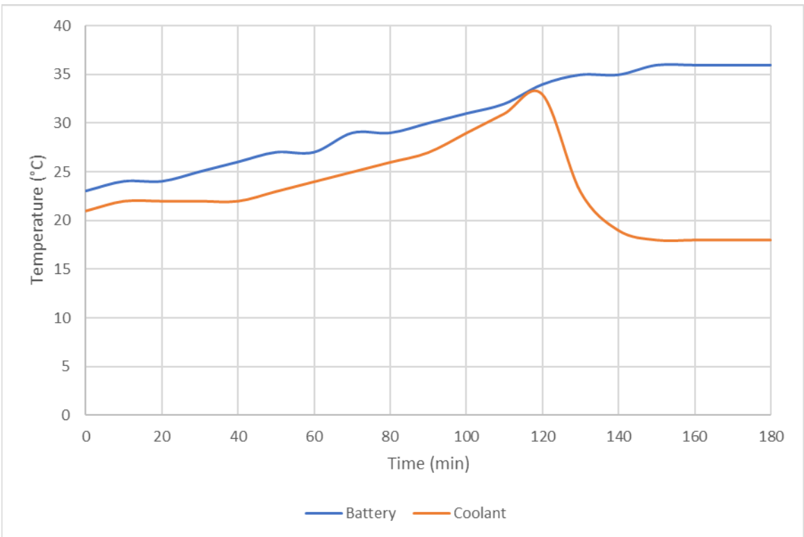
Figure 44: Over-Temperature Test Battery Temperature
