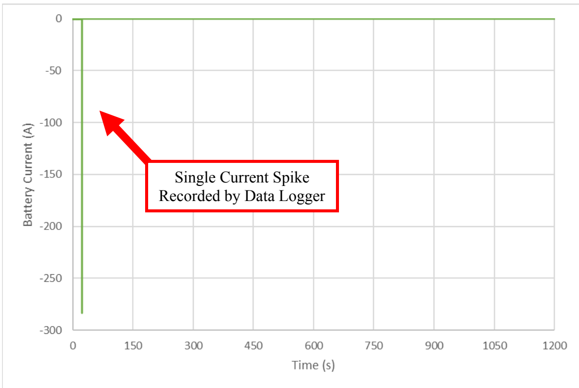
Figure 19: External Short Circuit Test Battery Current
