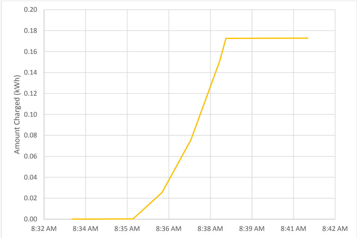
Figure 55: Over-Current Test Battery Tester Amount Charged
