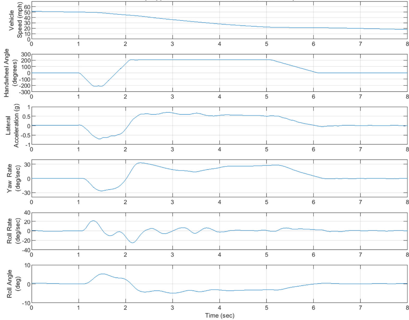
2020 MB Sprinter 2500 12P RWD, Date: 9/8/2020, MES = 50 mph, (Supplemental Test Series, Part 2, Test 0021)
