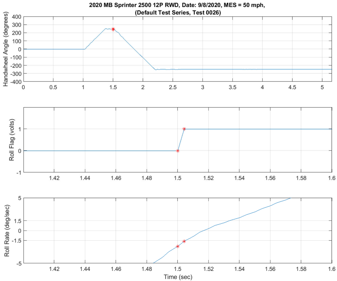
Figure D6. Steering Machine Operation Time History Plots for Default Test Series, R-L, 50 mph
