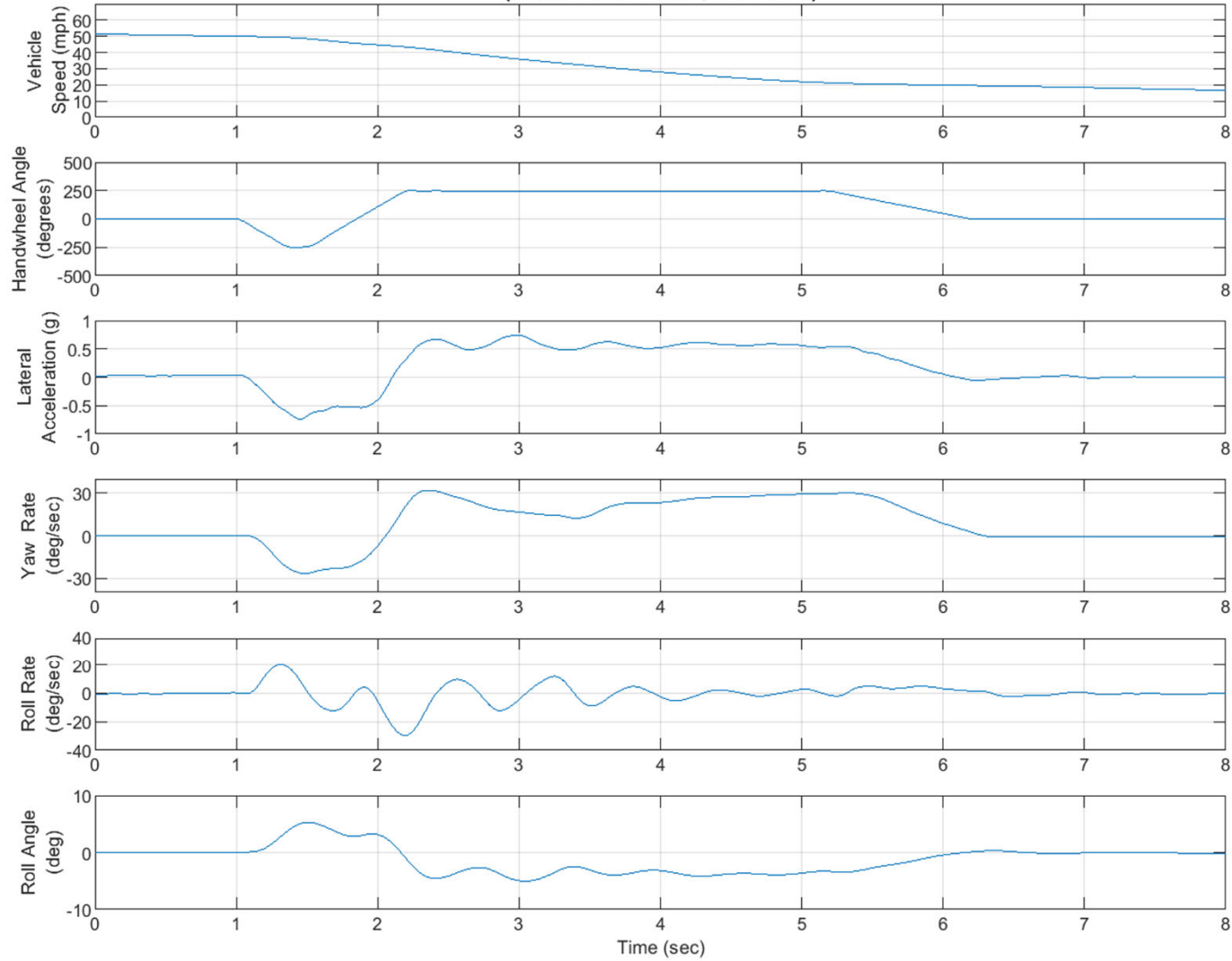
2020 MB Sprinter 2500 12P RWD, Date: 9/8/2020, MES = 50 mph, (Default Test Series, Test 0018)
