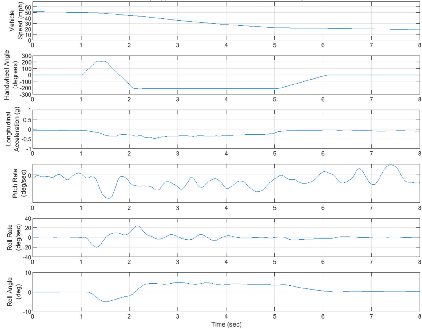
2020 MB Sprinter 2500 12P RWD, Date: 9/8/2020, MES = 50 mph, (Supplemental Test Series, Part 2, Test 0029)
