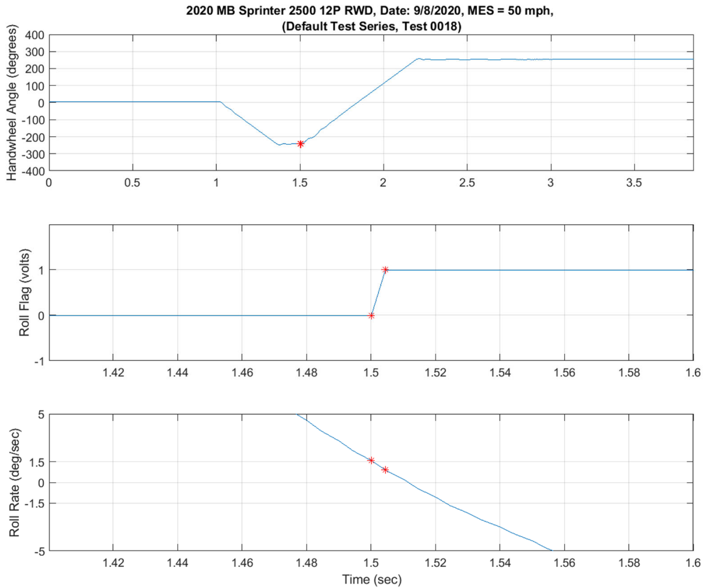
Figure D2. Steering Machine Operation Time History Plots for Default Test Series, L-R, 50 mph
