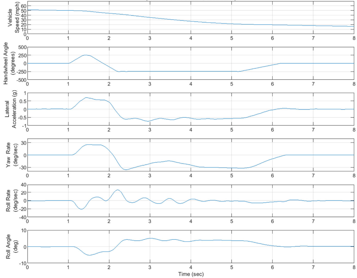
2020 MB Sprinter 2500 12P RWD, Date: 9/8/2020, MES = 50 mph, (Default Test Series, Test 0026)
