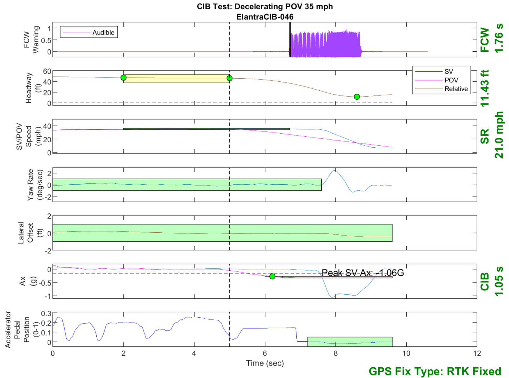
Figure D33. Time History for CIB Run 46, SV Encounters Decelerating POV, SV 35 mph, POV 35 mph
