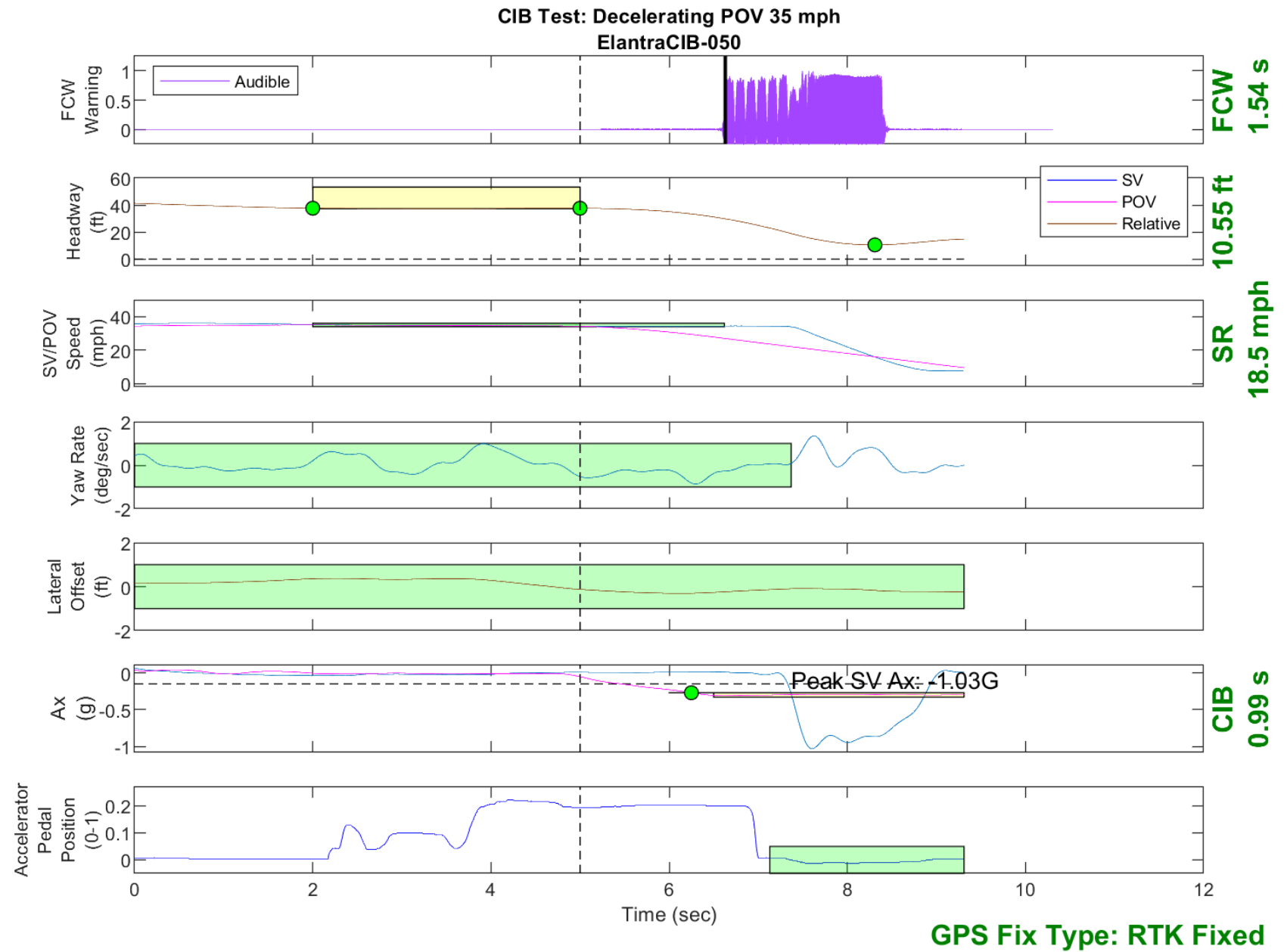
Figure D37. Time History for CIB Run 50, SV Encounters Decelerating POV, SV 35 mph, POV 35 mph
