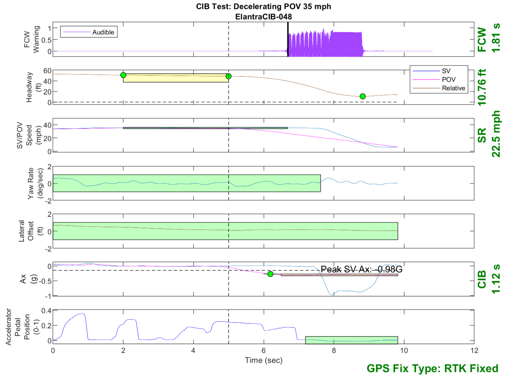
Figure D35. Time History for CIB Run 48, SV Encounters Decelerating POV, SV 35 mph, POV 35 mph
