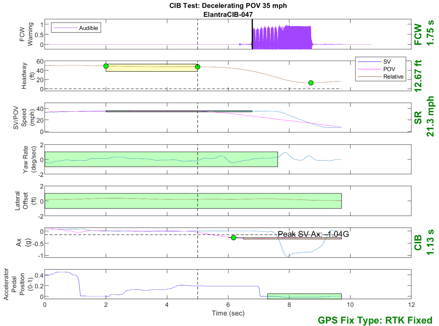
Figure D34. Time History for CIB Run 47, SV Encounters Decelerating POV, SV 35 mph, POV 35 mph
