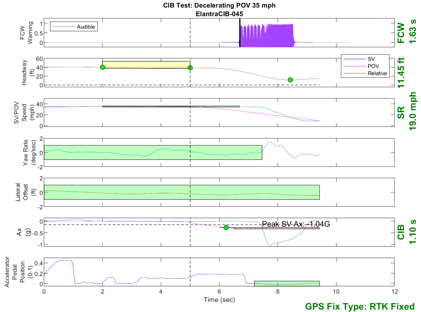
Figure D32. Time History for CIB Run 45, SV Encounters Decelerating POV, SV 35 mph, POV 35 mph
