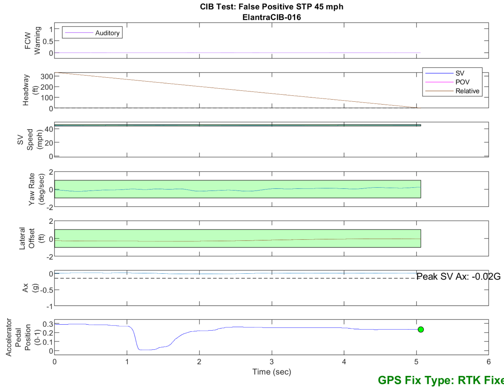
Figure D51. Time History for CIB Run 16, SV Encounters Steel Trench Plate, SV 45 mph
