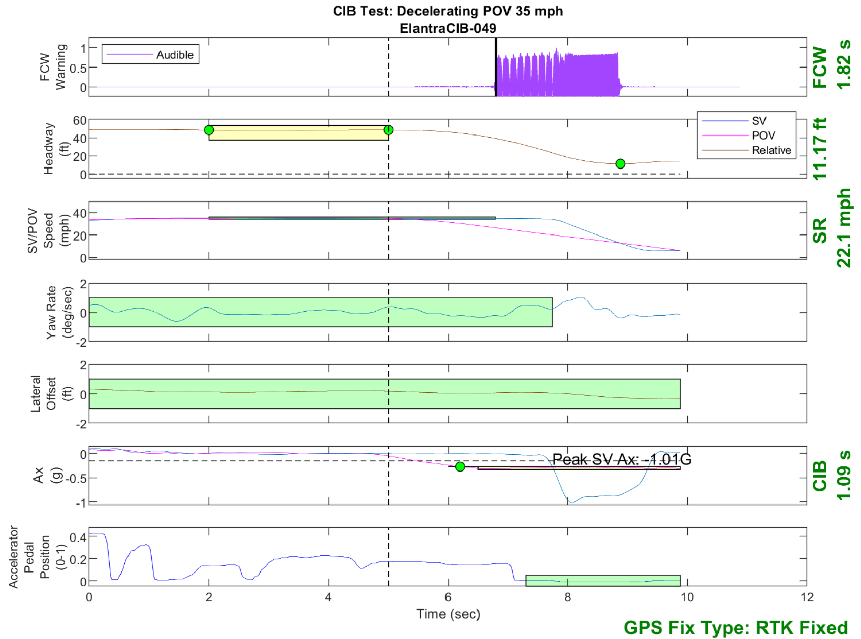
Figure D36. Time History for CIB Run 49, SV Encounters Decelerating POV, SV 35 mph, POV 35 mph
