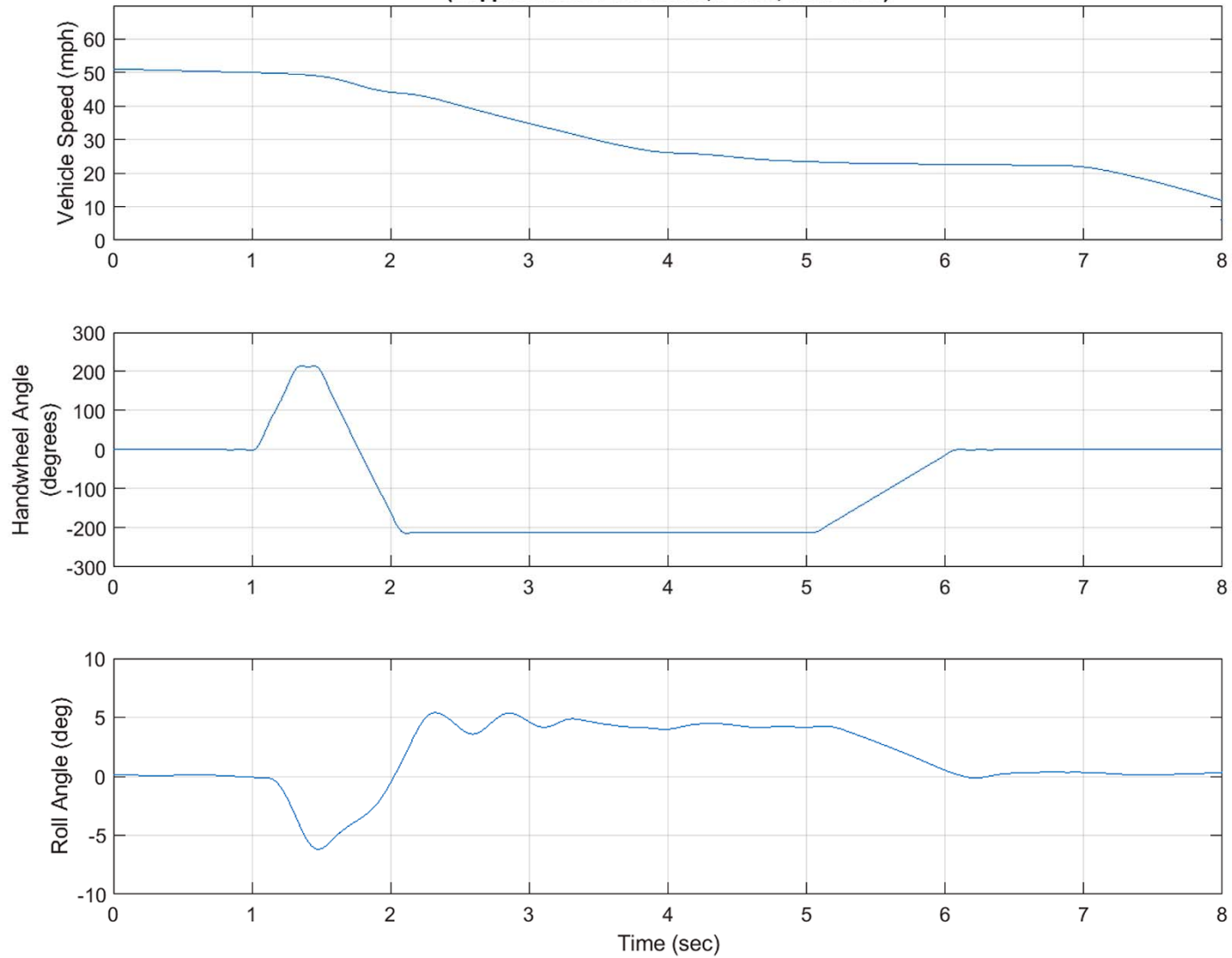
2020 Nissan Titan Crew Cab, Date: 04-21-2020, MES = 50 mph, (Supplemental Test Series, Part 2, Test 0029)
