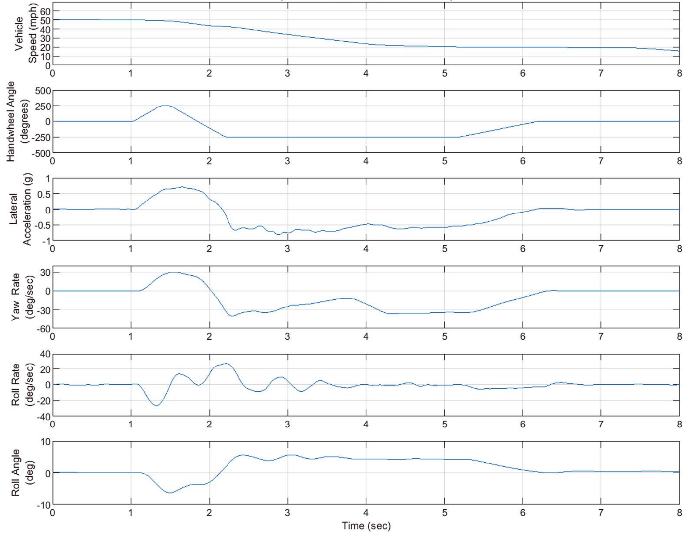
2020 Nissan Titan Crew Cab, Date: 04-21-2020, MES = 50 mph, (Default Test Series, Test 0026)
