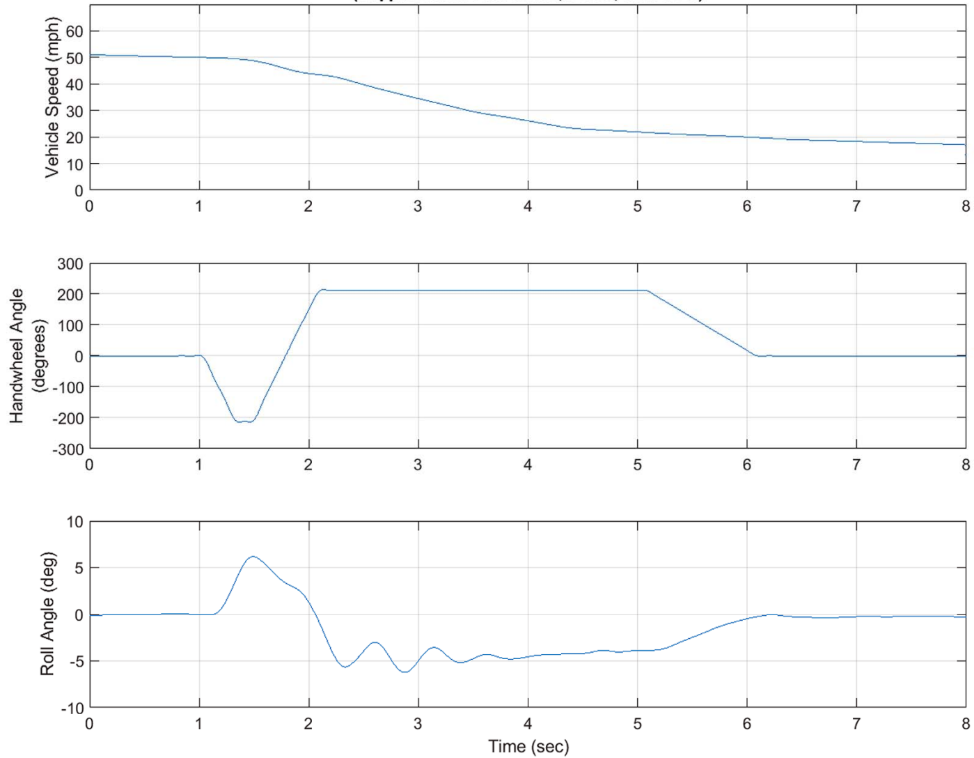
2020 Nissan Titan Crew Cab, Date: 04-21-2020, MES = 50 mph, (Supplemental Test Series, Part 2, Test 0021)
