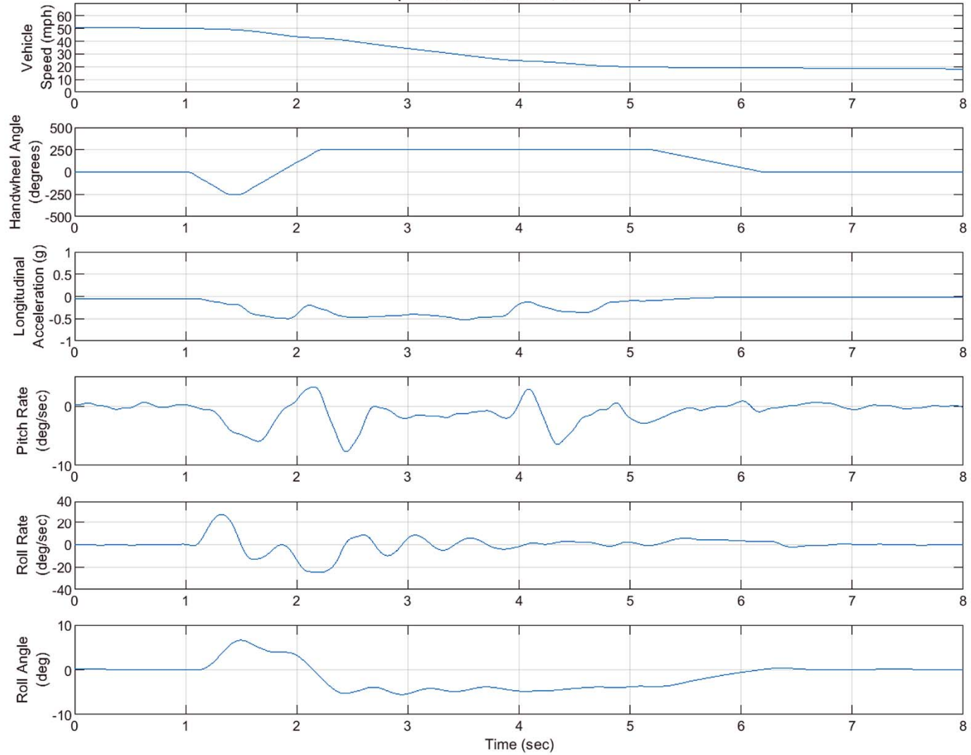
2020 Nissan Titan Crew Cab, Date: 04-21-2020, MES = 50 mph, (Default Test Series, Test 0018)
