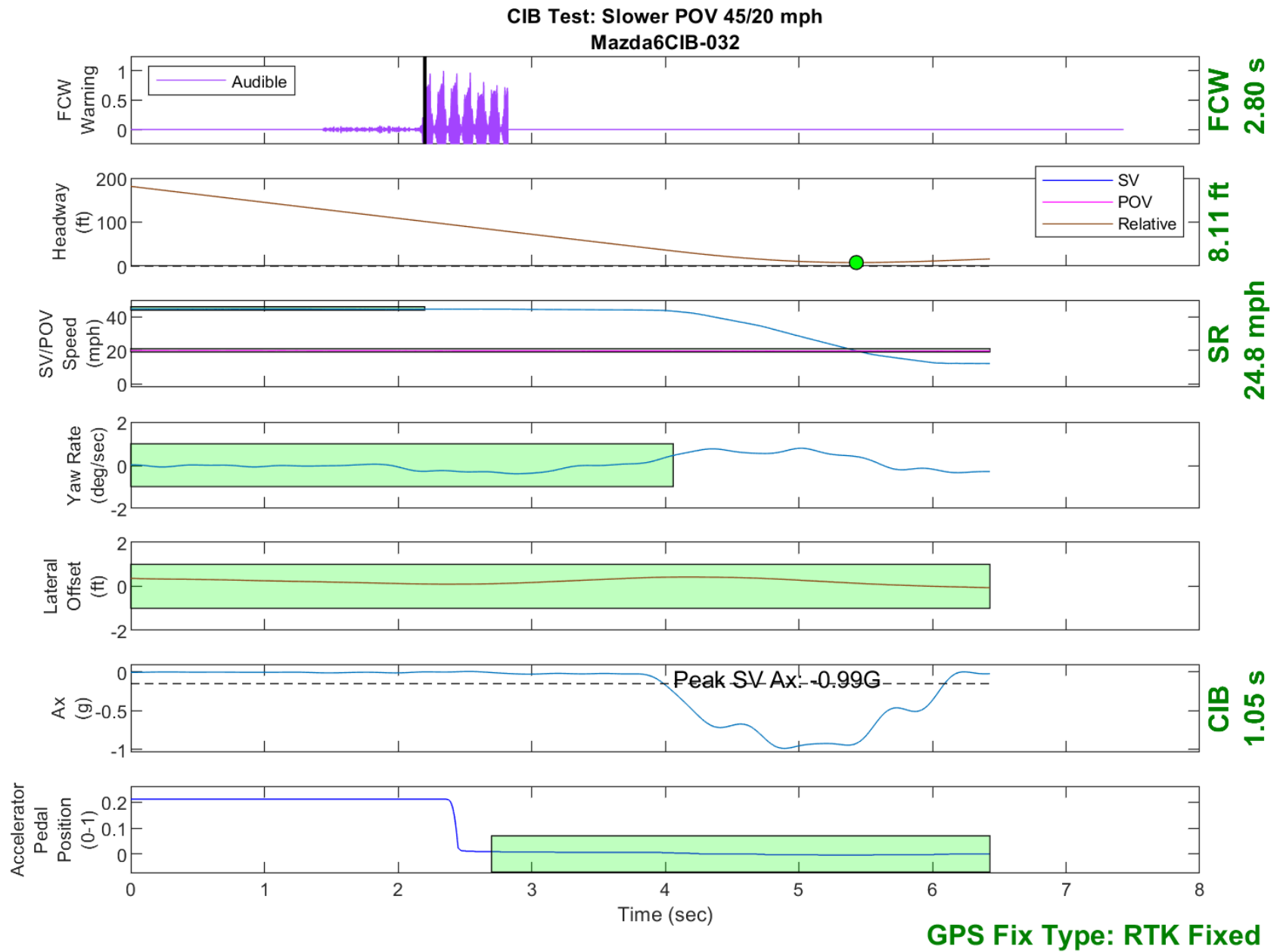
Figure D27. Time History for CIB Run 32, SV Encounters Slower POV, SV 45 mph, POV 20 mph
