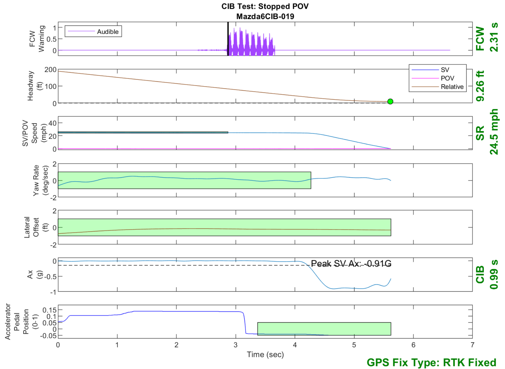
Figure D16. Time History for CIB Run 19, SV Encounters Stopped POV
