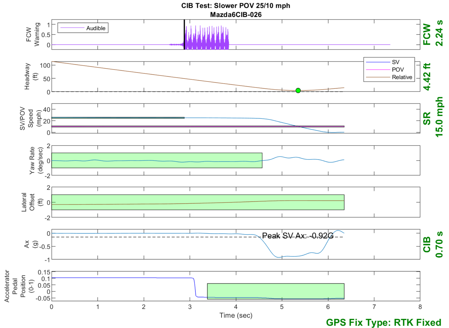
Figure D22. Time History for CIB Run 26, SV Encounters Slower POV, SV 25 mph, POV 10 mph
