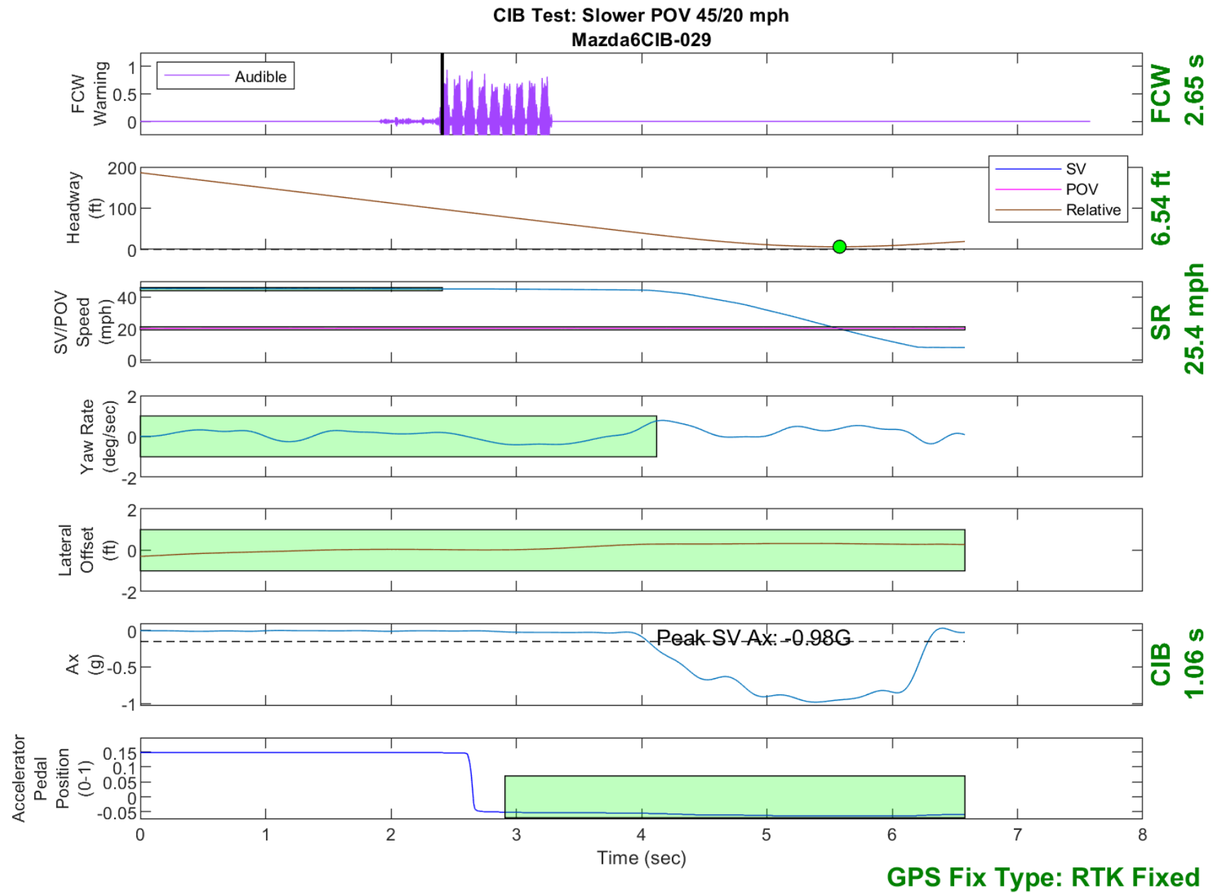
Figure D24. Time History for CIB Run 29, SV Encounters Slower POV, SV 45 mph, POV 20 mph
