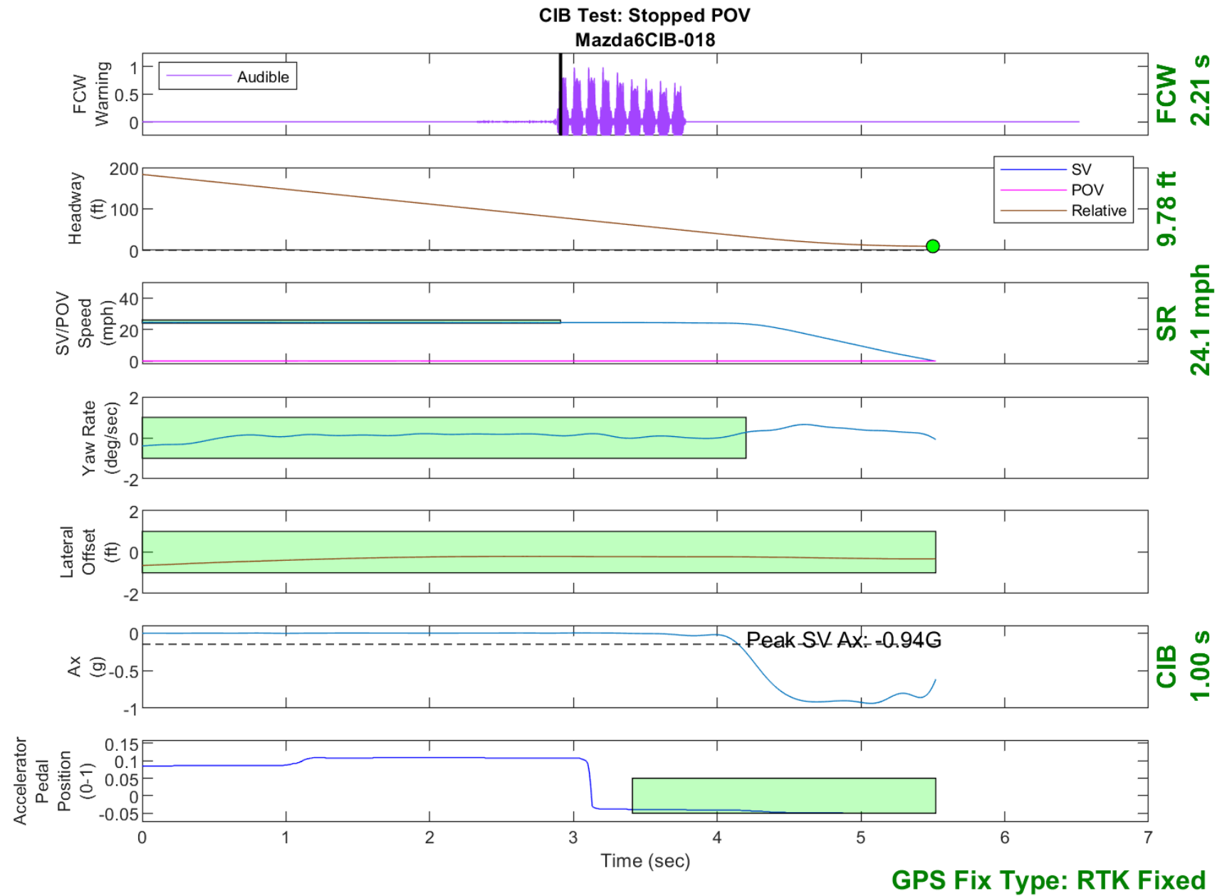
Figure D15. Time History for CIB Run 18, SV Encounters Stopped POV
