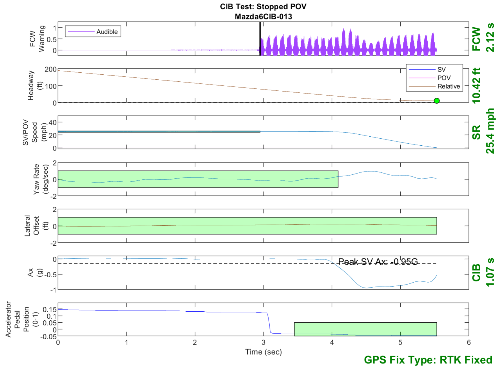
Figure D10. Time History for CIB Run 13, SV Encounters Stopped POV
