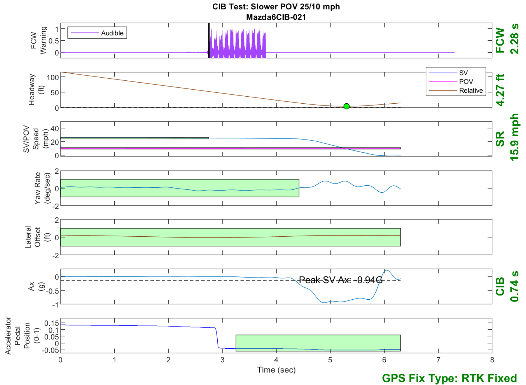
Figure D17. Time History for CIB Run 21, SV Encounters Slower POV, SV 25 mph, POV 10 mph
