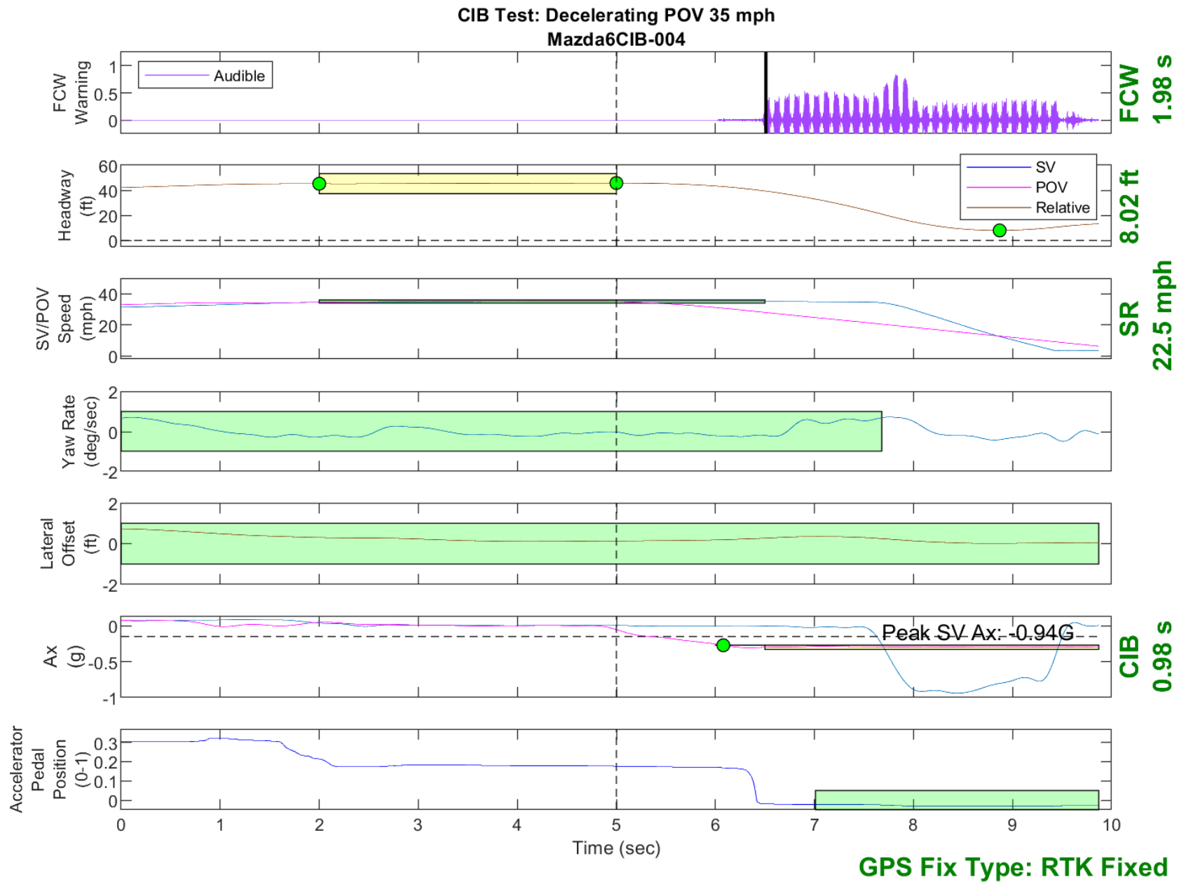
Figure D31. Time History for CIB Run 4, SV Encounters Decelerating POV, SV 35 mph, POV 35 mph
