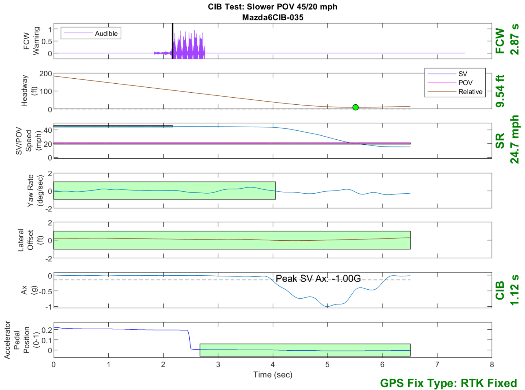
Figure D30. Time History for CIB Run 35, SV Encounters Slower POV, SV 45 mph, POV 20 mph
