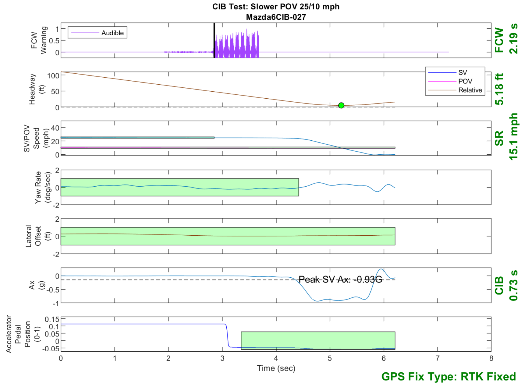
Figure D23. Time History for CIB Run 27, SV Encounters Slower POV, SV 25 mph, POV 10 mph
