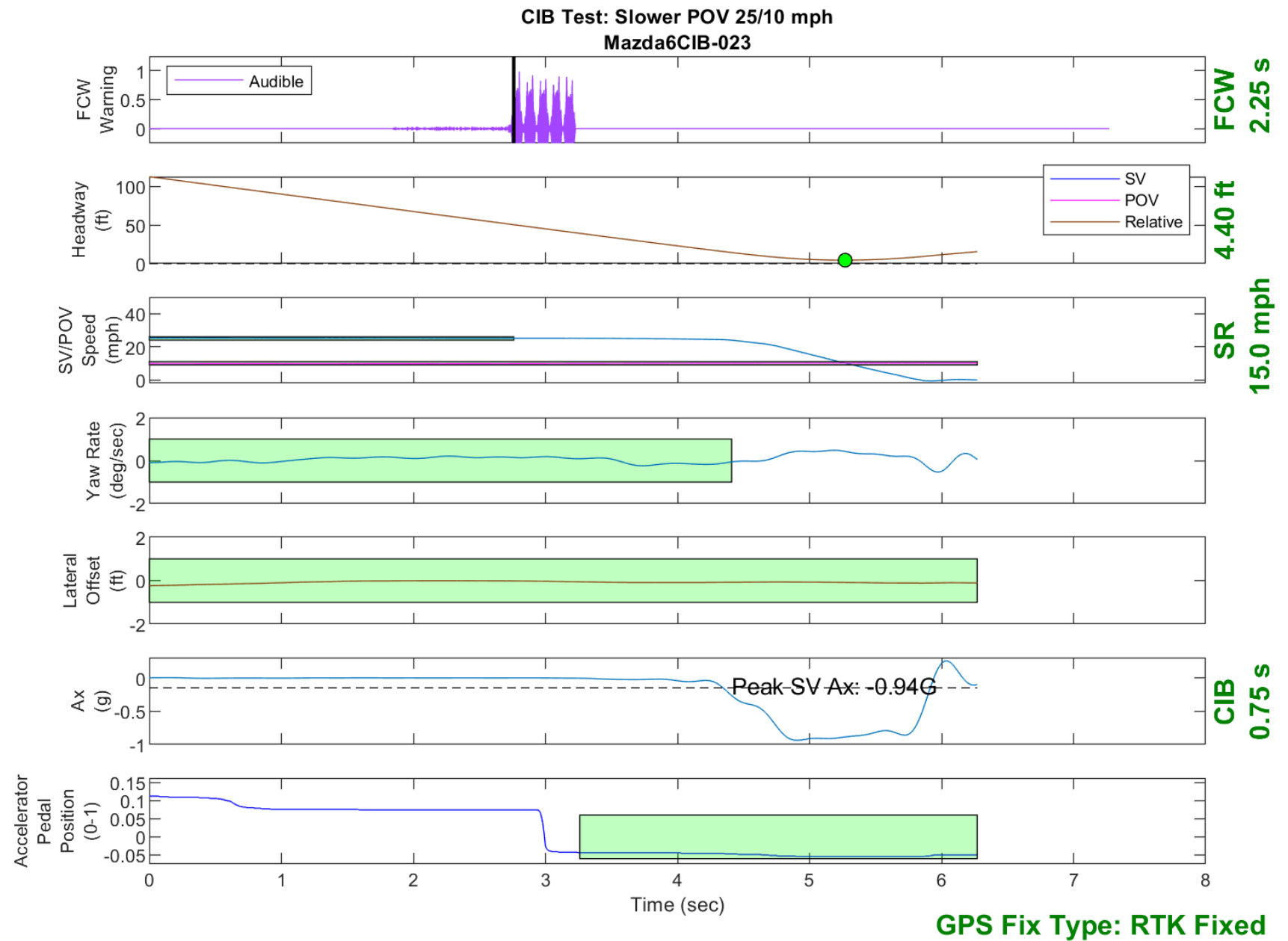
Figure D19. Time History for CIB Run 23, SV Encounters Slower POV, SV 25 mph, POV 10 mph
