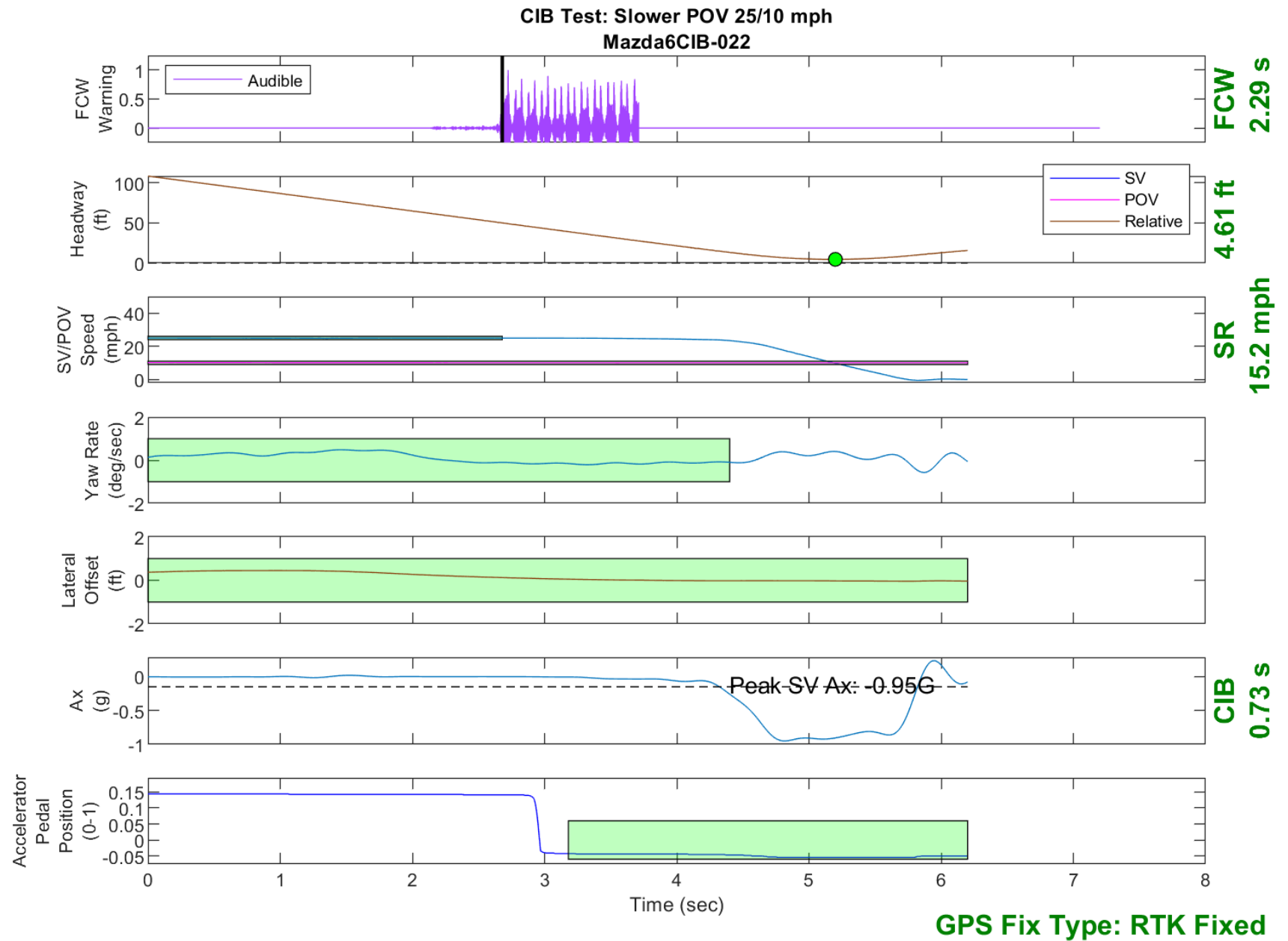
Figure D18. Time History for CIB Run 22, SV Encounters Slower POV, SV 25 mph, POV 10 mph
