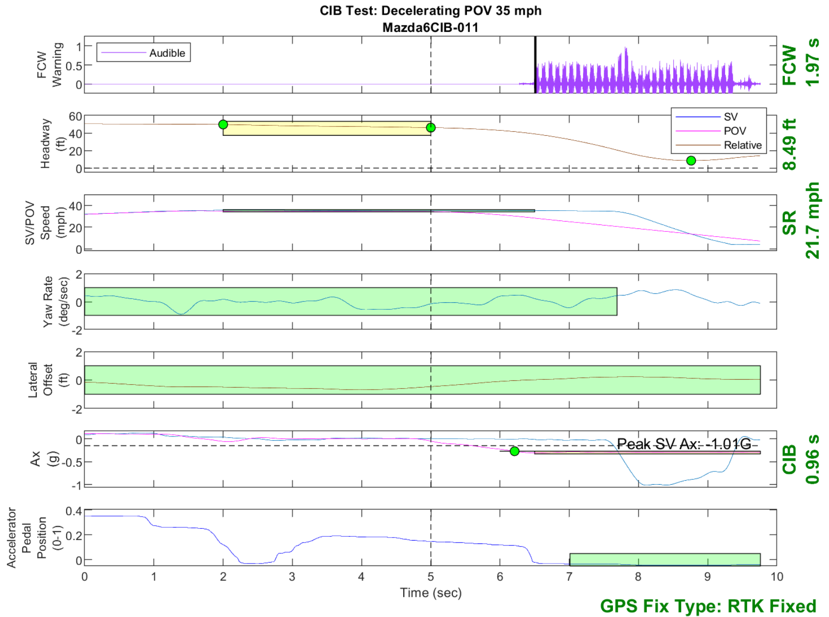
Figure D37. Time History for CIB Run 11, SV Encounters Decelerating POV, SV 35 mph, POV 35 mph
