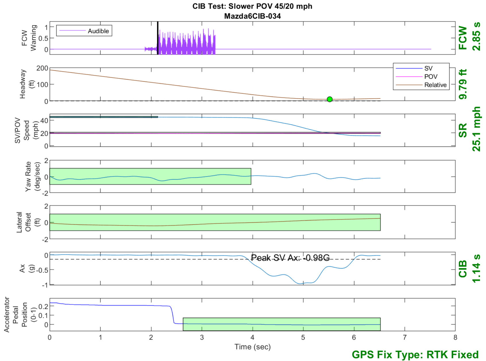
Figure D29. Time History for CIB Run 34, SV Encounters Slower POV, SV 45 mph, POV 20 mph
