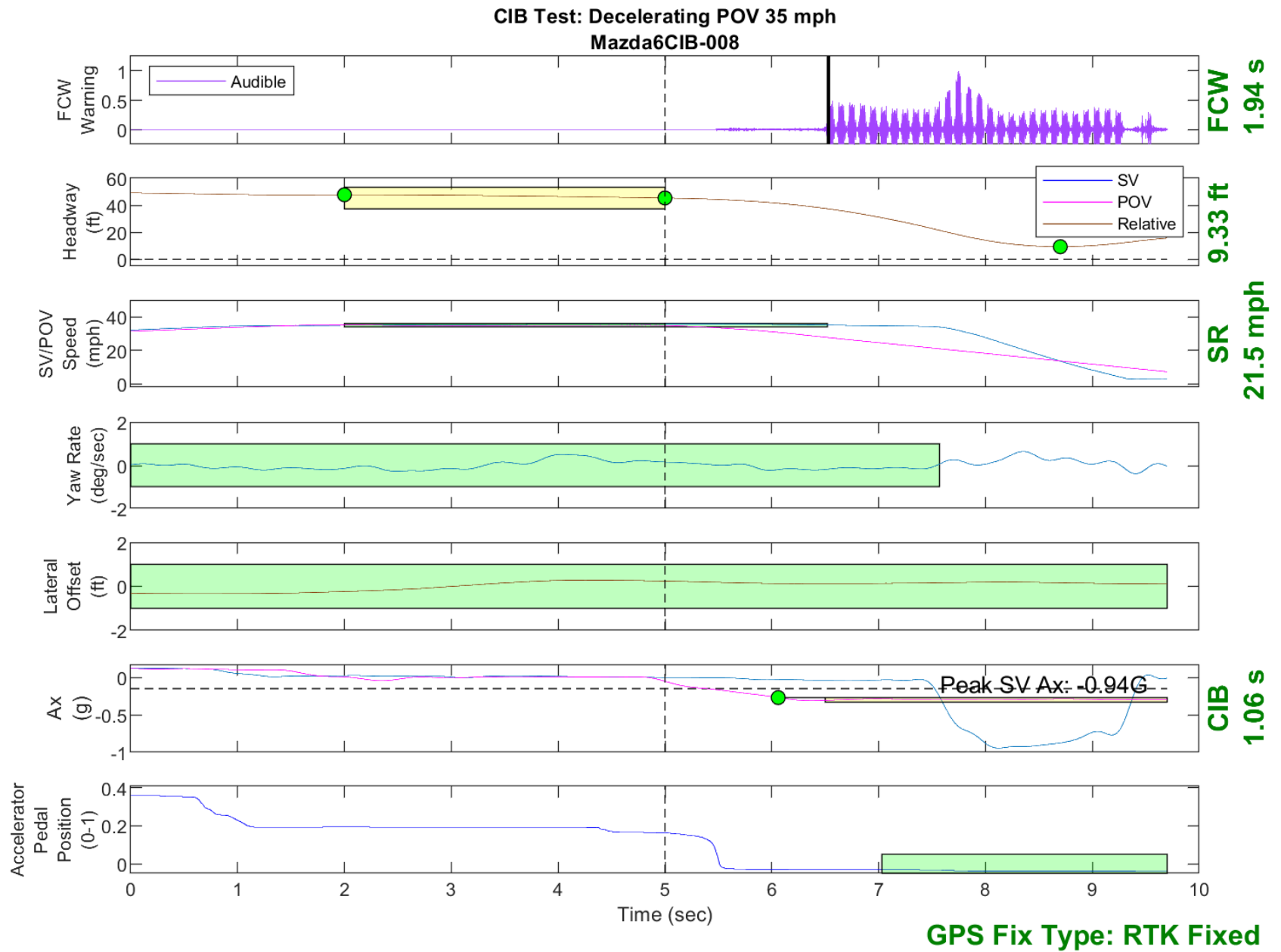
Figure D34. Time History for CIB Run 8, SV Encounters Decelerating POV, SV 35 mph, POV 35 mph
