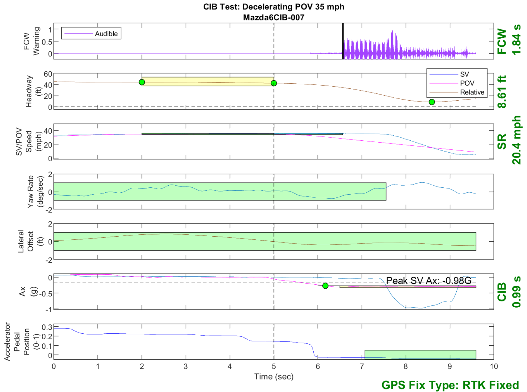
Figure D33. Time History for CIB Run 7, SV Encounters Decelerating POV, SV 35 mph, POV 35 mph
