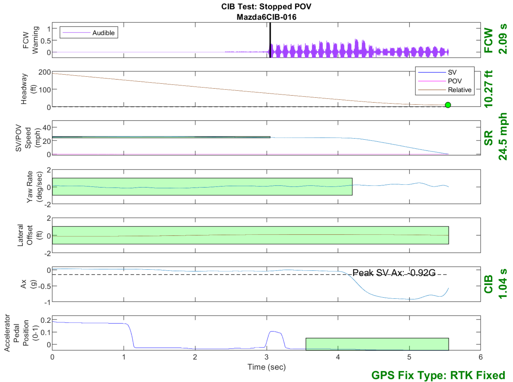
Figure D13. Time History for CIB Run 16, SV Encounters Stopped POV
