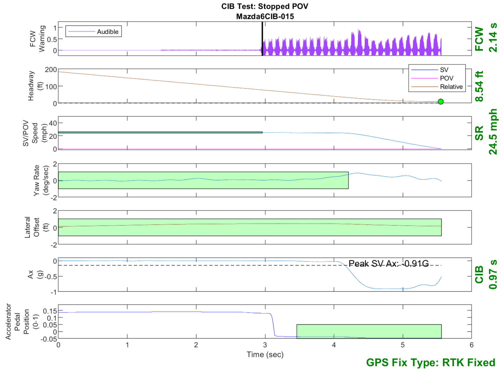
Figure D12. Time History for CIB Run 15, SV Encounters Stopped POV
