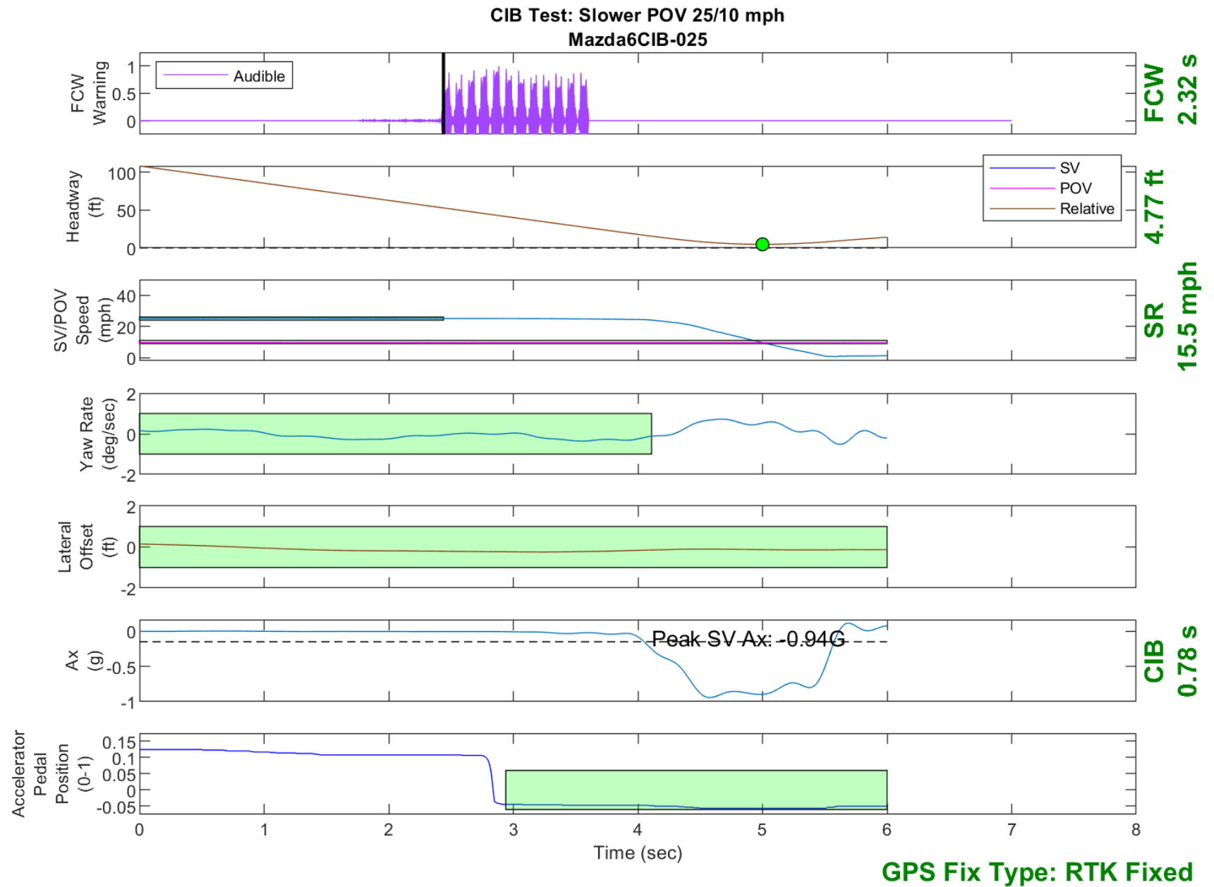
Figure D21. Time History for CIB Run 25, SV Encounters Slower POV, SV 25 mph, POV 10 mph
