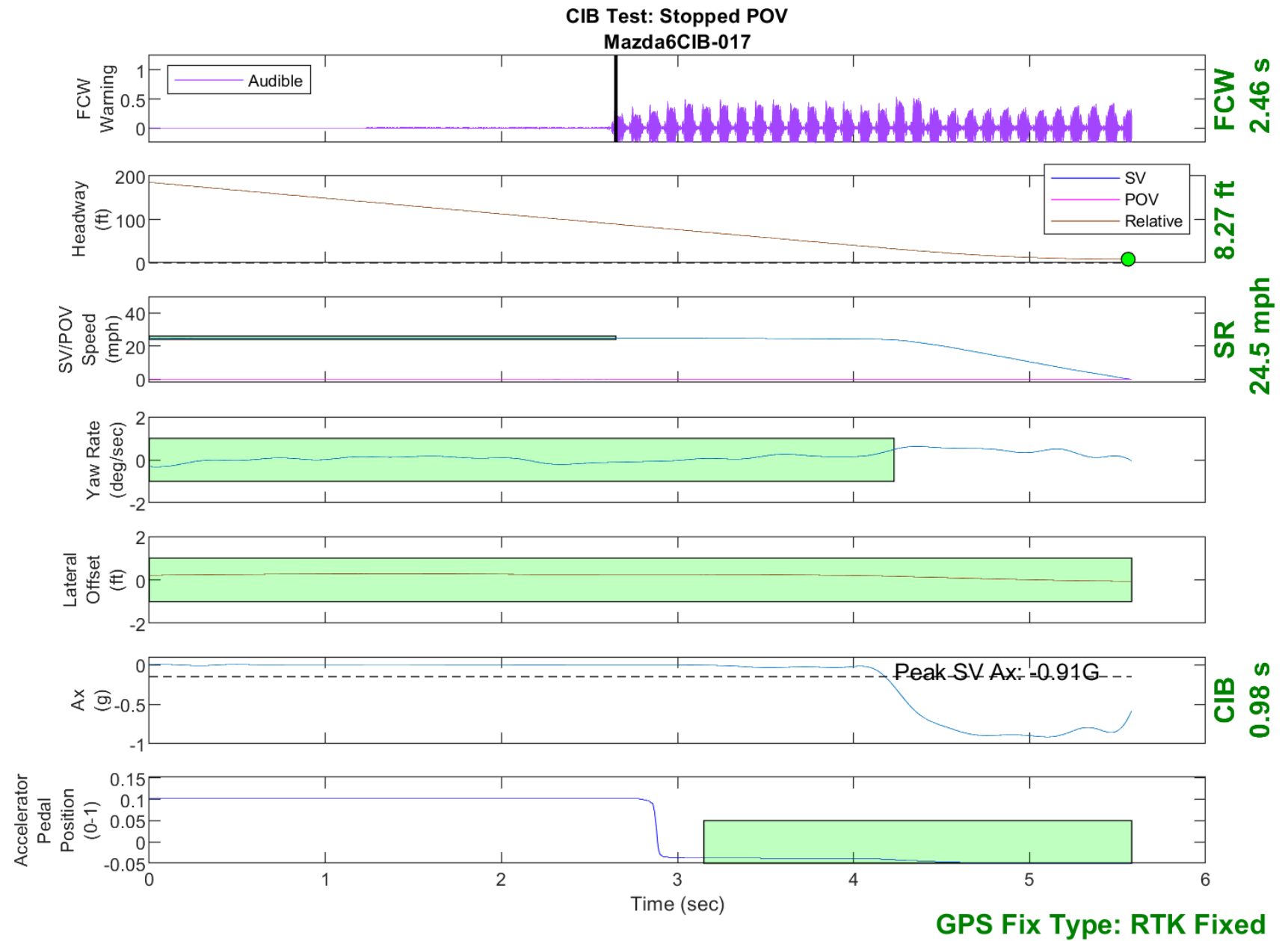
Figure D14. Time History for CIB Run 17, SV Encounters Stopped POV
