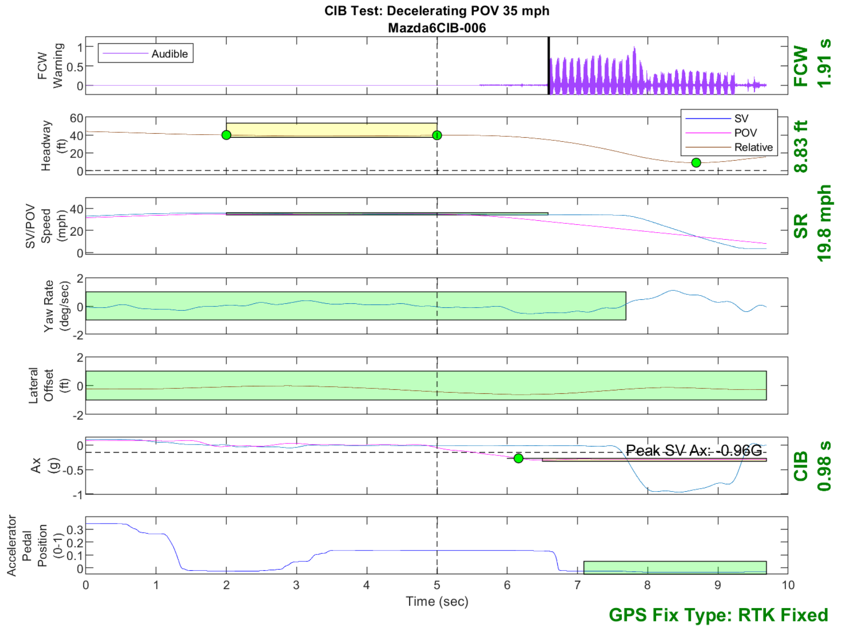
Figure D32. Time History for CIB Run 6, SV Encounters Decelerating POV, SV 35 mph, POV 35 mph
