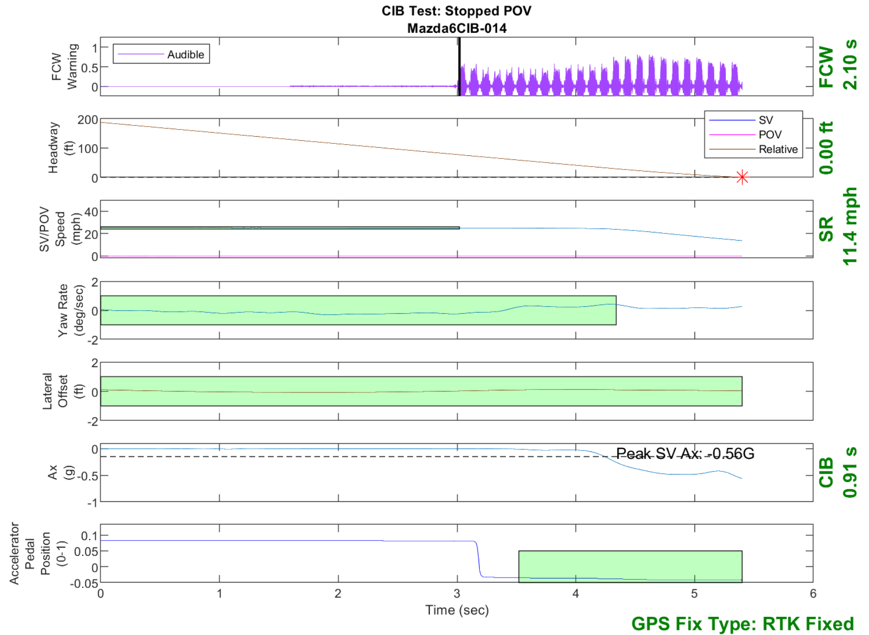
Figure D11. Time History for CIB Run 14, SV Encounters Stopped POV
