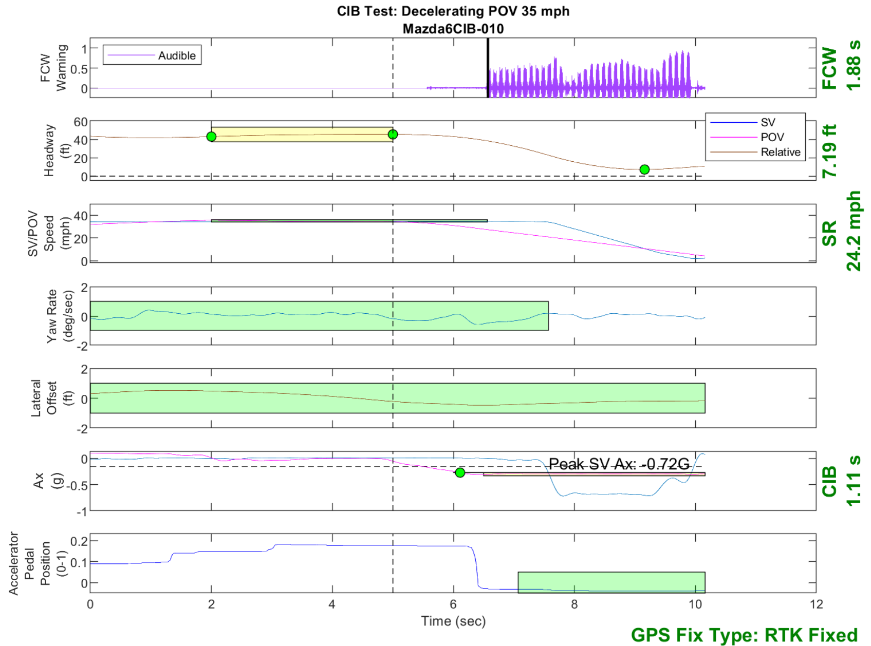
Figure D36. Time History for CIB Run 10, SV Encounters Decelerating POV, SV 35 mph, POV 35 mph
