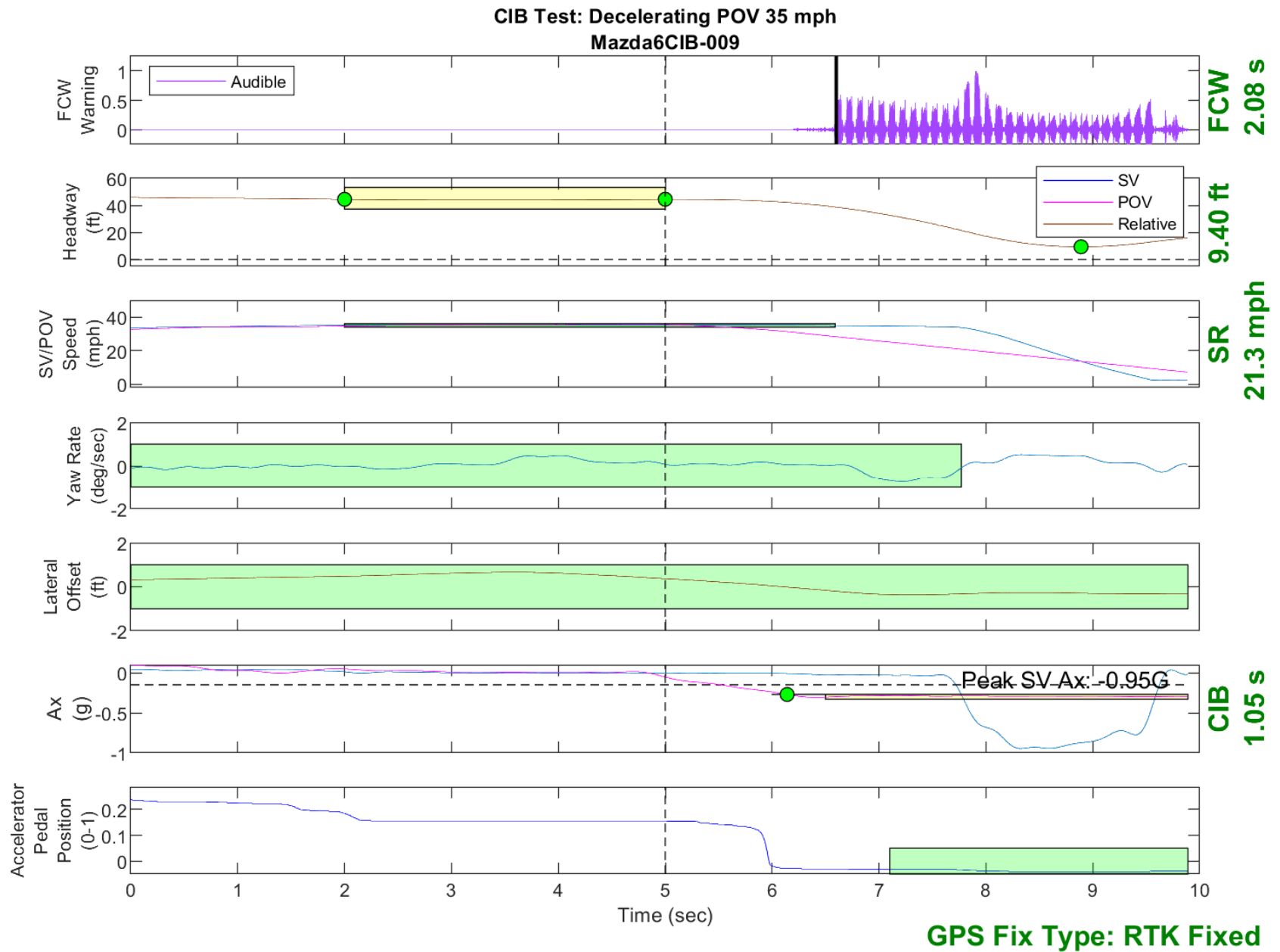
Figure D35. Time History for CIB Run 9, SV Encounters Decelerating POV, SV 35 mph, POV 35 mph
