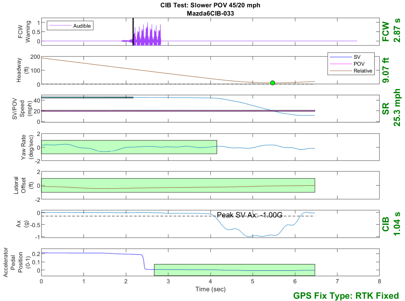
Figure D28. Time History for CIB Run 33, SV Encounters Slower POV, SV 45 mph, POV 20 mph
