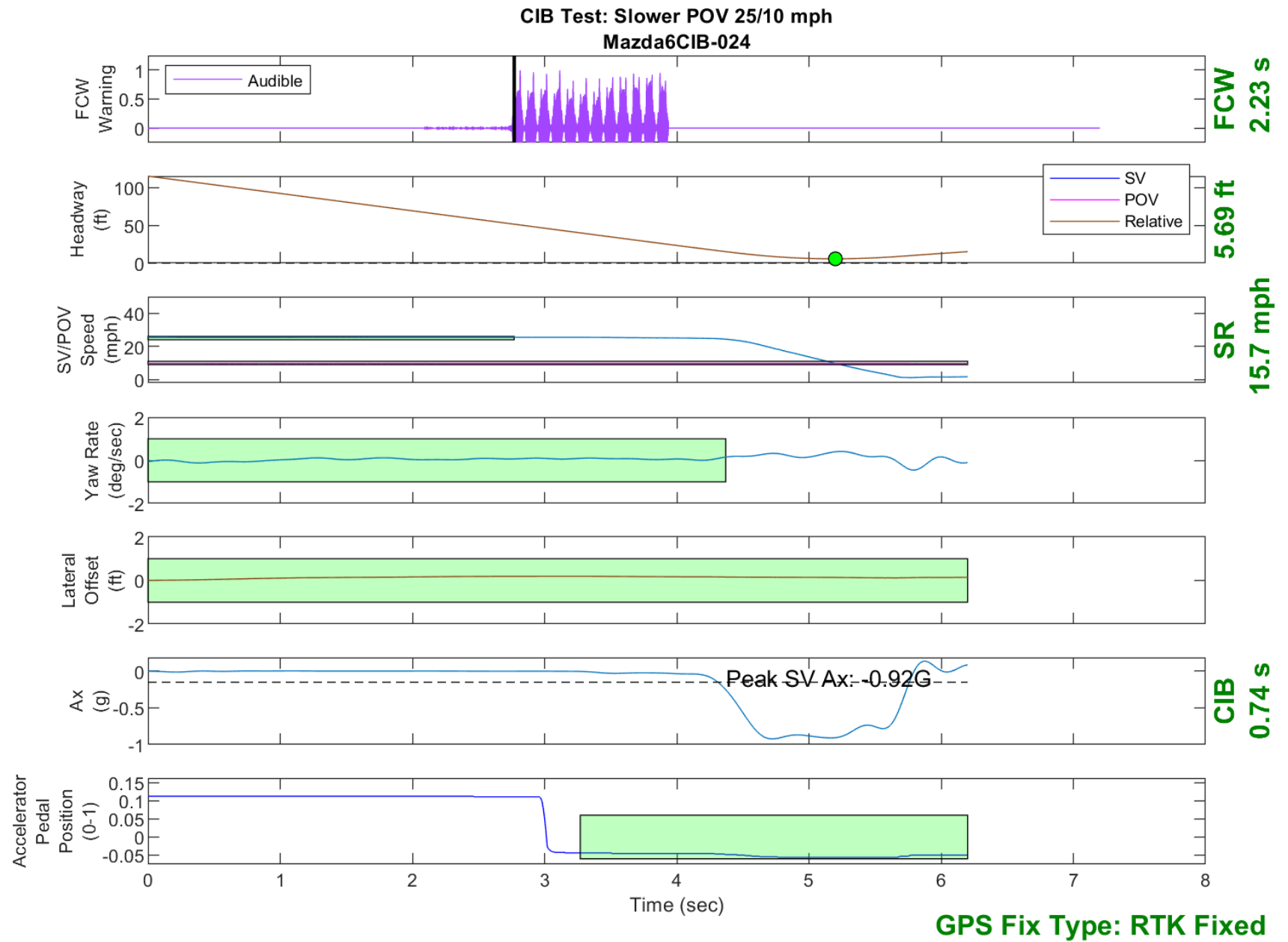
Figure D20. Time History for CIB Run 24, SV Encounters Slower POV, SV 25 mph, POV 10 mph
