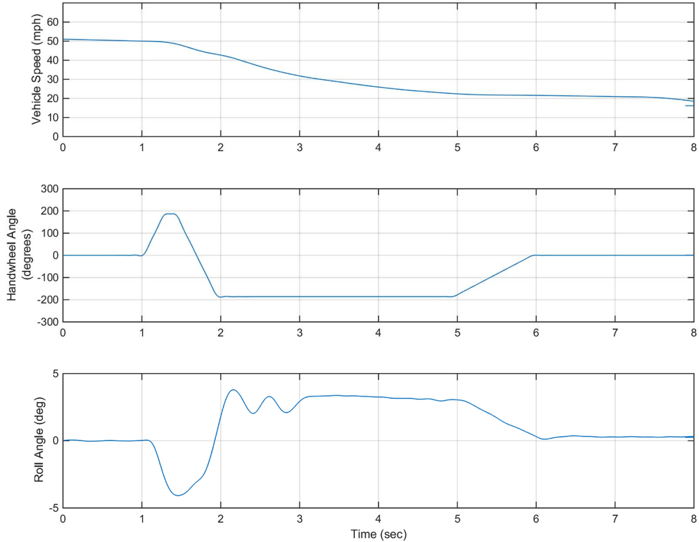
2020 Volkswagen Atlas Cross Sport, Date: 3/26/2020, MES = 50 mph, (Default Test Series, Test 0026)
