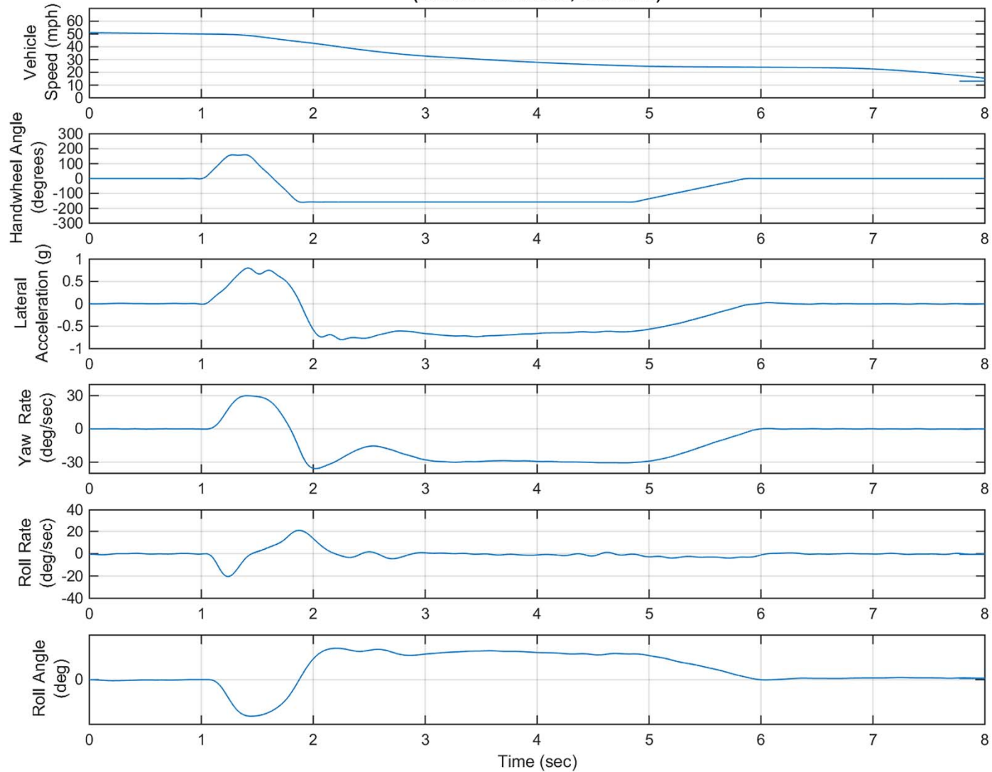
2020 Volkswagen Atlas Cross Sport, Date: 3/26/2020, MES = 50 mph, (Default Test Series, Test 0029)
