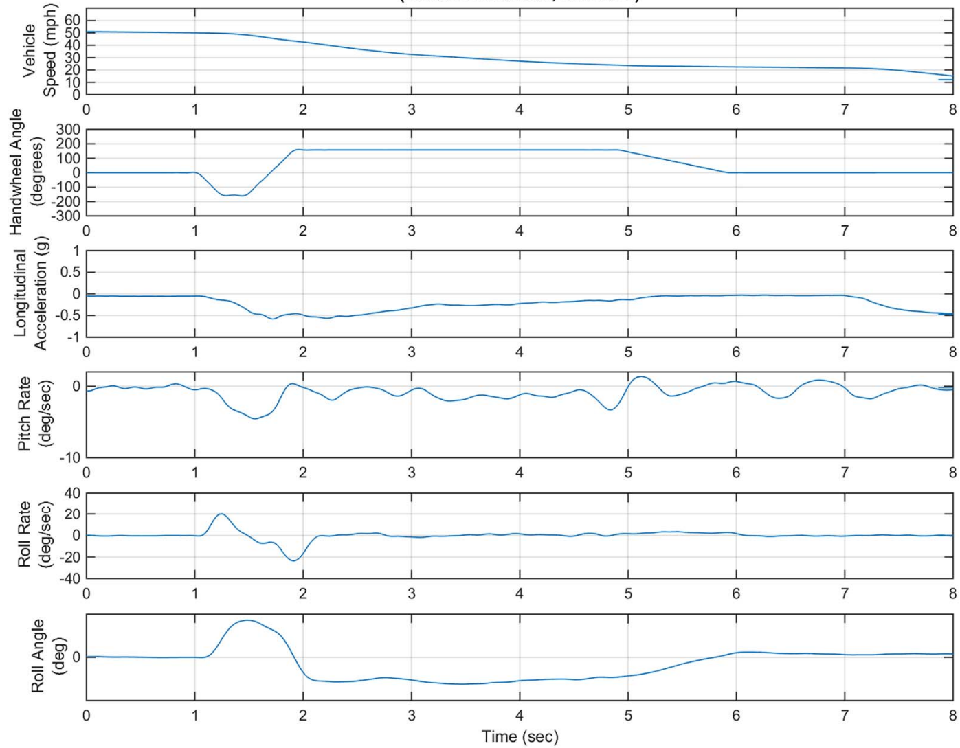
2020 Volkswagen Atlas Cross Sport, Date: 3/26/2020, MES = 50 mph, (Default Test Series, Test 0021)
