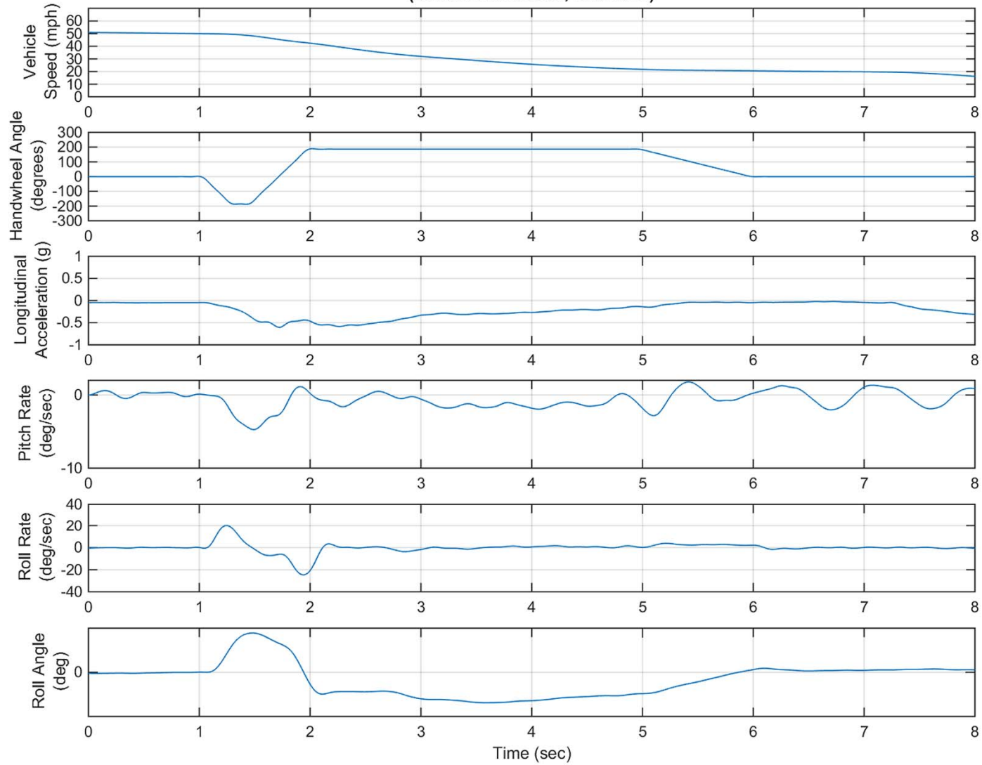
2020 Volkswagen Atlas Cross Sport, Date: 3/26/2020, MES = 50 mph, (Default Test Series, Test 0018)
