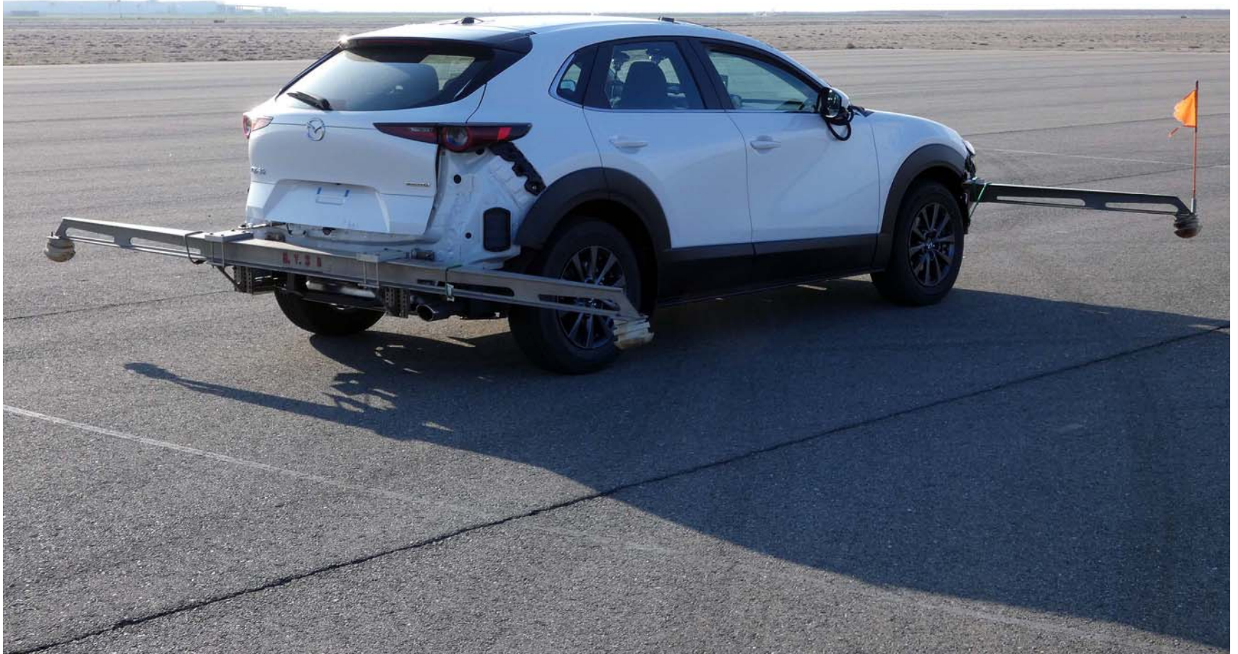
Figure A5. Rear View, Test Vehicle in Test Condition
