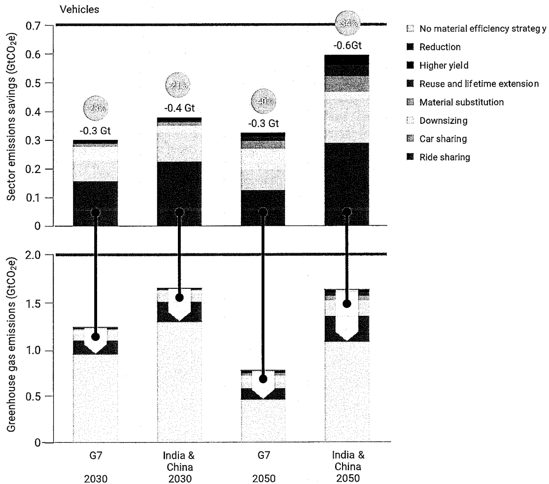
Figure 7.3. Annual emissions from the manufacturing and use of passenger vehicles in the G7 and in China and India, in a scenario that follows the Shared Socioeconomic Pathway SSP1 to mitigate emissions to below 2°C
