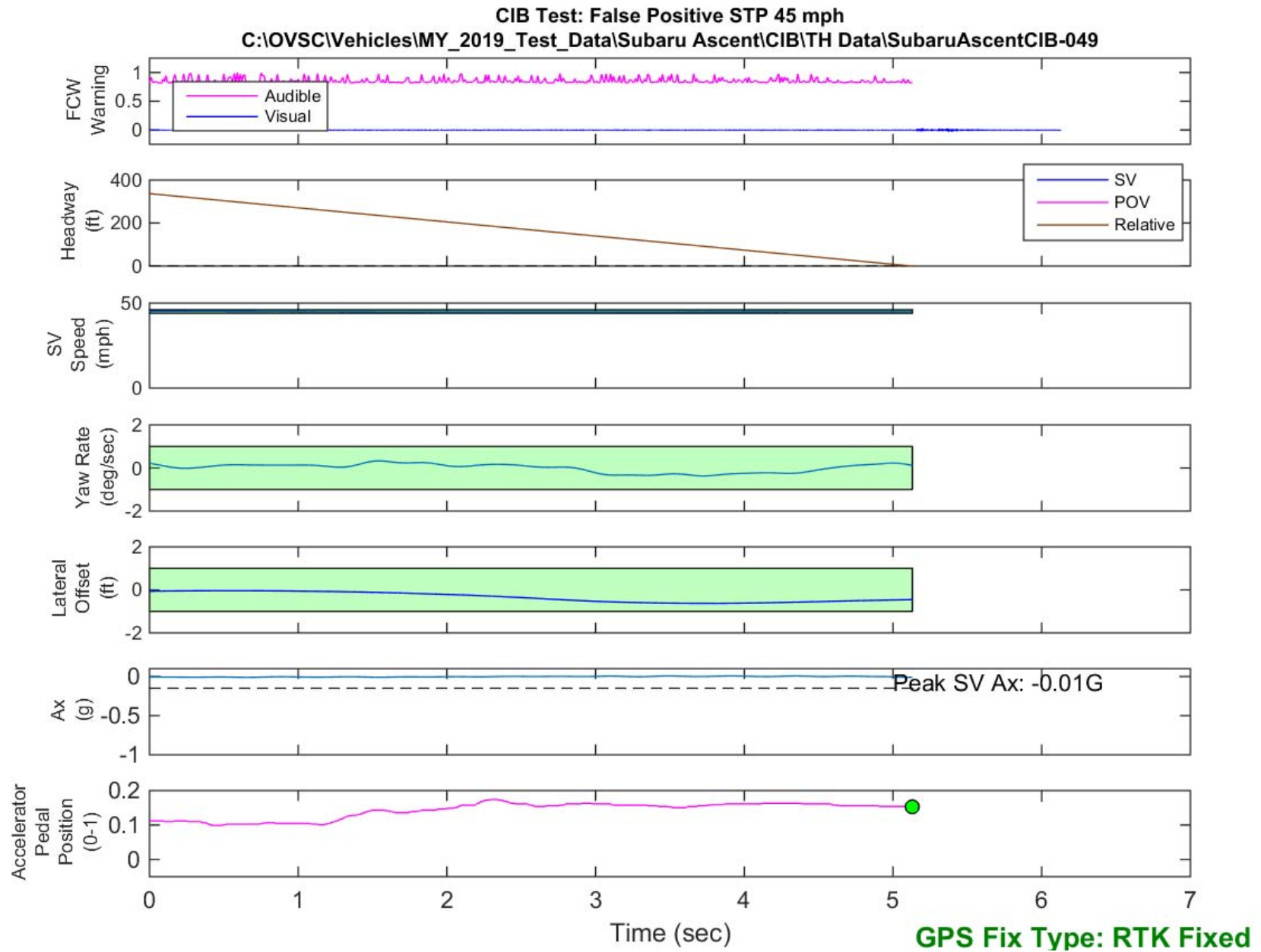
Figure D46. Time History for CIB Run 49, SV Encounters Steel Trench Plate, SV 45 mph
