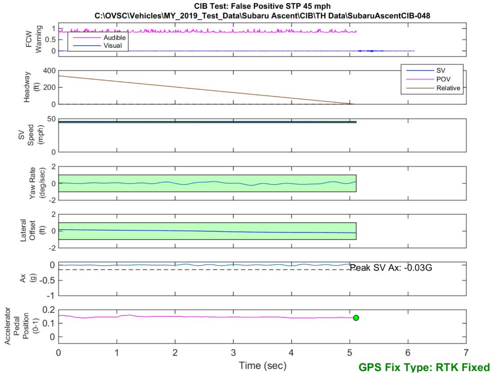
Figure D45. Time History for CIB Run 48, SV Encounters Steel Trench Plate, SV 45 mph
