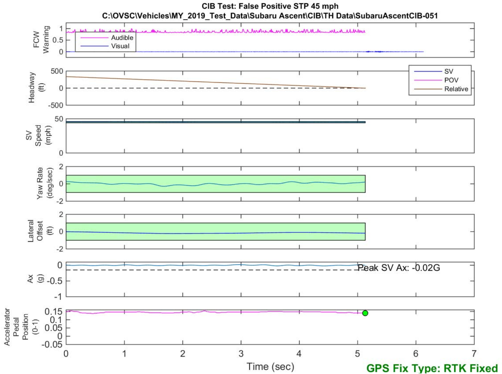
Figure D48. Time History for CIB Run 51, SV Encounters Steel Trench Plate, SV 45 mph
