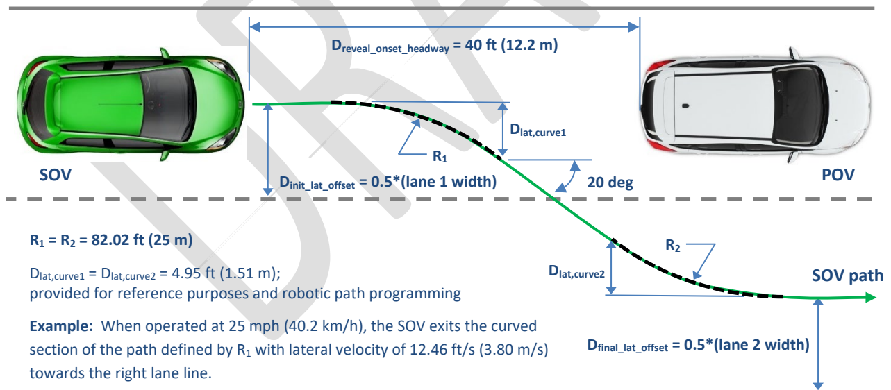
Figure 4. SOV lane change path used during the SRSV scenario.
