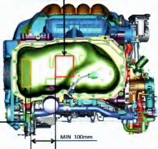
VIEW a
