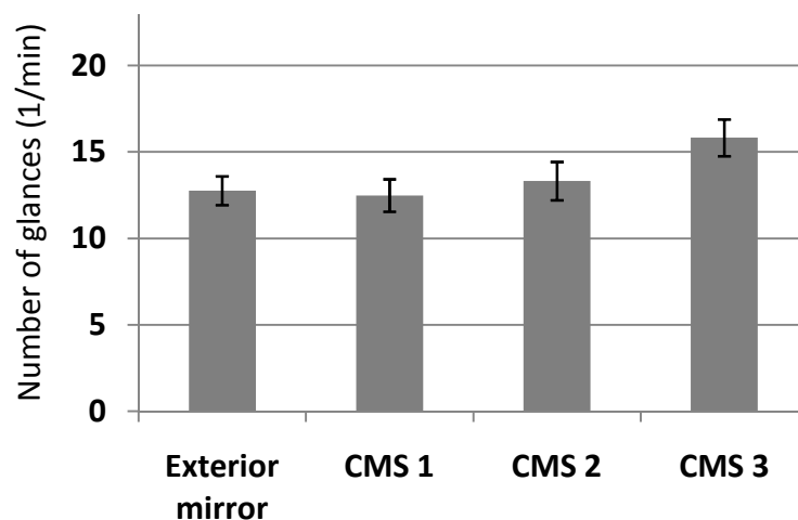
Figure 65: Number of glances per minute during overtaking, for different monitor/mirror positions.
