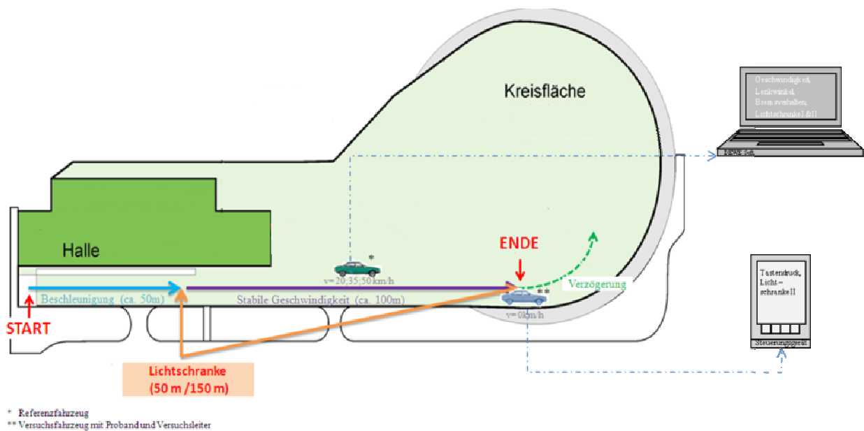
Figure 58: Schematic test set-up for distance and speed estimation of an approaching object vehicle at the test facilities of BAST
