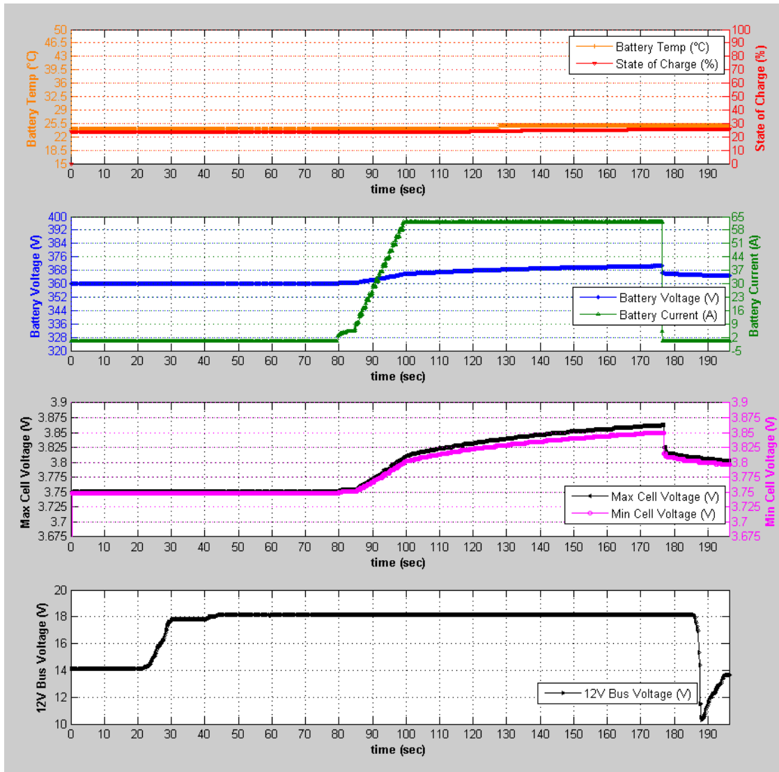
Figure 54: 12V System Over-Voltage Charge Data
