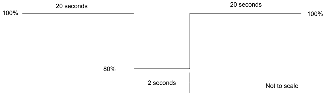
Figure 22: Voltage Sag
