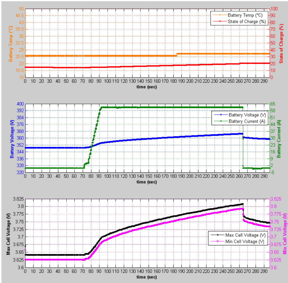
Figure 59: Charge Operation Disturbance Charge Data
