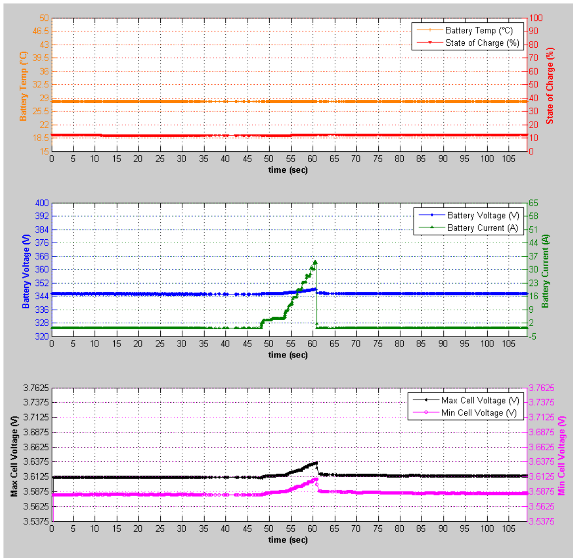
Figure 46: 47 \Omega During Charge Session Charge Data
