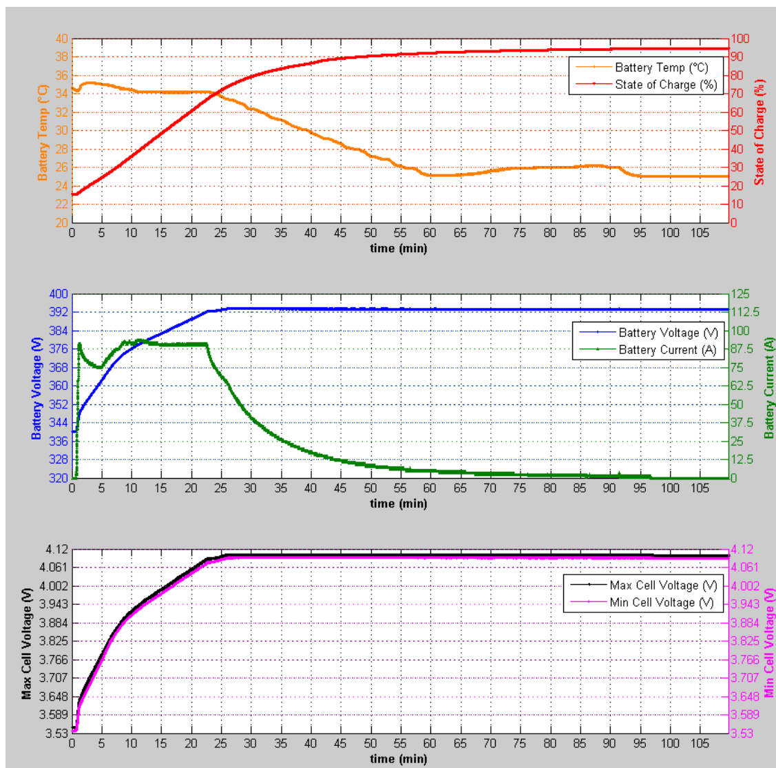
Figure 71: High Ambient Temperature (Coolant) Charge Data
