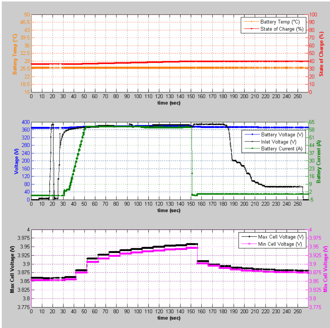
Figure 53: During Charge Session Charge Data
