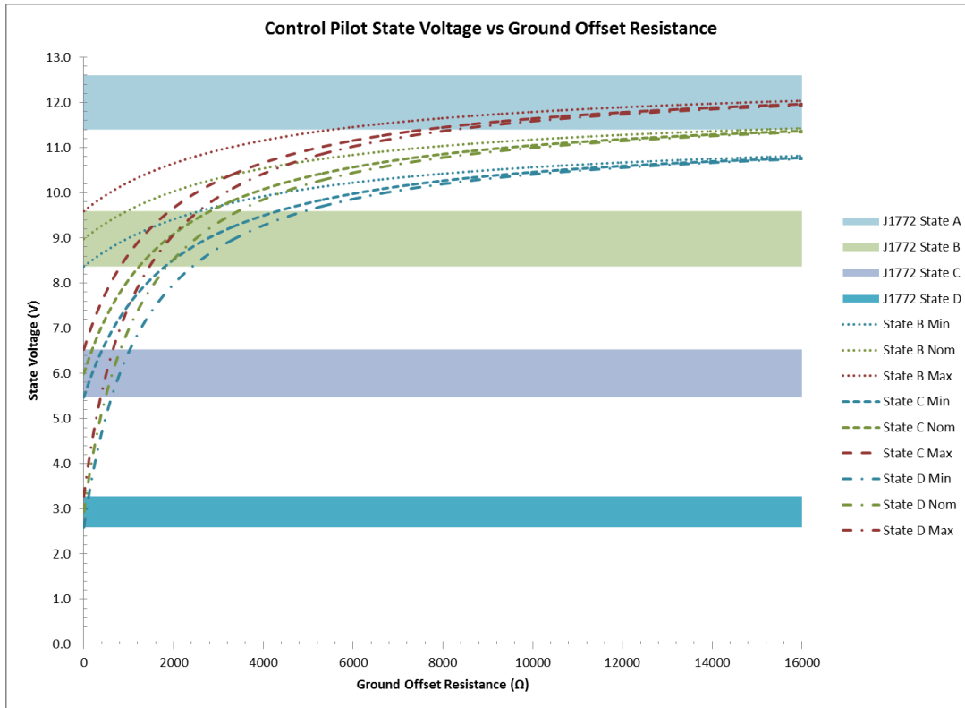
Figure 36: SAE J1772 Control Pilot State Voltage Versus Ground Offset Resistance (0 - 16 k \Omega )
