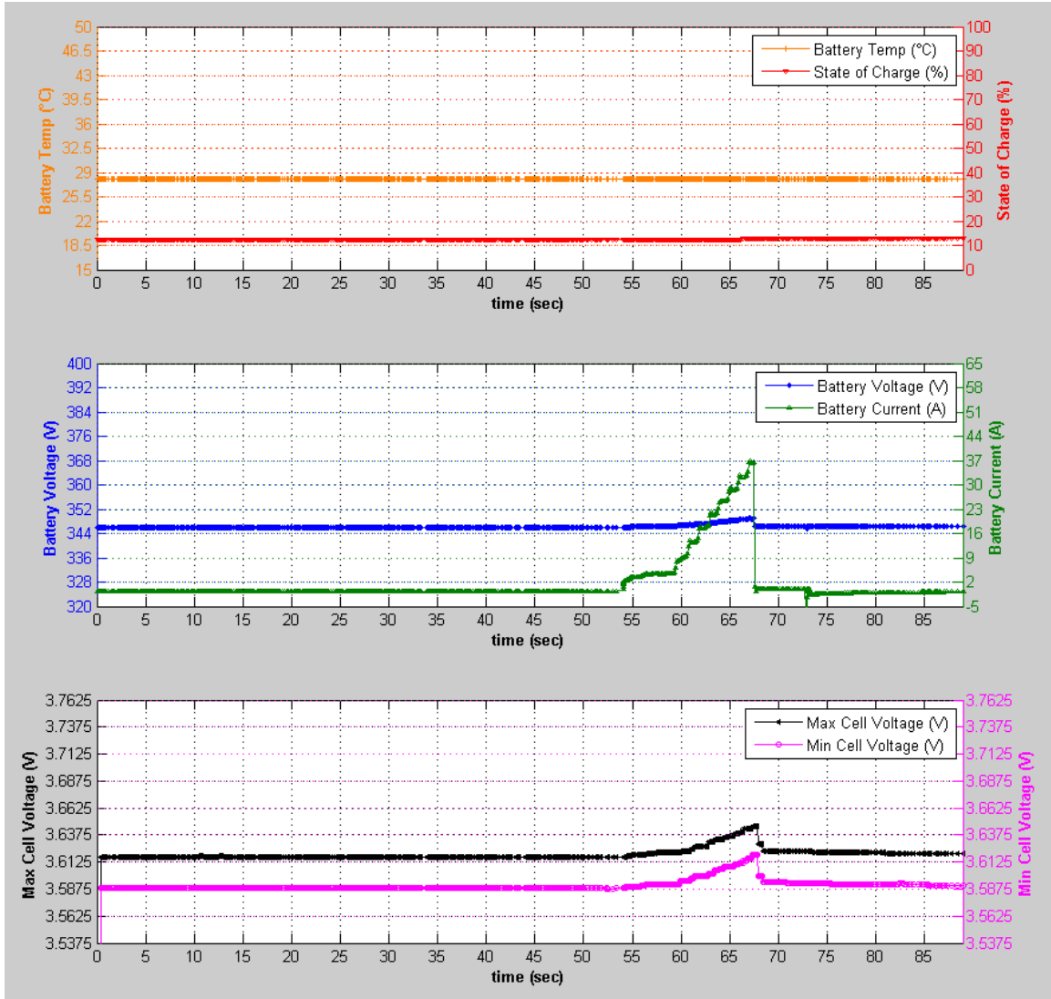
Figure 45: 100 \Omega During Charge Session Charge Data
