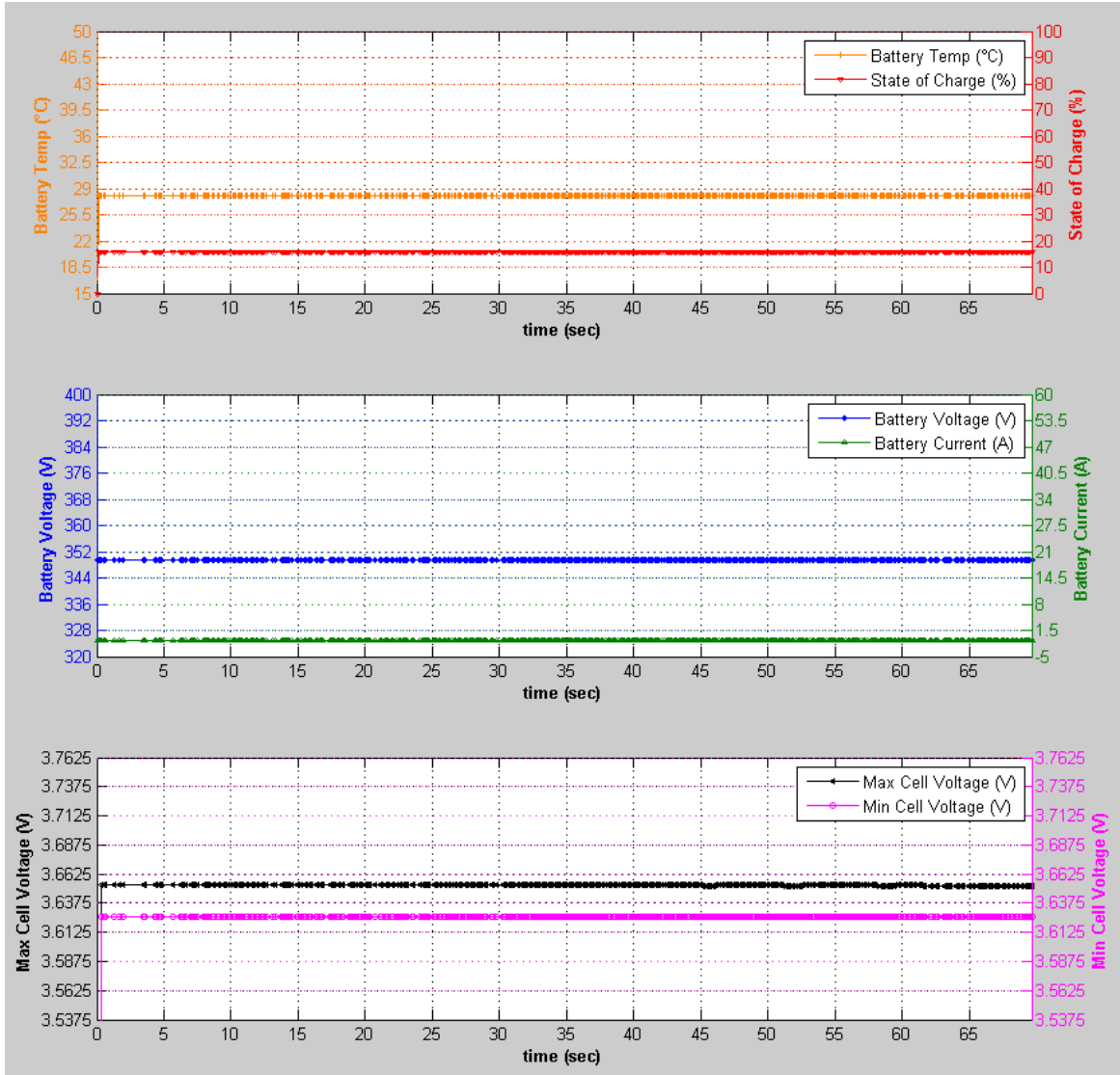
Figure 40: 1 k \Omega Before Charge Session Charge Data
