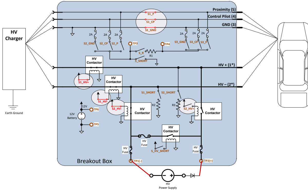
Figure 8: DC Bus Held High Test - Initial DC Fast-Charge Breakout Box Configuration
