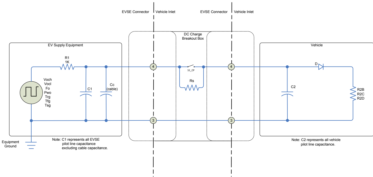
Figure 60: CCS Control Pilot Circuit With Added Series Resistance R_s . 2
