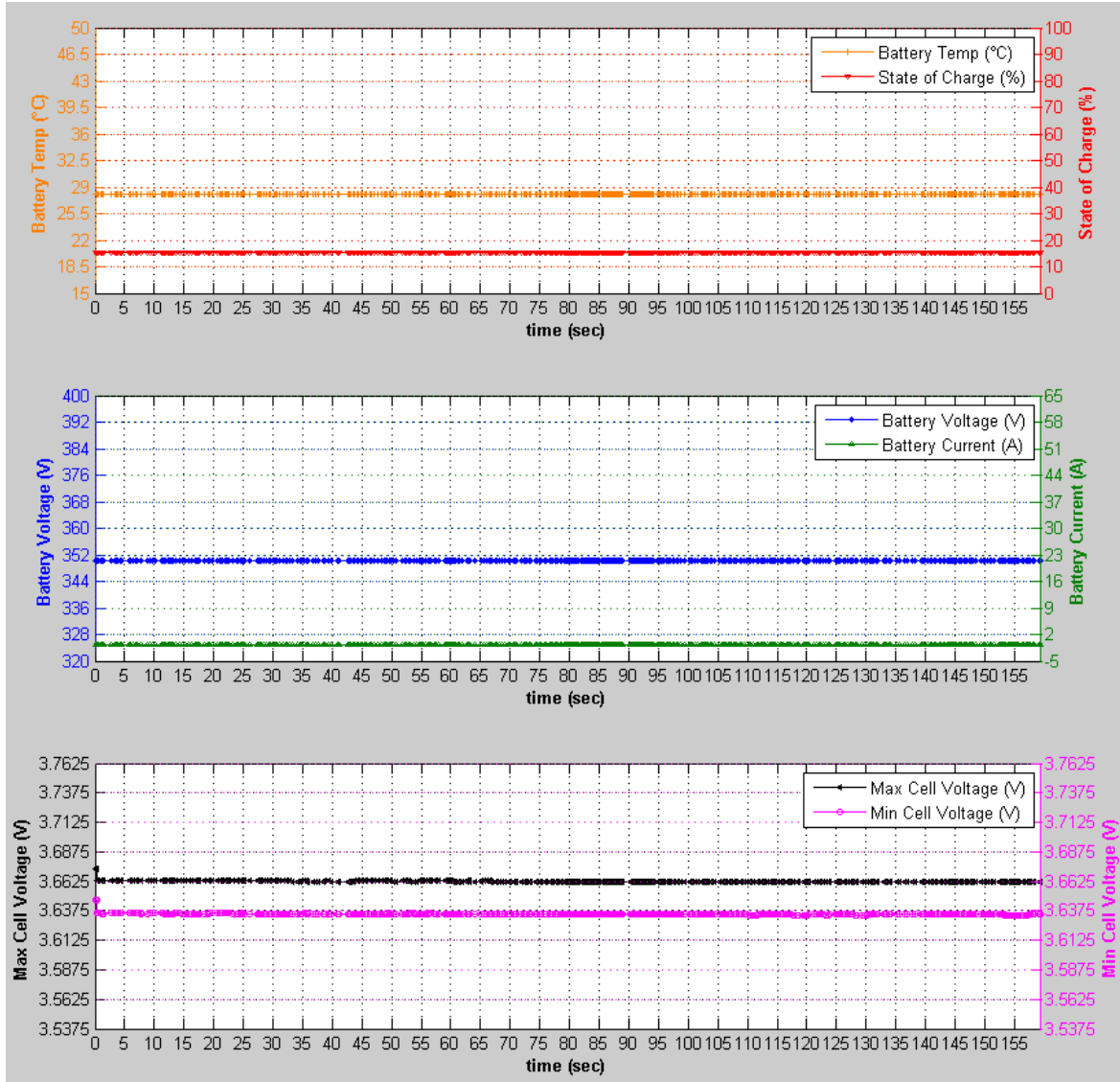
Figure 48: Gradual Decrease Before Charge Session Charge Data
