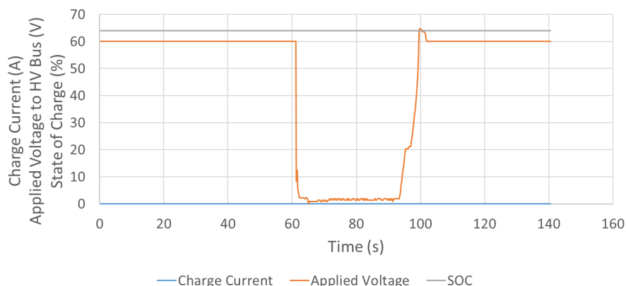
Figure 51: Before Charge Session Charge Data (60V applied to HV bus)
