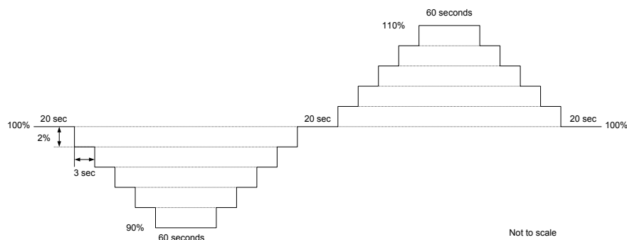
Figure 20: Voltage Range Variation
