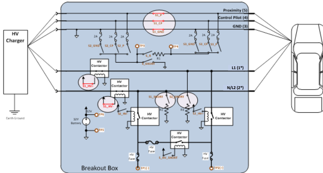
Figure 19: Charge Connector Control Signal Disturbance Test Setup
