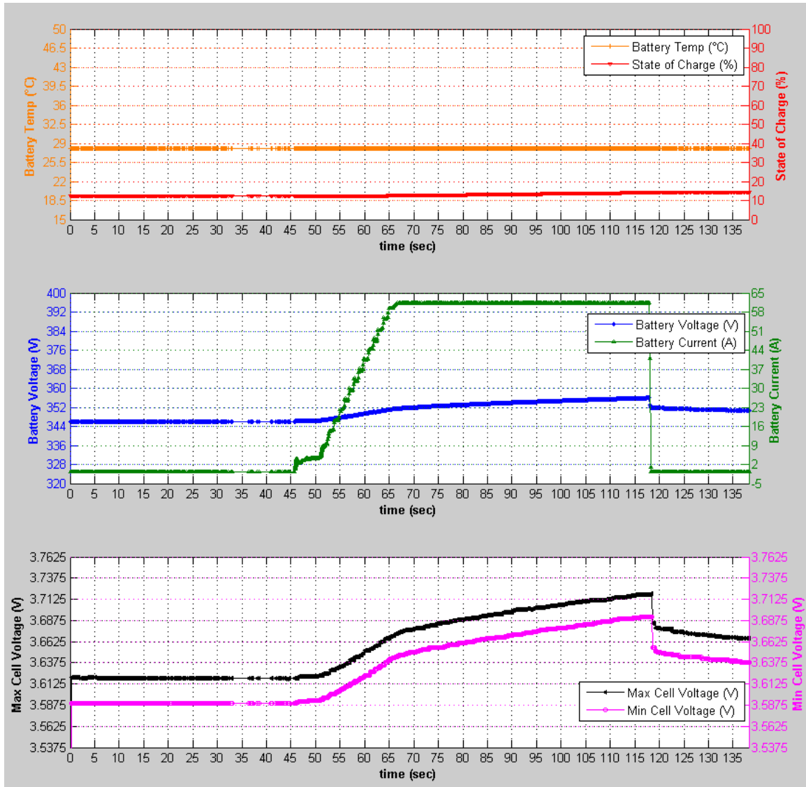
Figure 47: 24 \Omega During Charge Session Charge Data
