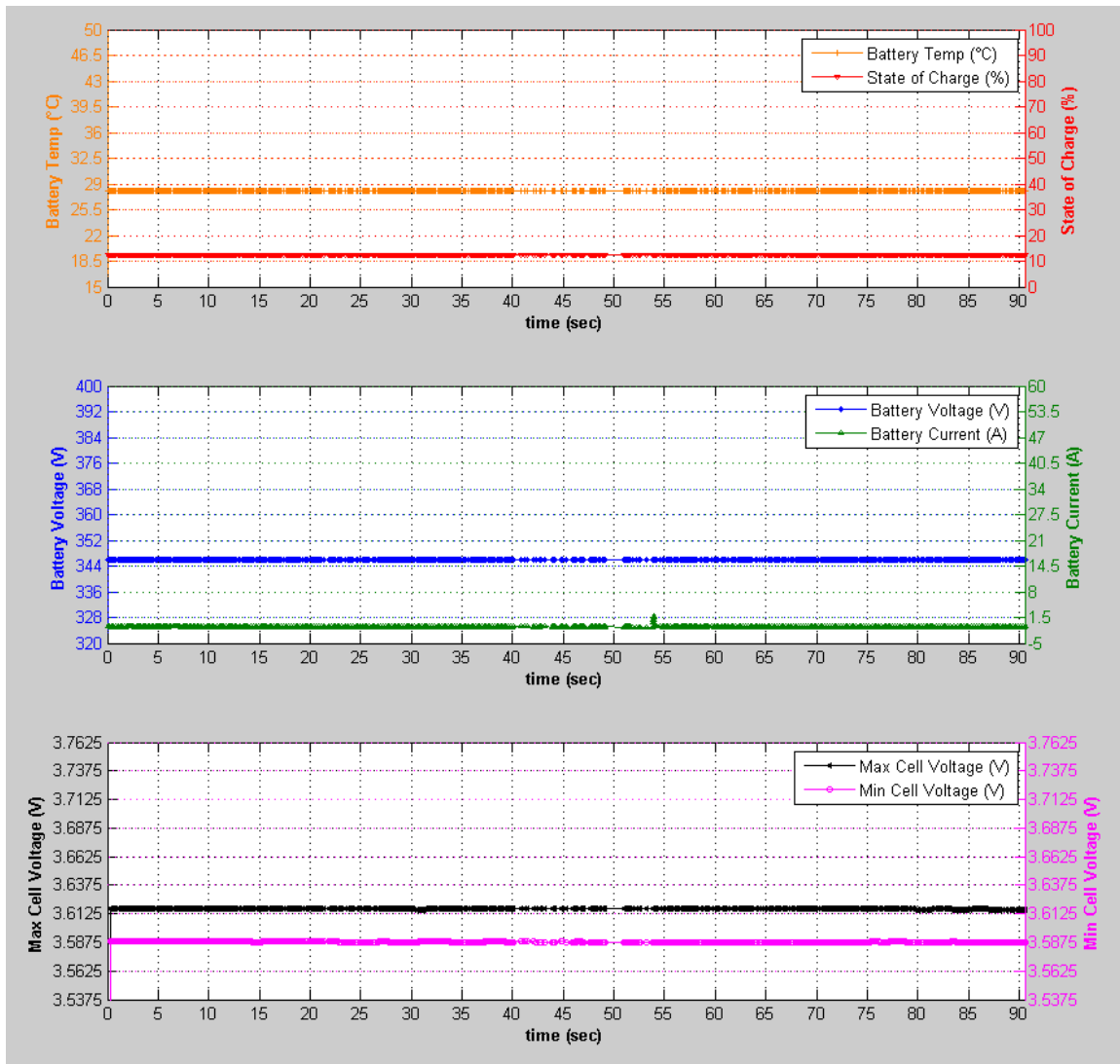
Figure 42: 47 Ω Before Charge Session Charge Data
