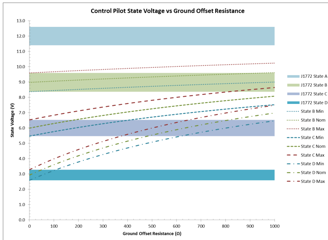
Figure 37: SAE J1772 Control Pilot State Voltage Versus Ground Offset Resistance (0 - 1 k \Omega )
