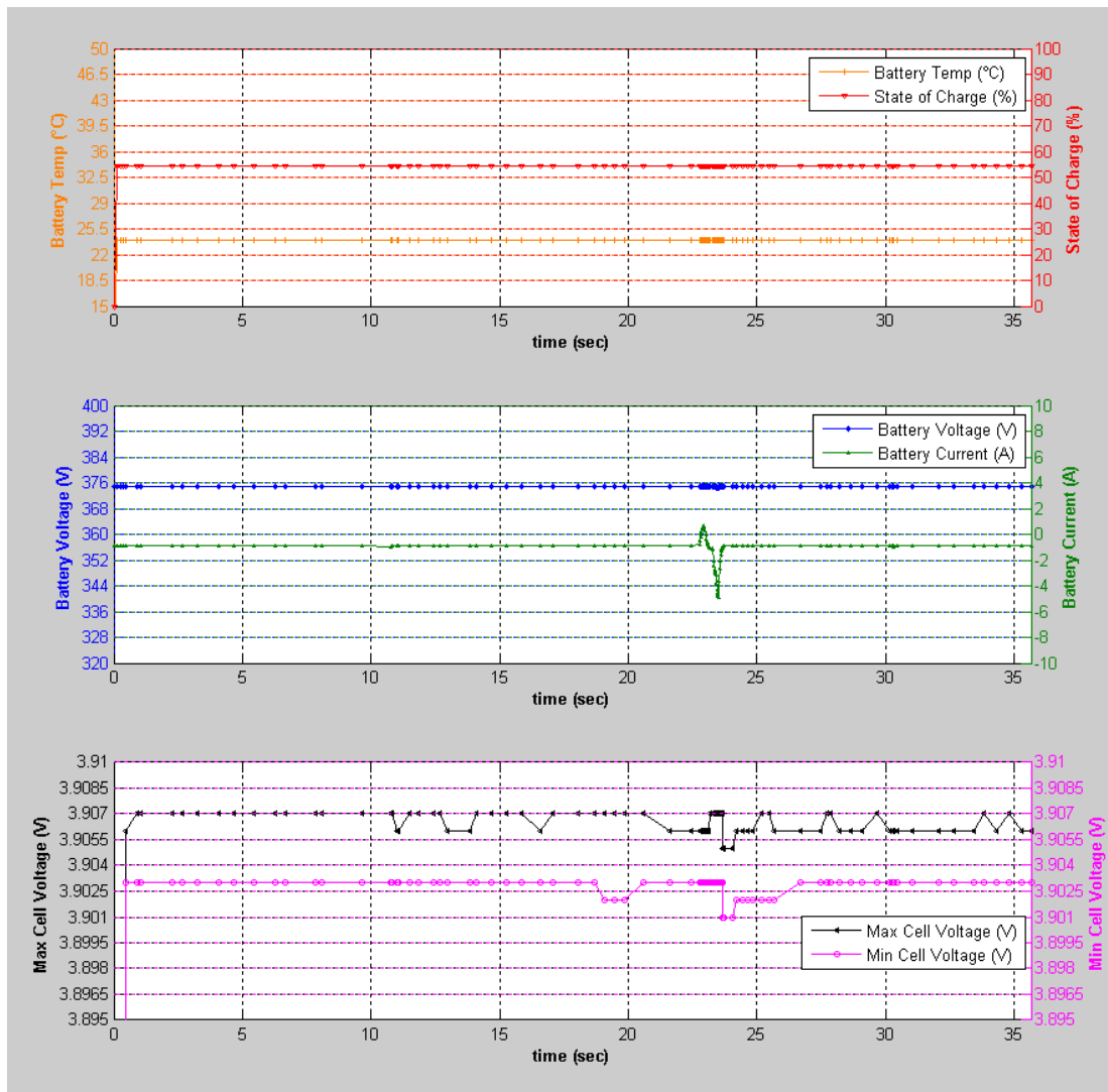
Figure 75: Reverse Power Flow Test Charge Data
