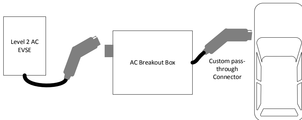
Figure 3: AC Charge Breakout Box Connection
