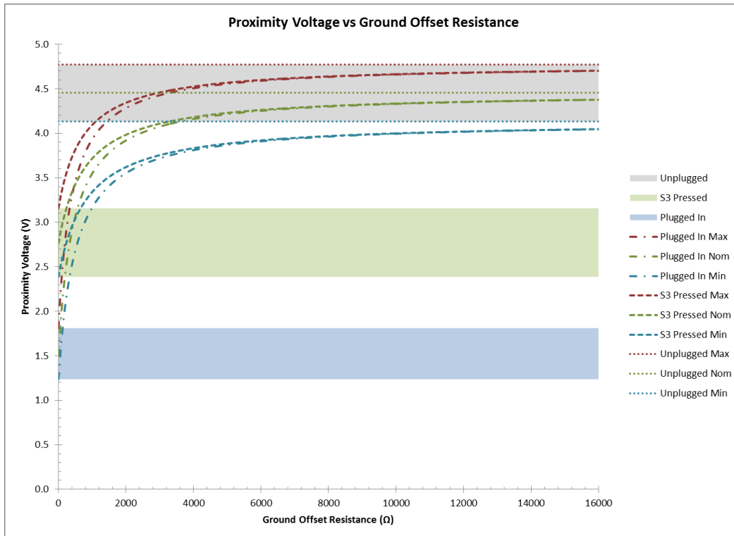
Figure 38: SAE J1772 Proximity Voltage Versus Ground Offset Resistance (0 - 16 k \Omega )
