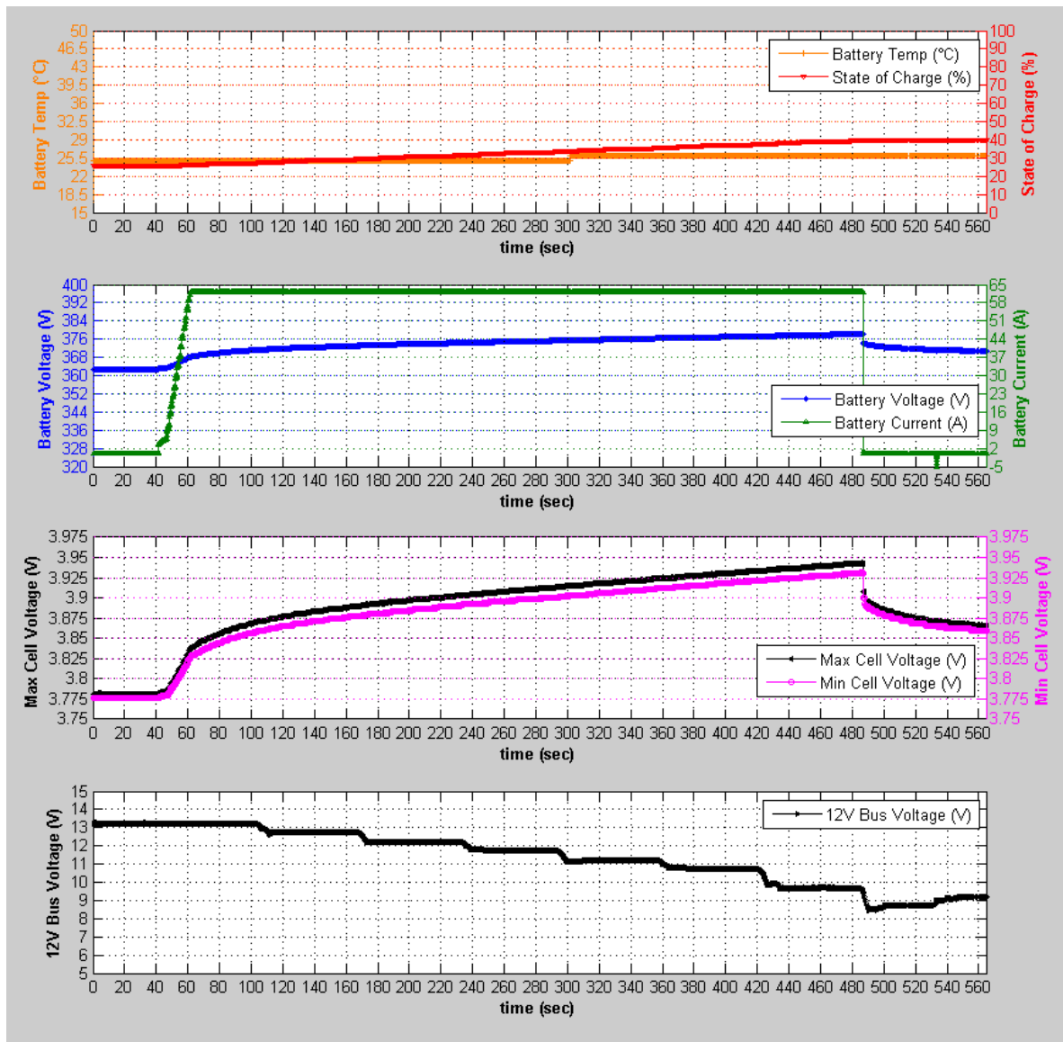
Figure 55: 12V System Under-Voltage Charge Data
