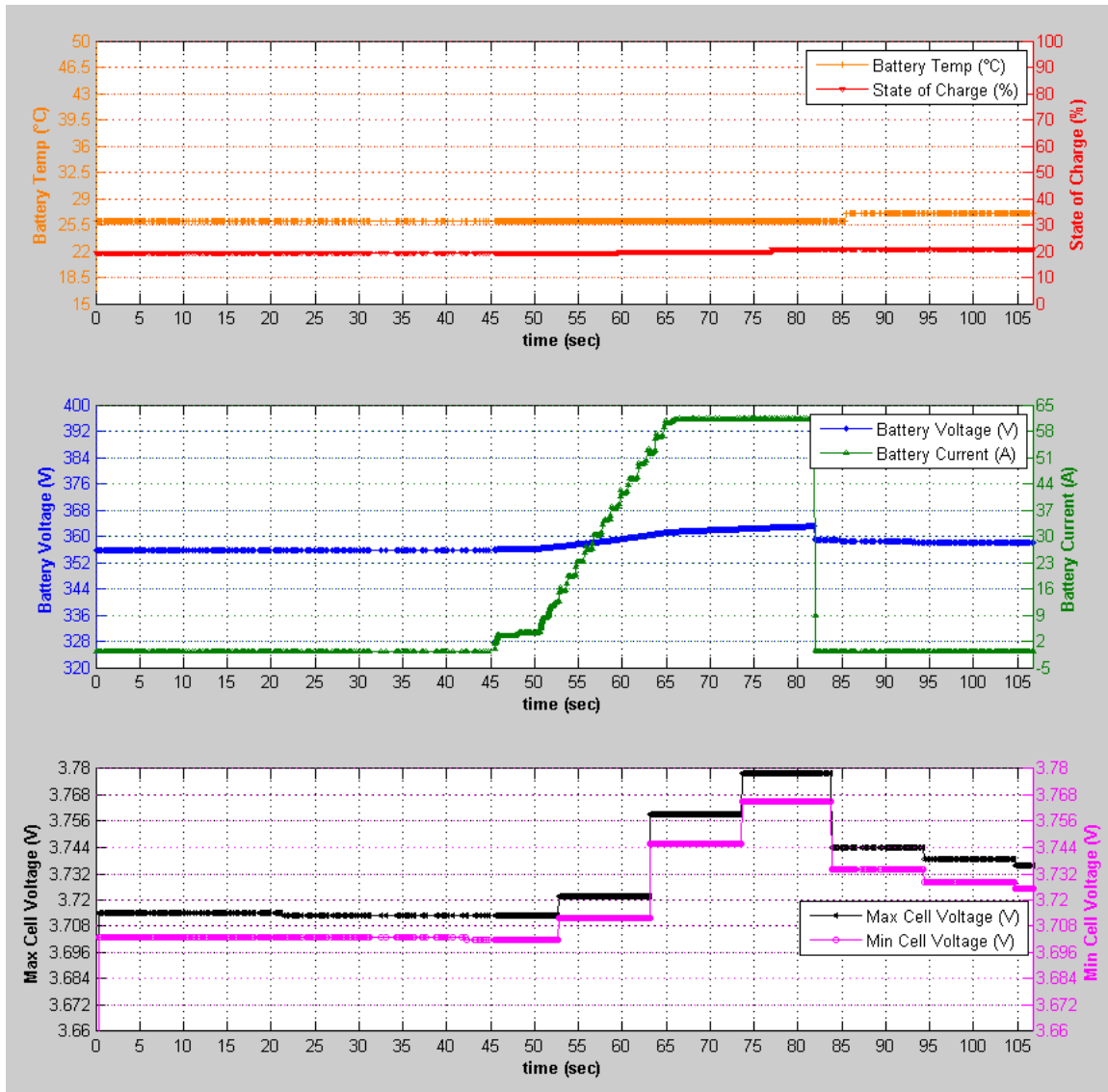
Figure 68: Disconnect HV- During Charge Session Charge Data
