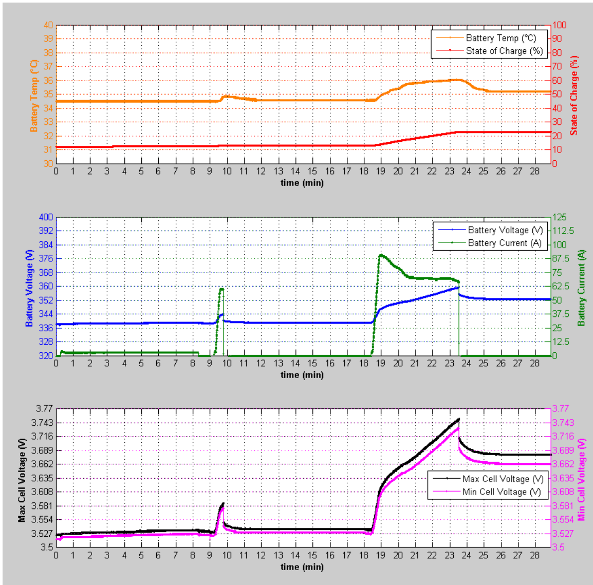
Figure 70: High Ambient Temperature (No Coolant) Charge Data
