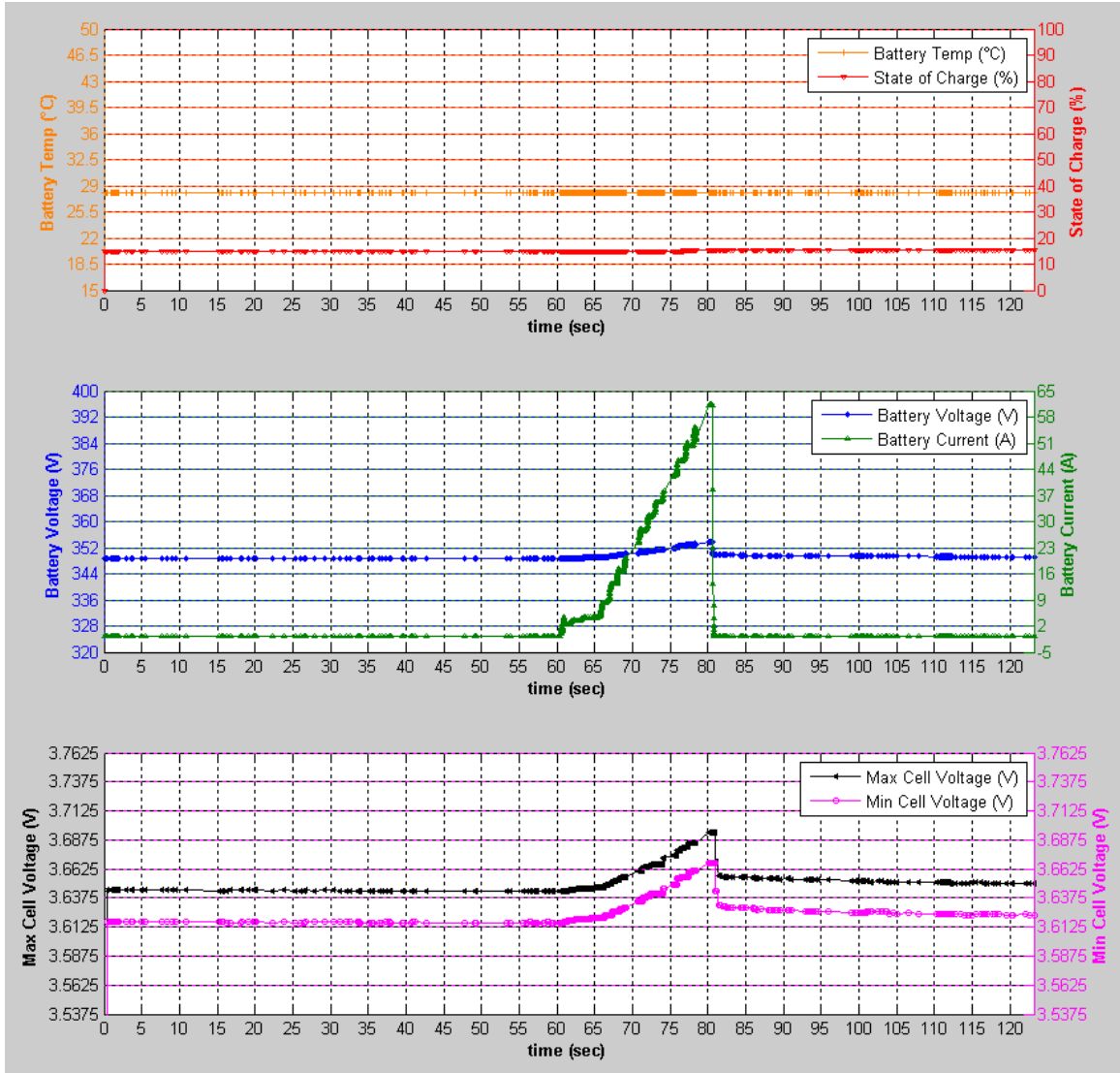
Figure 44: 1 k \Omega During Charge Session Charge Data
