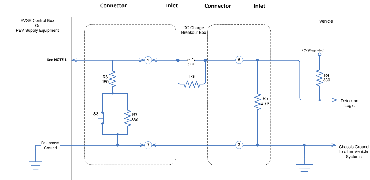
Figure 61: CCS Proximity Circuit With Added Series Resistance R_s . 2
