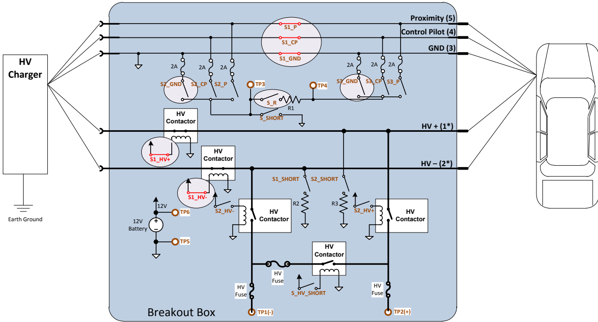
Figure 17: AC Bus Held High Test Setup
