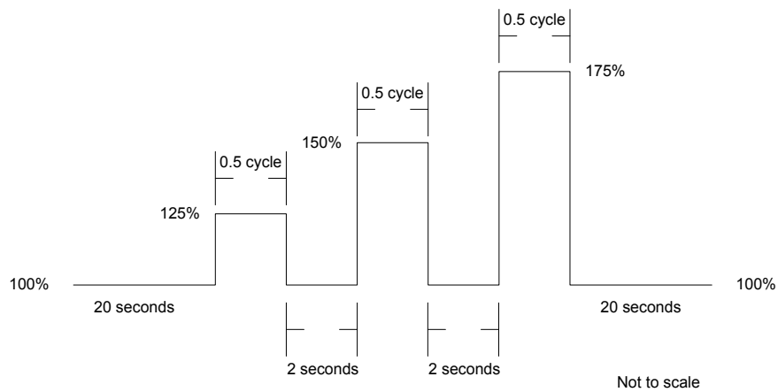
Figure 21: Voltage Swell
