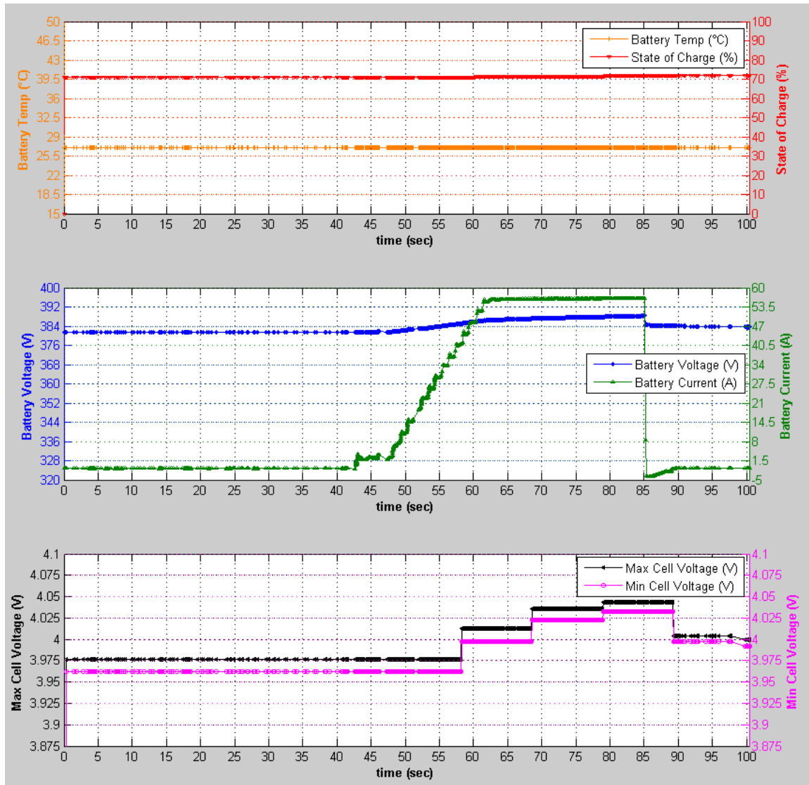
Figure 35: DC- to Gnd During Charge Session Charge Data
