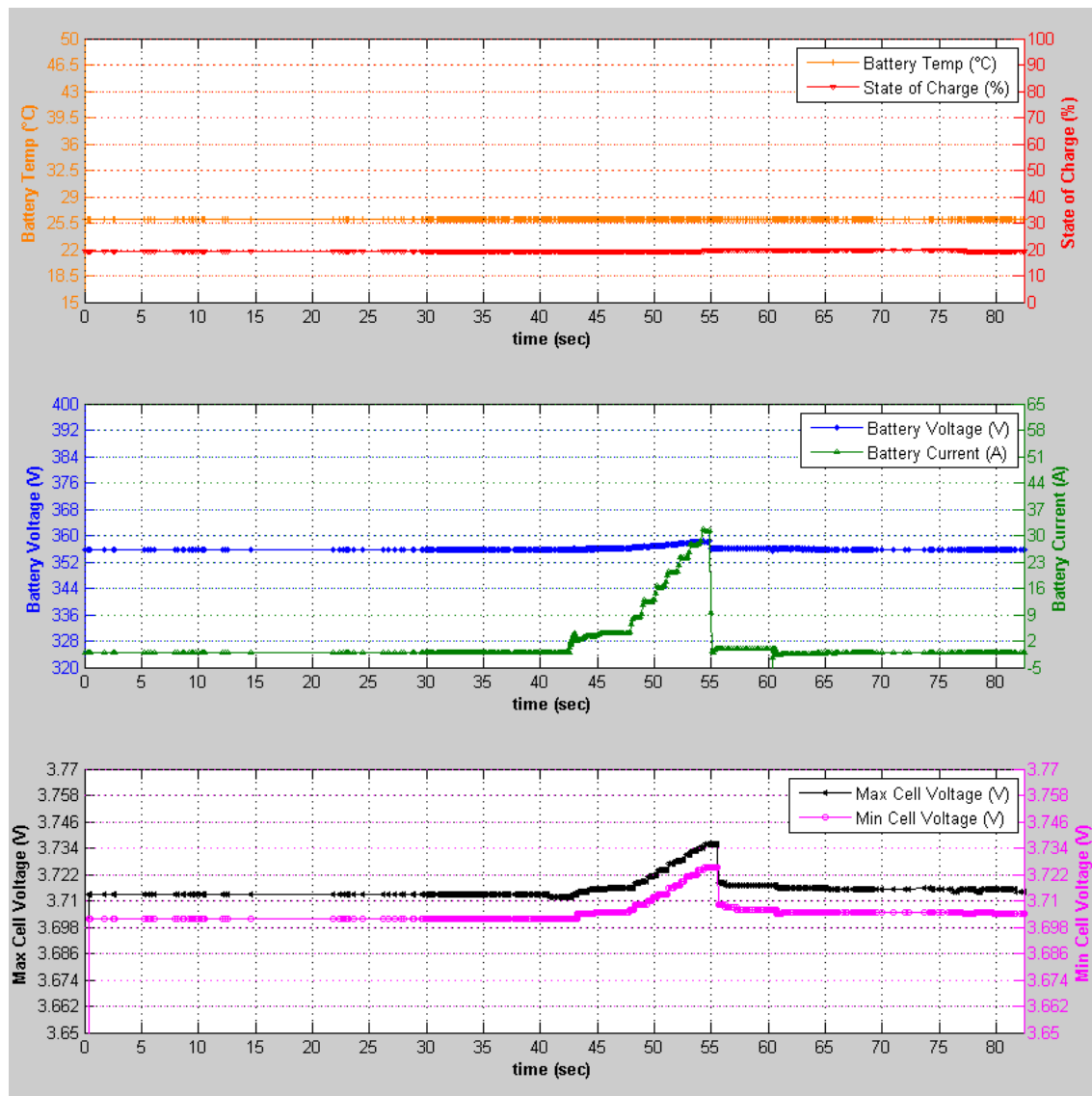
Figure 66: Charge Connector Ground Disturbance Charge Data
