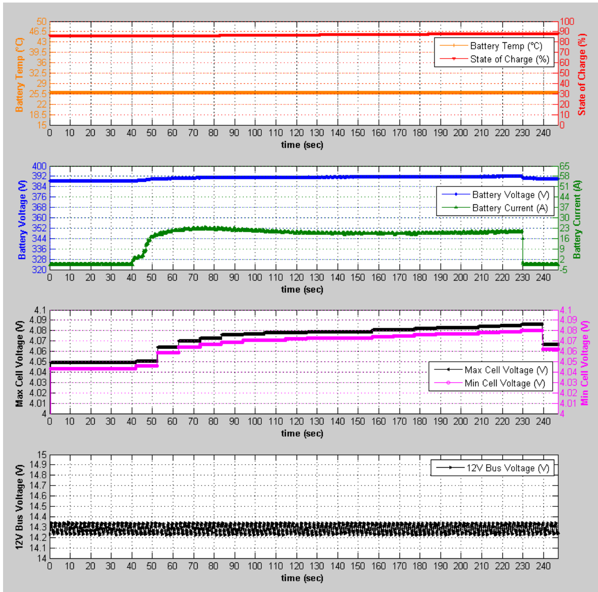
Figure 56: 12V System Disturbance Charge Data
