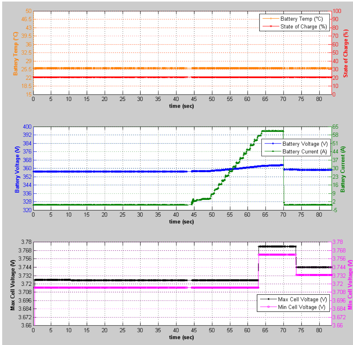
Figure 69: Disconnect HV- & HV+ During Charge Session Charge Data
