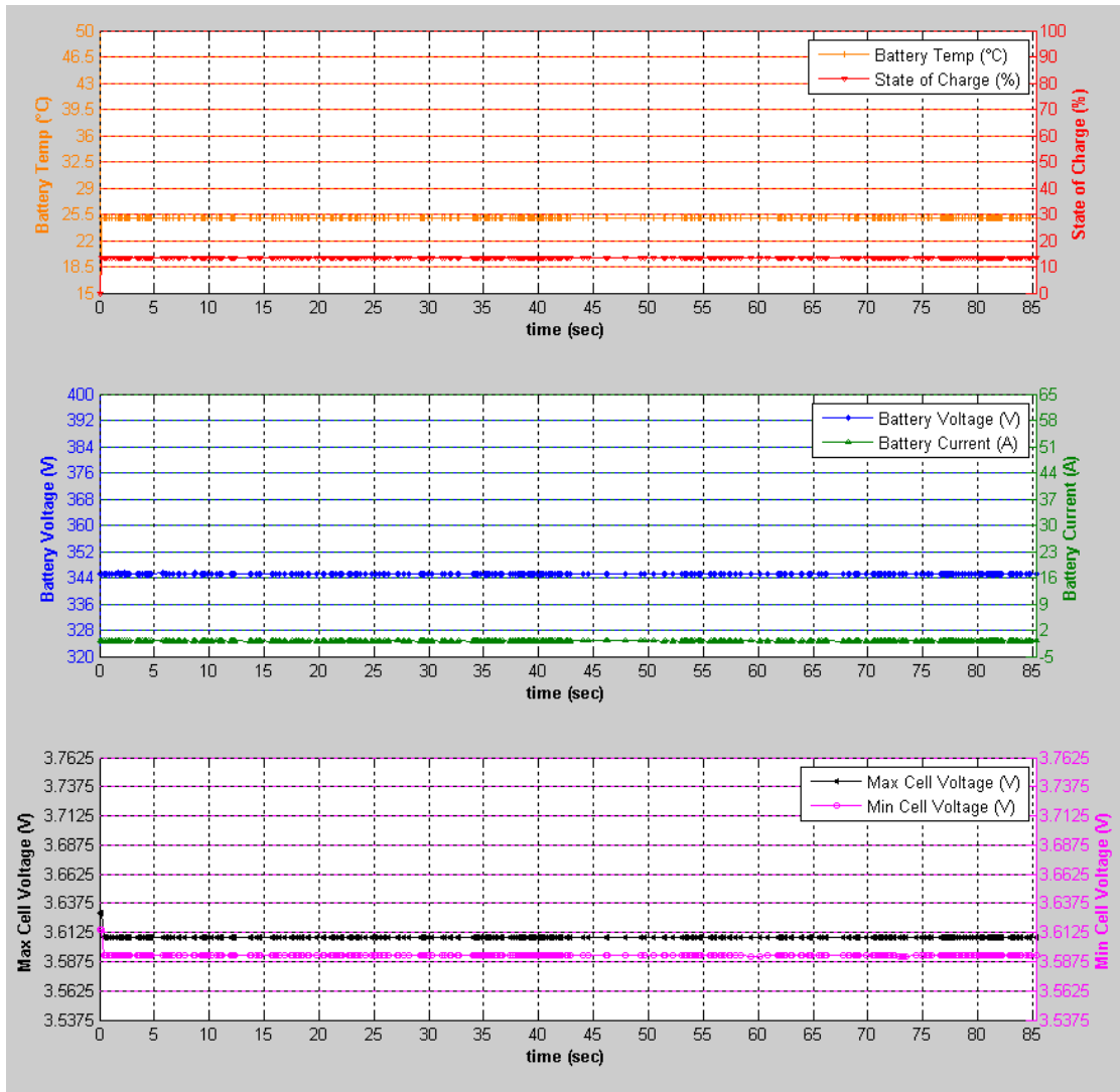
Figure 50: DC Bus Short Test Charge Data
