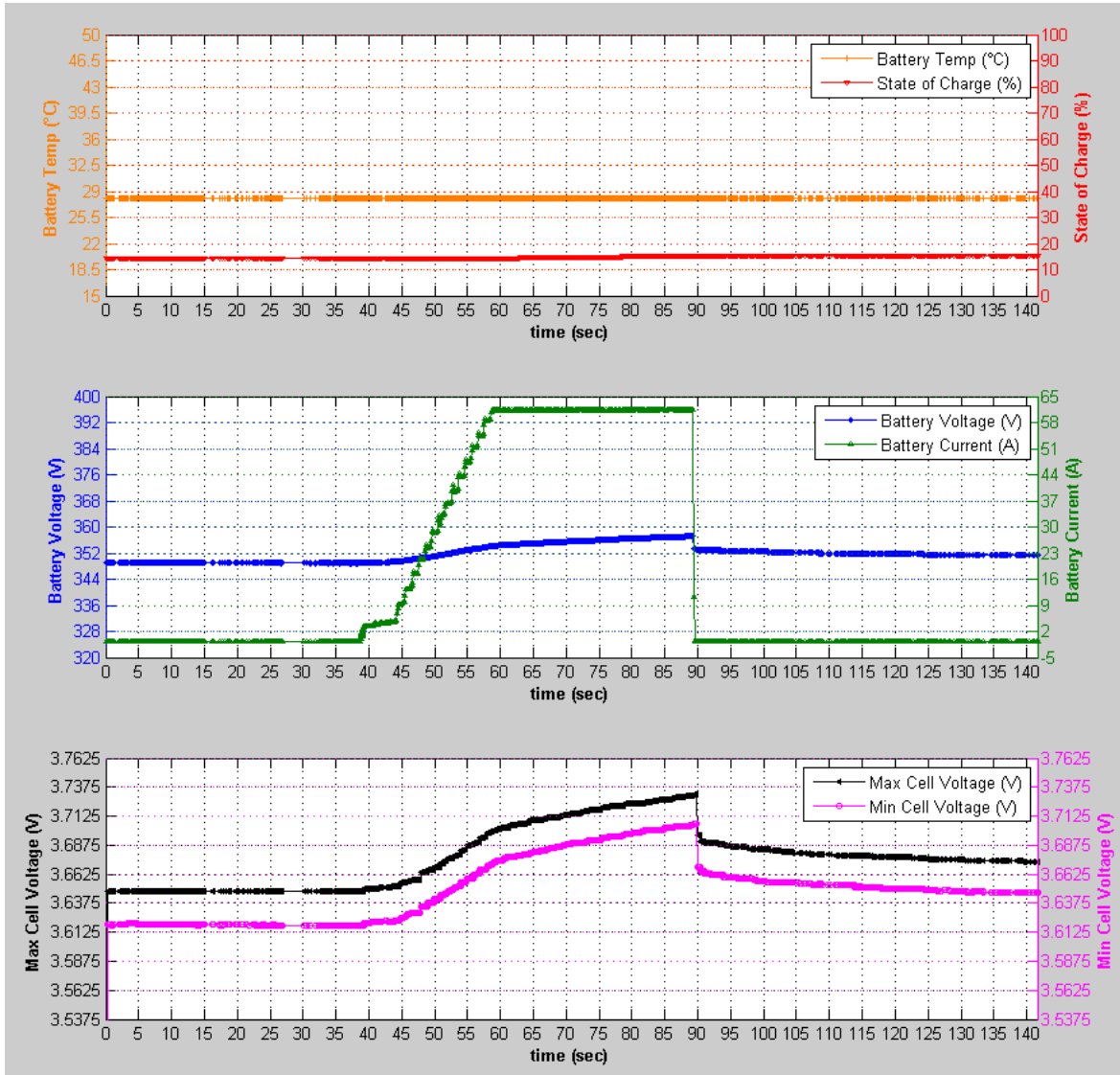
Figure 49: Gradual Increase During Charge Session Charge Data
