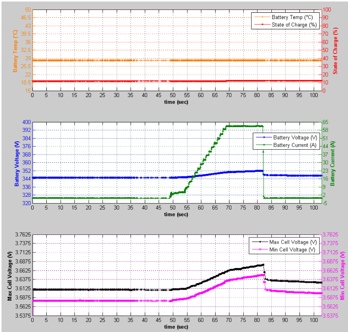
Figure 43: 24 Ω Before Charge Session Charge Data
