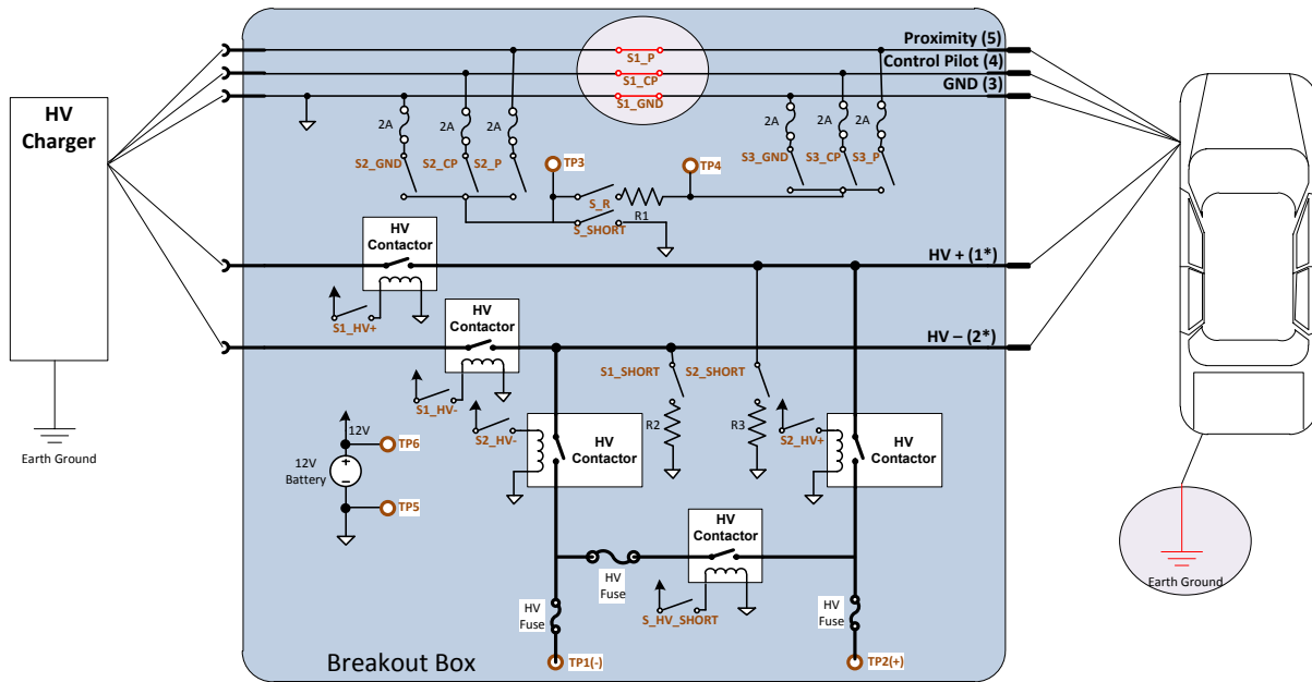
Figure 13: Ground Connection Disturbance Test - Initial Breakout Box Configuration
