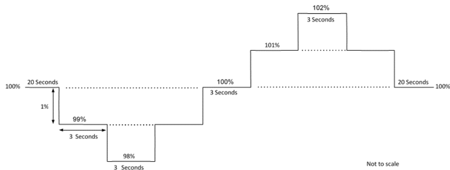
Figure 24: Frequency Range Variation
