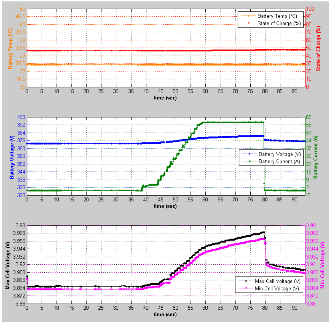
Figure 62: Control Pilot Open During Charge Session Charge Data
