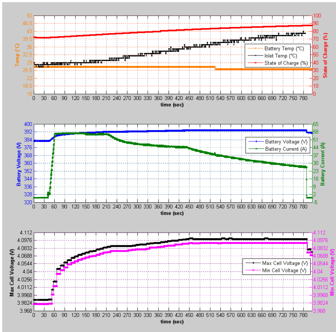
Figure 76: PEV Inlet Temperature Test Charge Data
