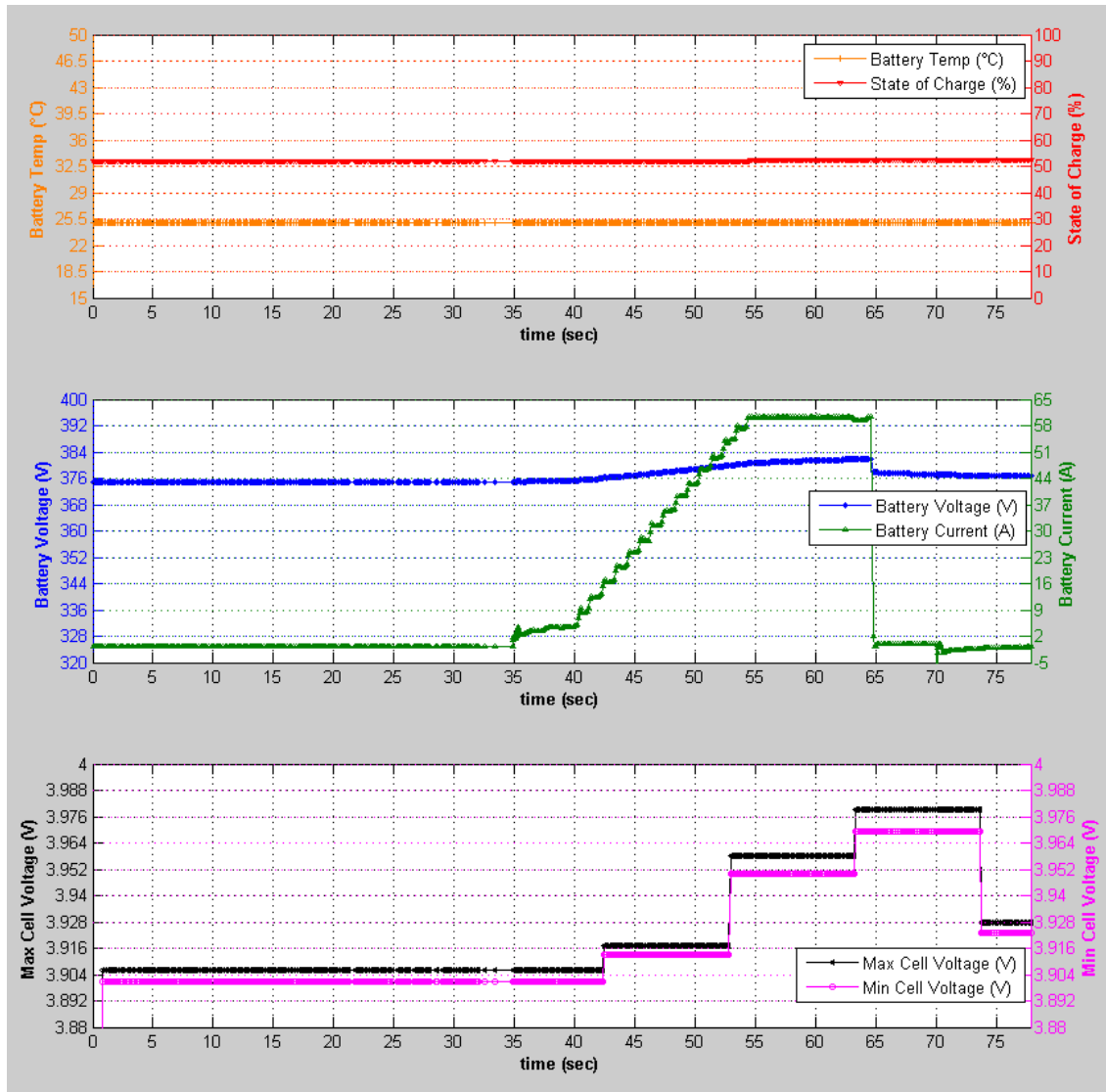
Figure 65: Proximity Short to Gnd During Charge Session Charge Data
