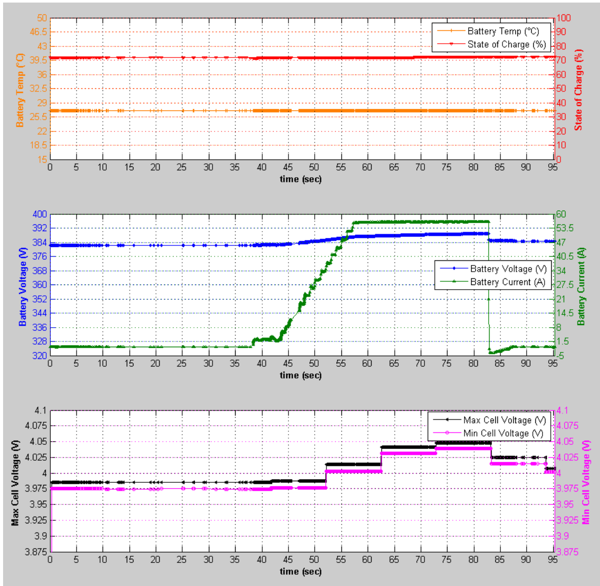
Figure 34: DC+ to Gnd During Charge Session Charge Data
