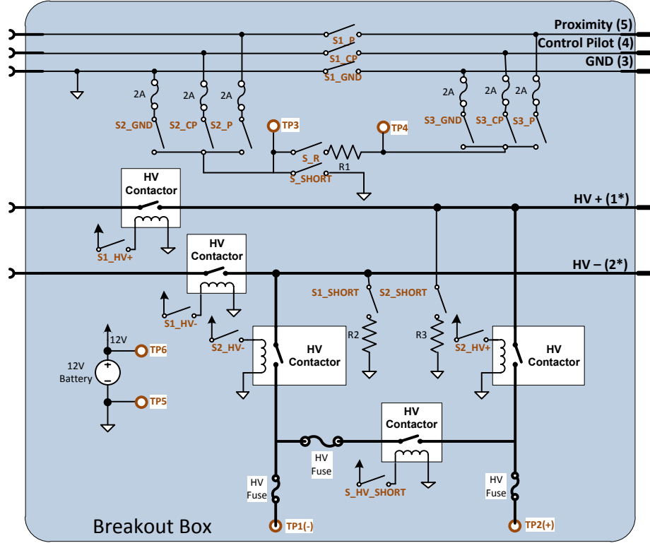
Figure 2: DC Fast-Charge Breakout Box Schematic (CCS version shown)
