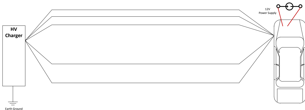
Figure 10: 12V System Under Voltage Test – 12V Power Supply Connection
