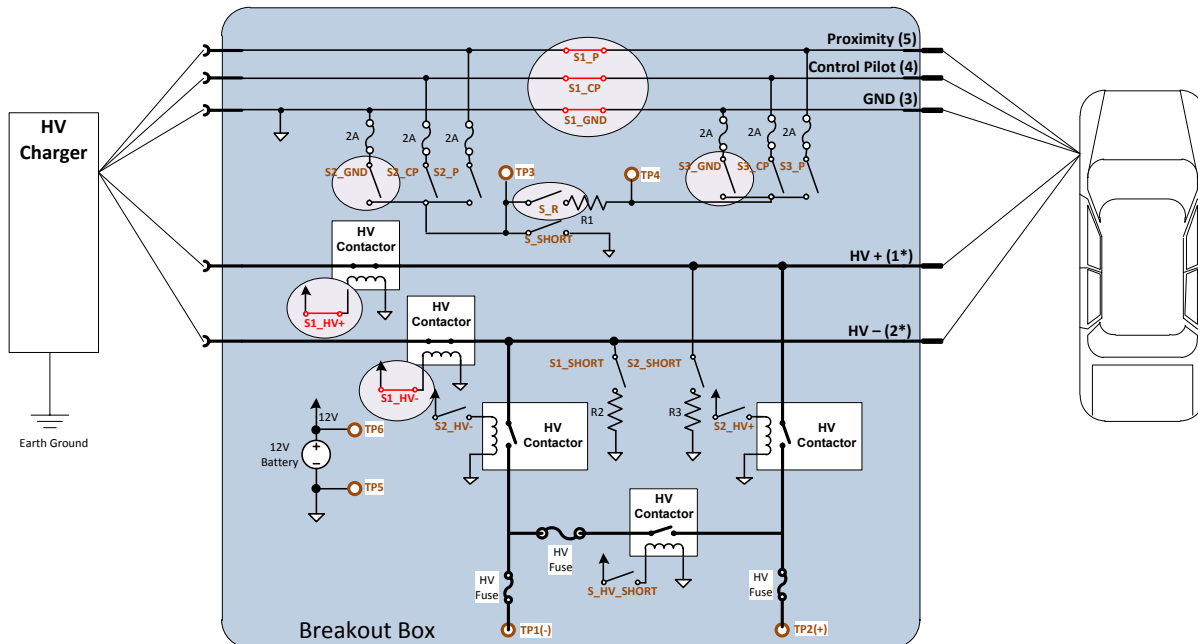
Figure 6: Chassis Ground Offset Test - Initial DC Fast-Charge Breakout Box Configuration
