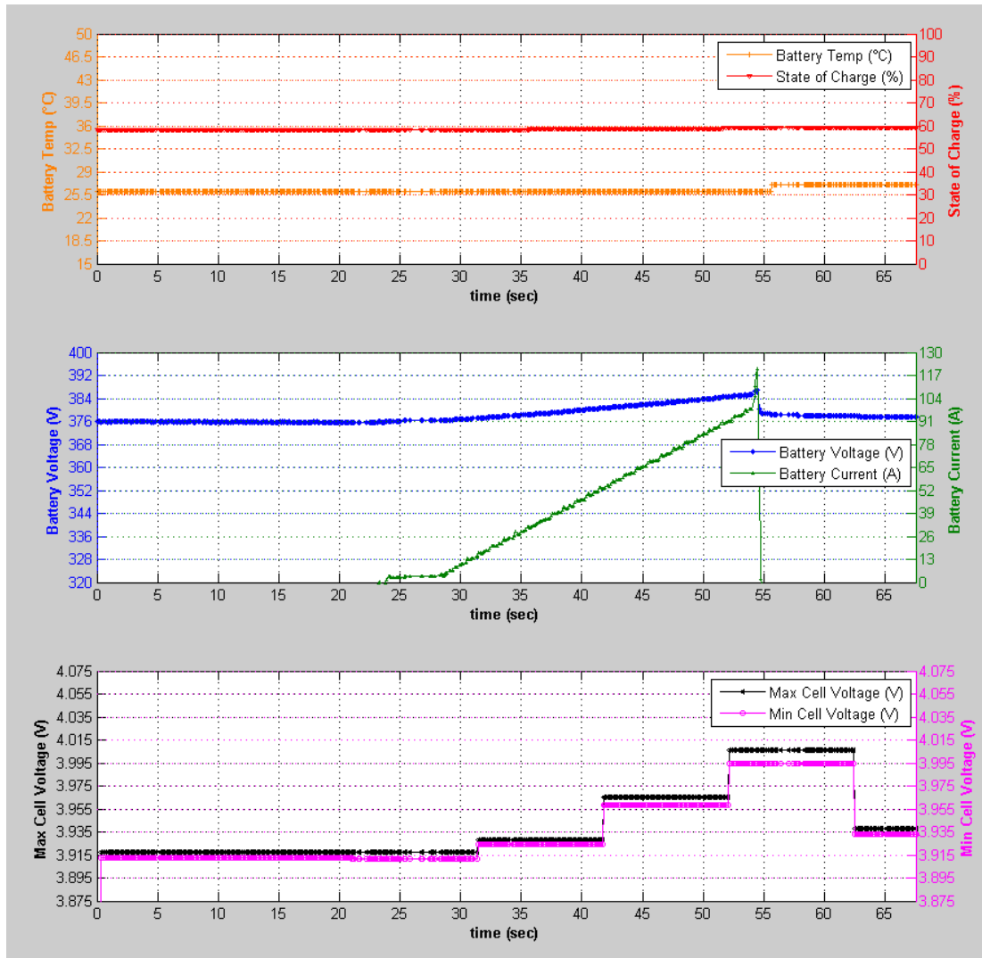
Figure 74: Over-Current Test Charge Data (20A Over)
