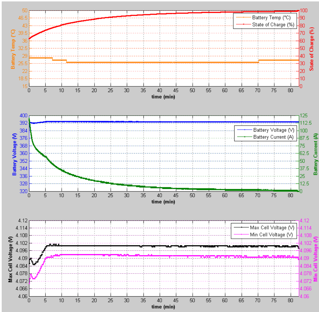
Figure 72: Over-Charge Test Charge Data
