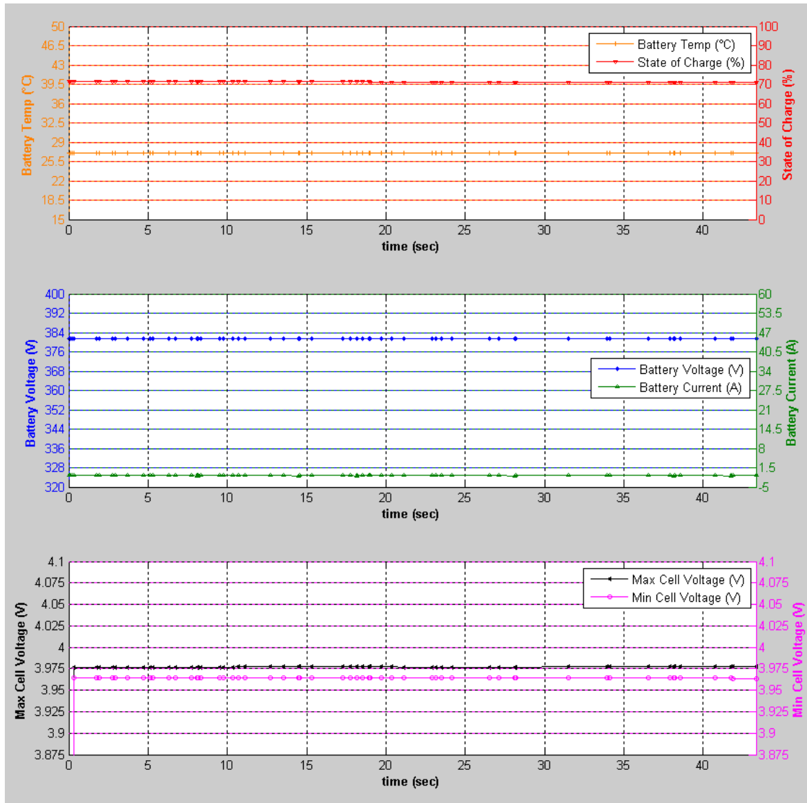
Figure 33: DC- to Gnd Before Charge Session Charge Data
