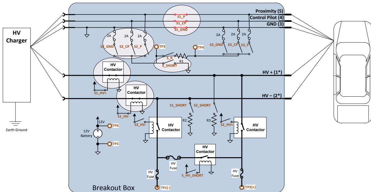
Figure 12: Control Signal Disturbance Test - Initial Breakout Box Configuration
