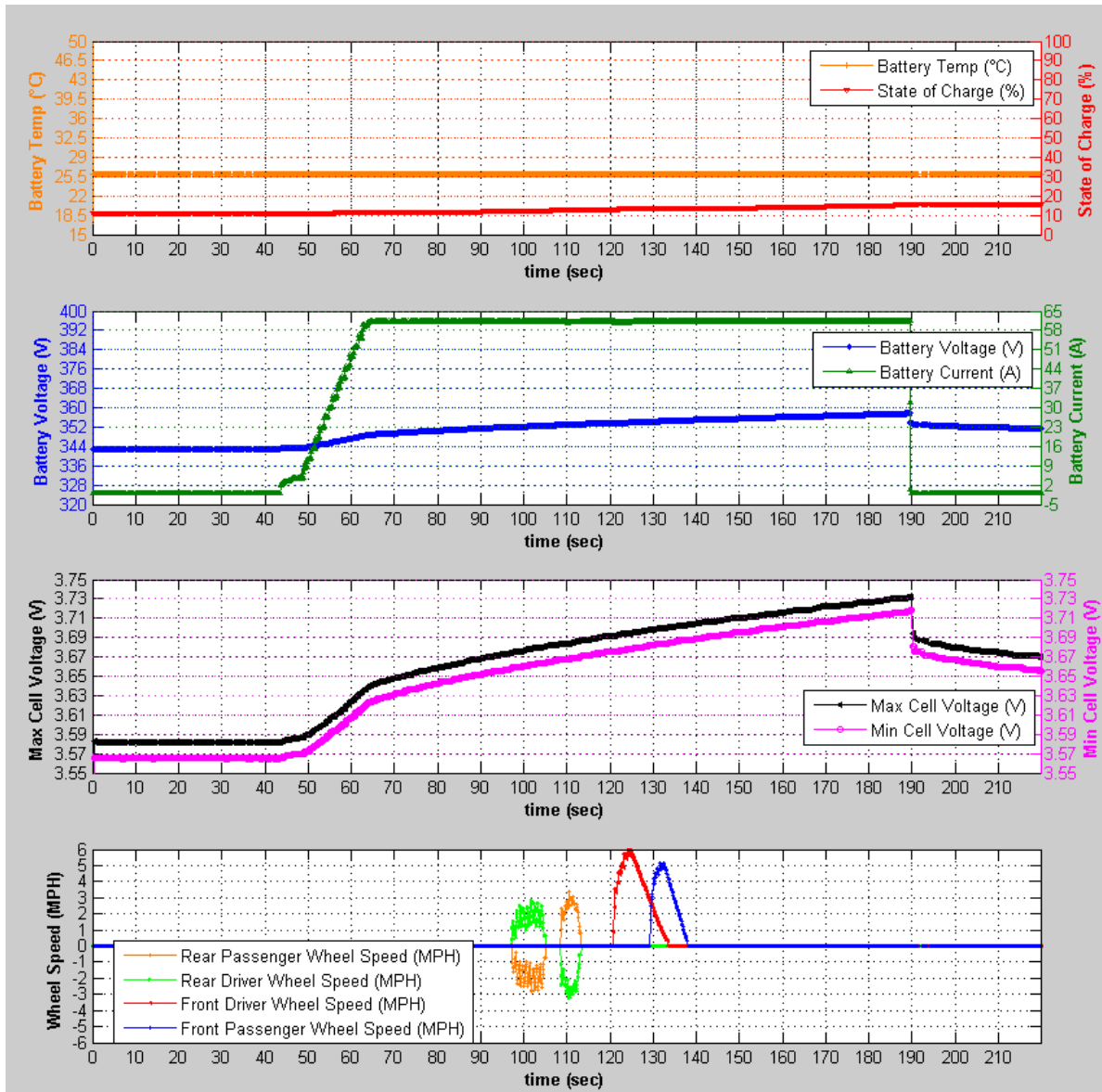
Figure 57: Drive Attempt while Charging and Simulated PEV Movement Data
