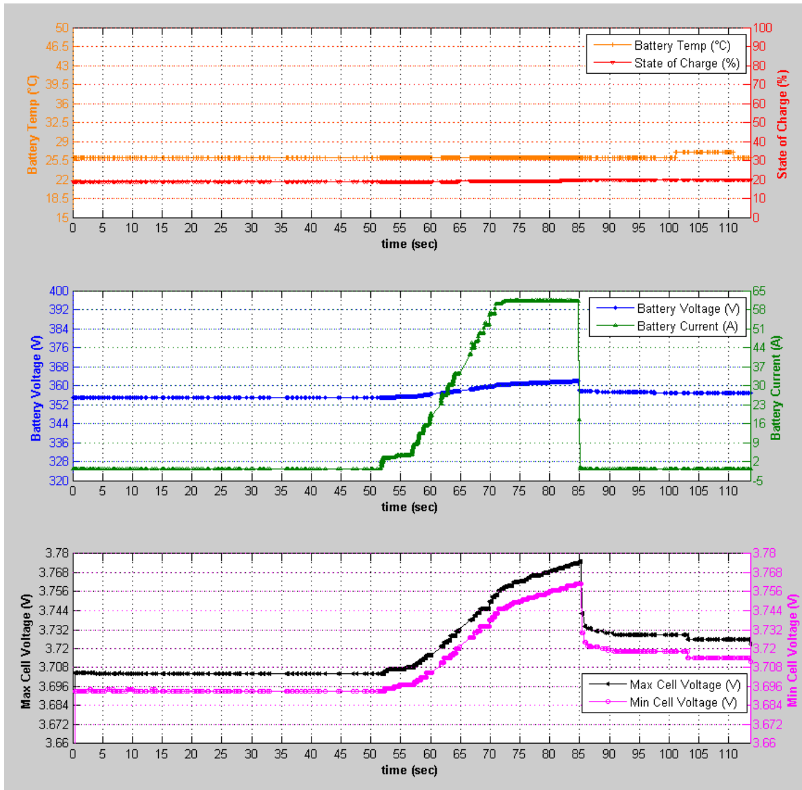
Figure 67: Disconnect HV+ During Charge Session Charge Data
