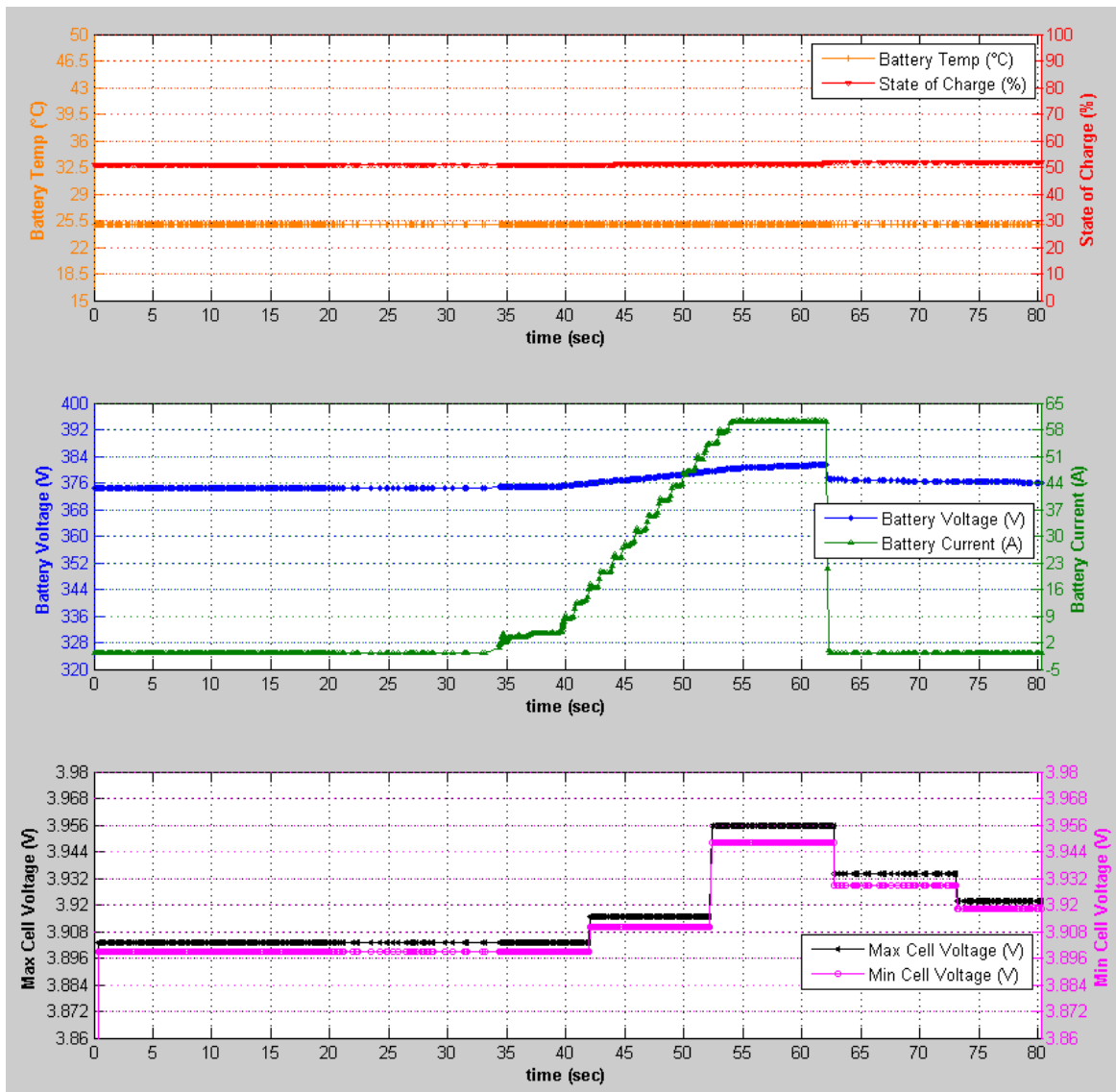
Figure 63: Control Pilot Short to Gnd During Charge Session Charge Data
