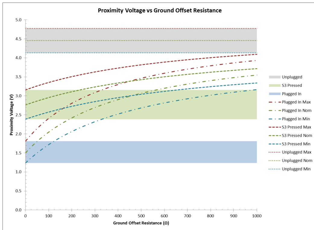
Figure 39: SAE J1772 Proximity Voltage Versus Ground Offset Resistance (0 - 1 k \Omega )
