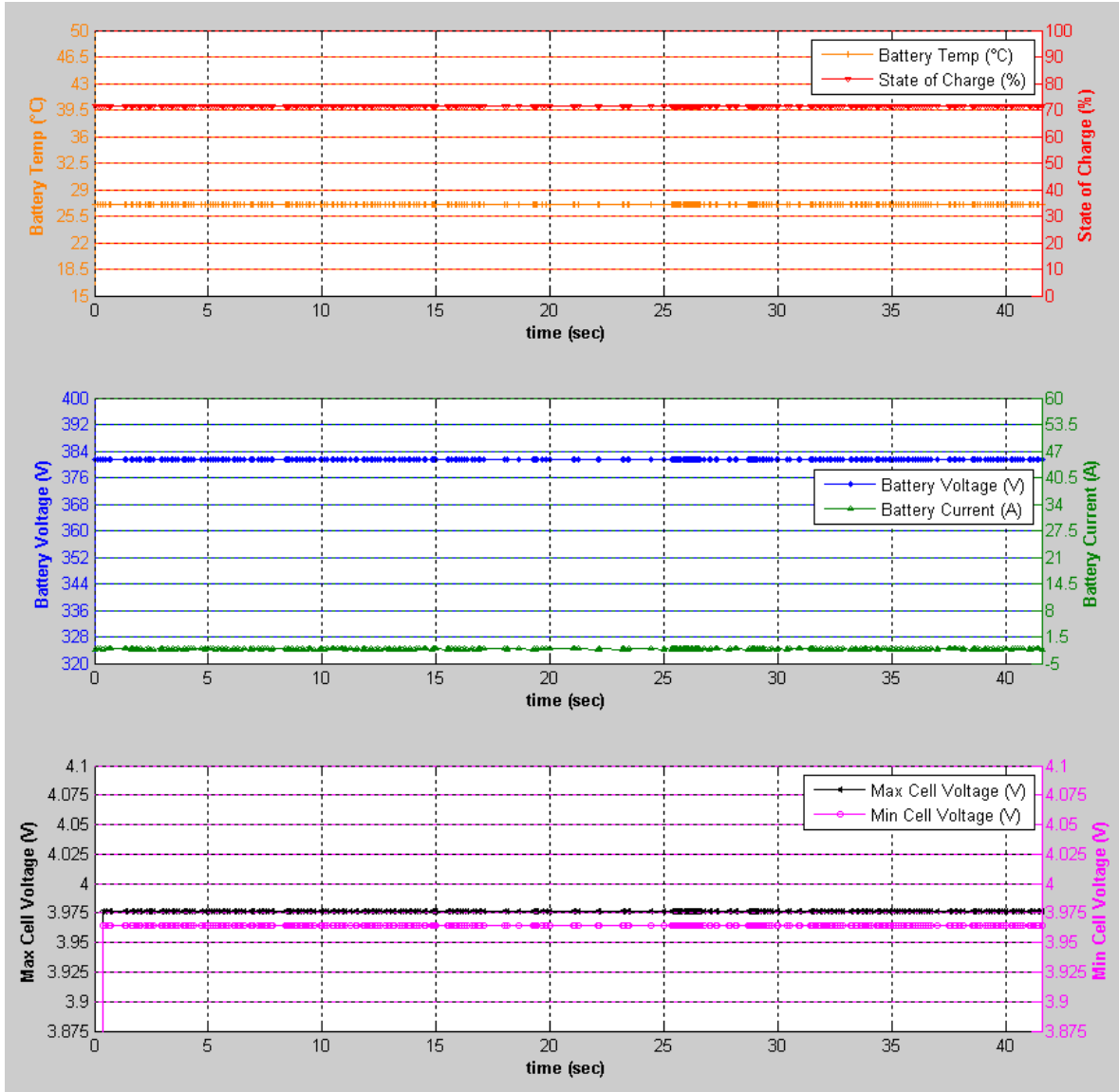
Figure 32: DC+ to Gnd Before Charge Session Charge Data
