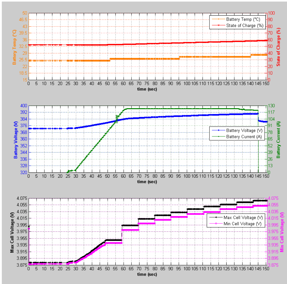
Figure 73: Over-Current Test Charge Data (10A Over)
