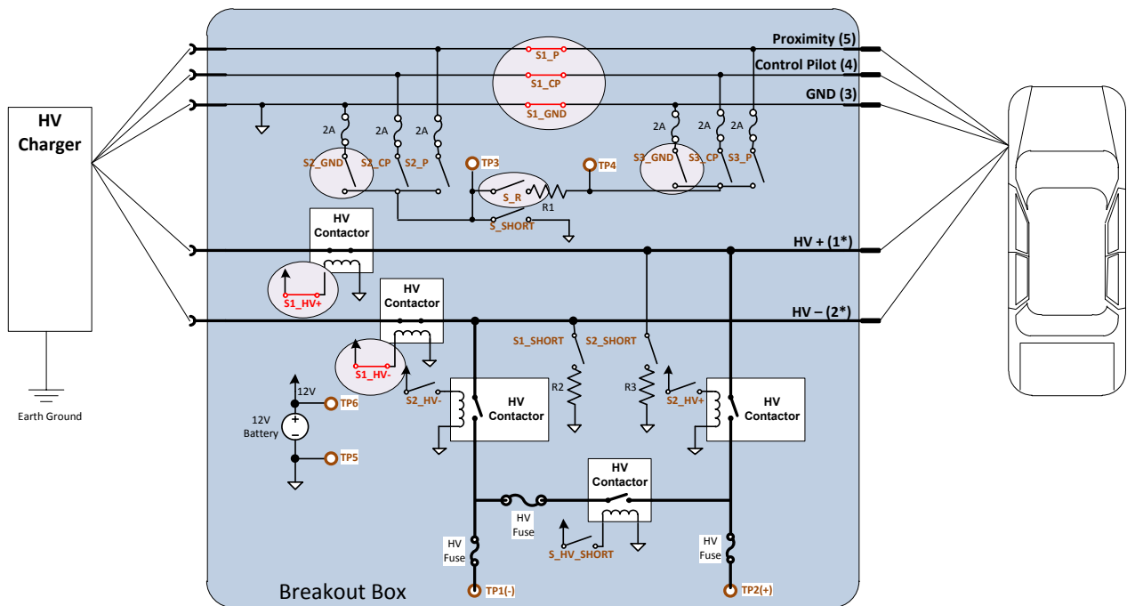
Figure 16: Chassis Ground Offset Test Setup
