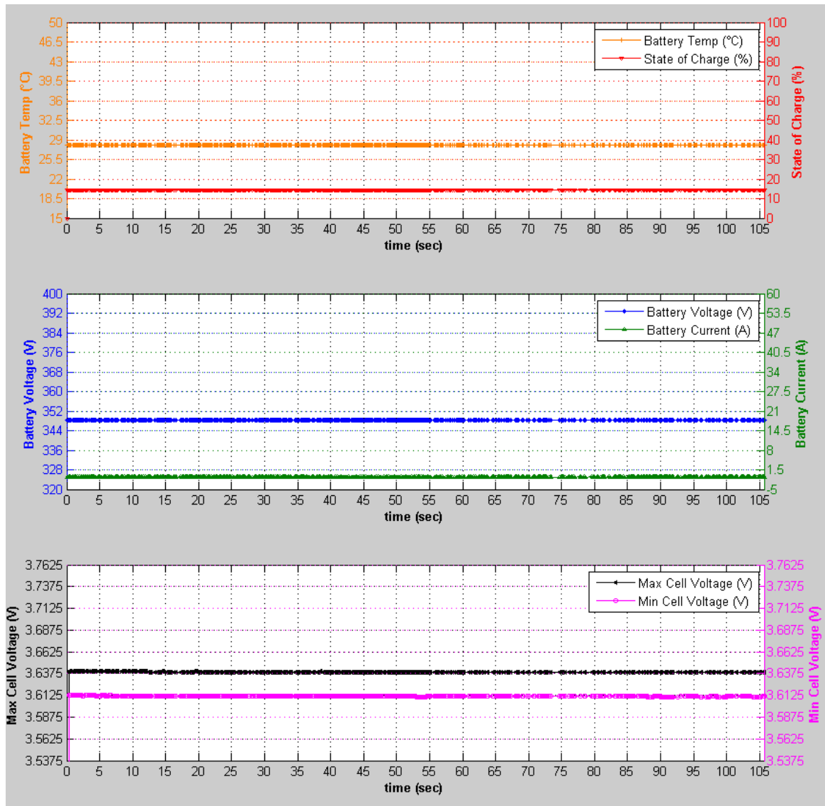
Figure 41: 100 \Omega Before Charge Session Charge Data
