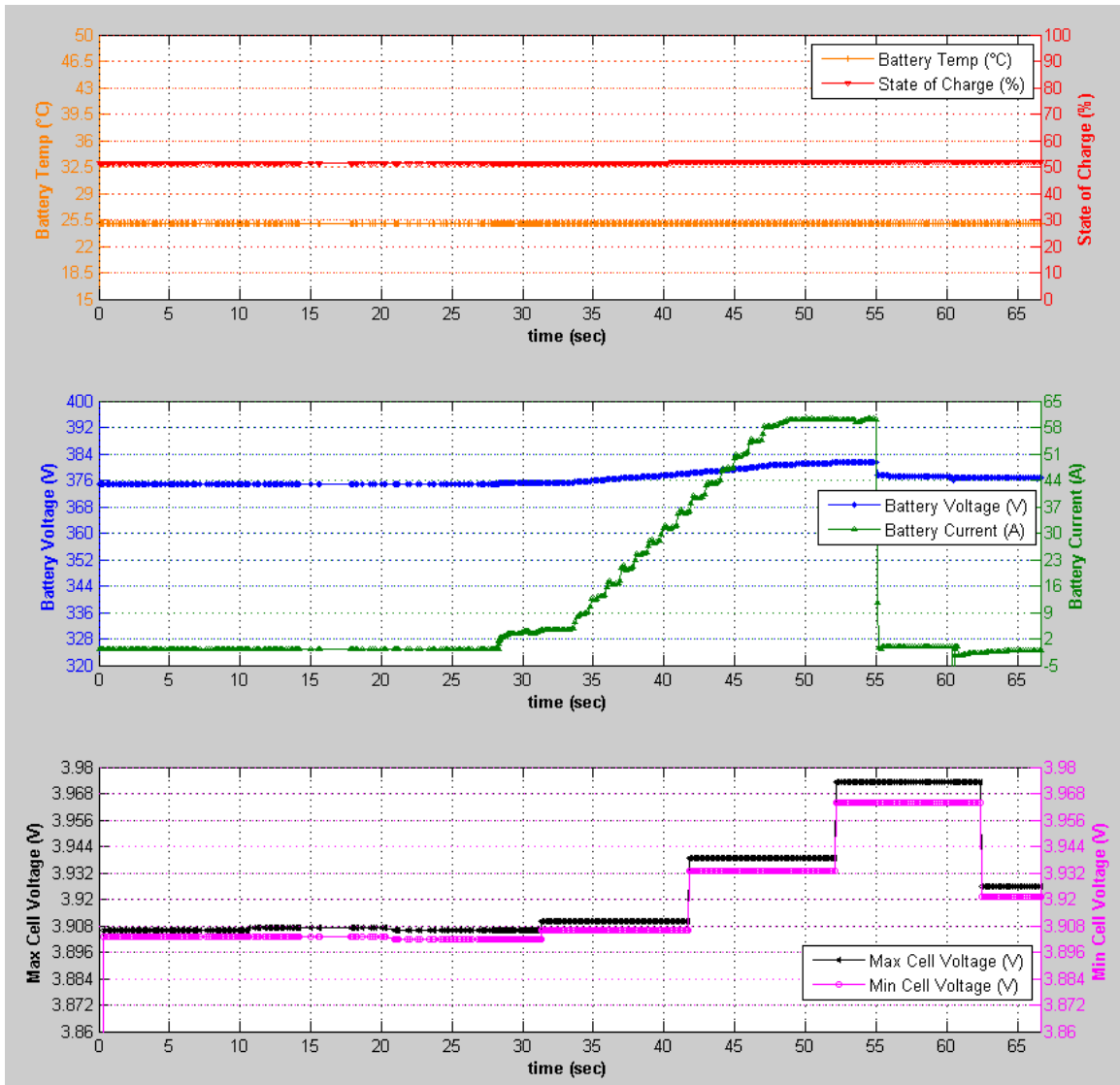
Figure 64: Proximity Open During Charge Session Charge Data
