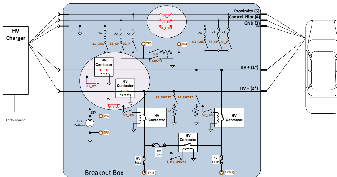
Figure 14: Charge Connector HV Connection Disturbance Test – Initial Breakout Box Configuration
