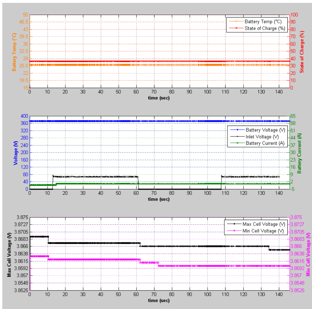
Figure 52: Before Charge Session Charge Data (65V applied to HV bus)
