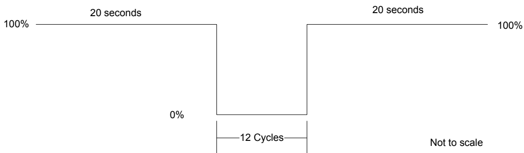
Figure 23: Momentary Outage
